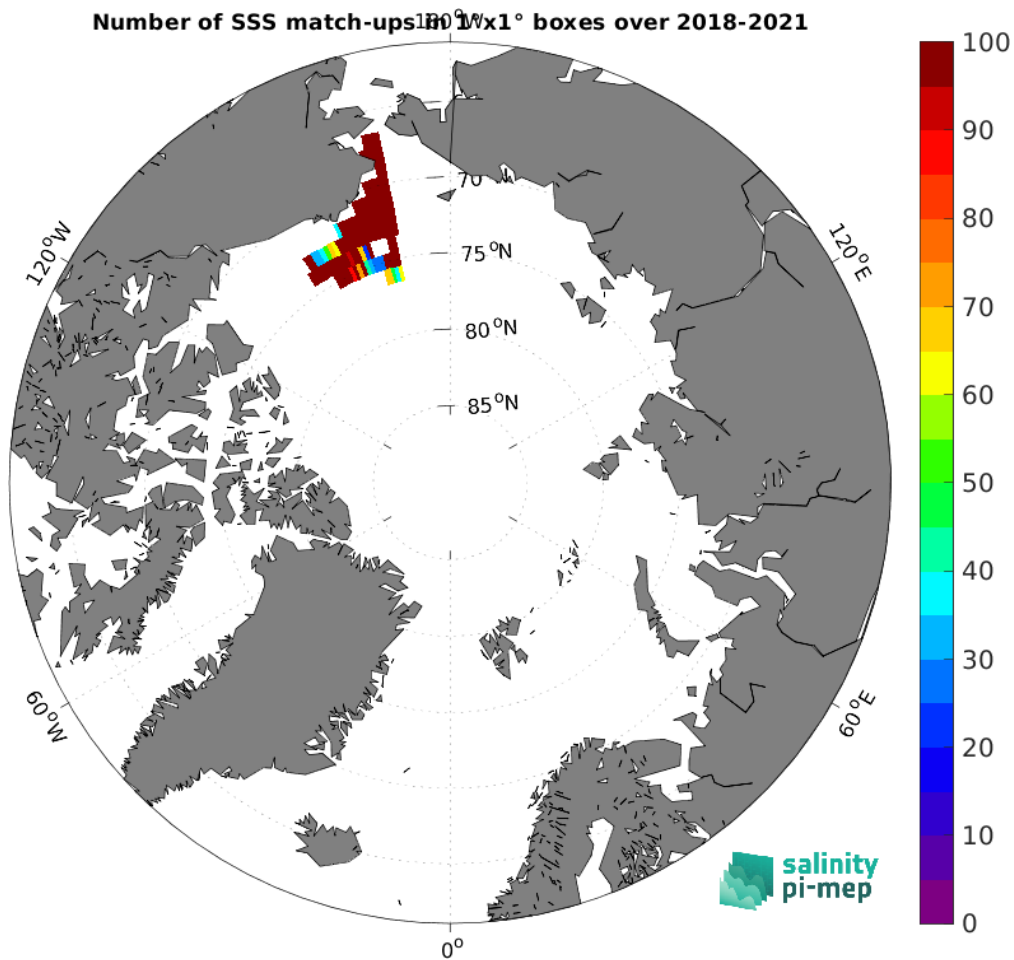
Figure 5: Number of SSS match-ups between Saildrone SSS and the SMAP SSS L3 v6 - Monthly (RSS) SSS product for the Arctic Ocean Pi-MEP region over 1^\circ \times 1^\circ boxes and for the full satellite product period.
