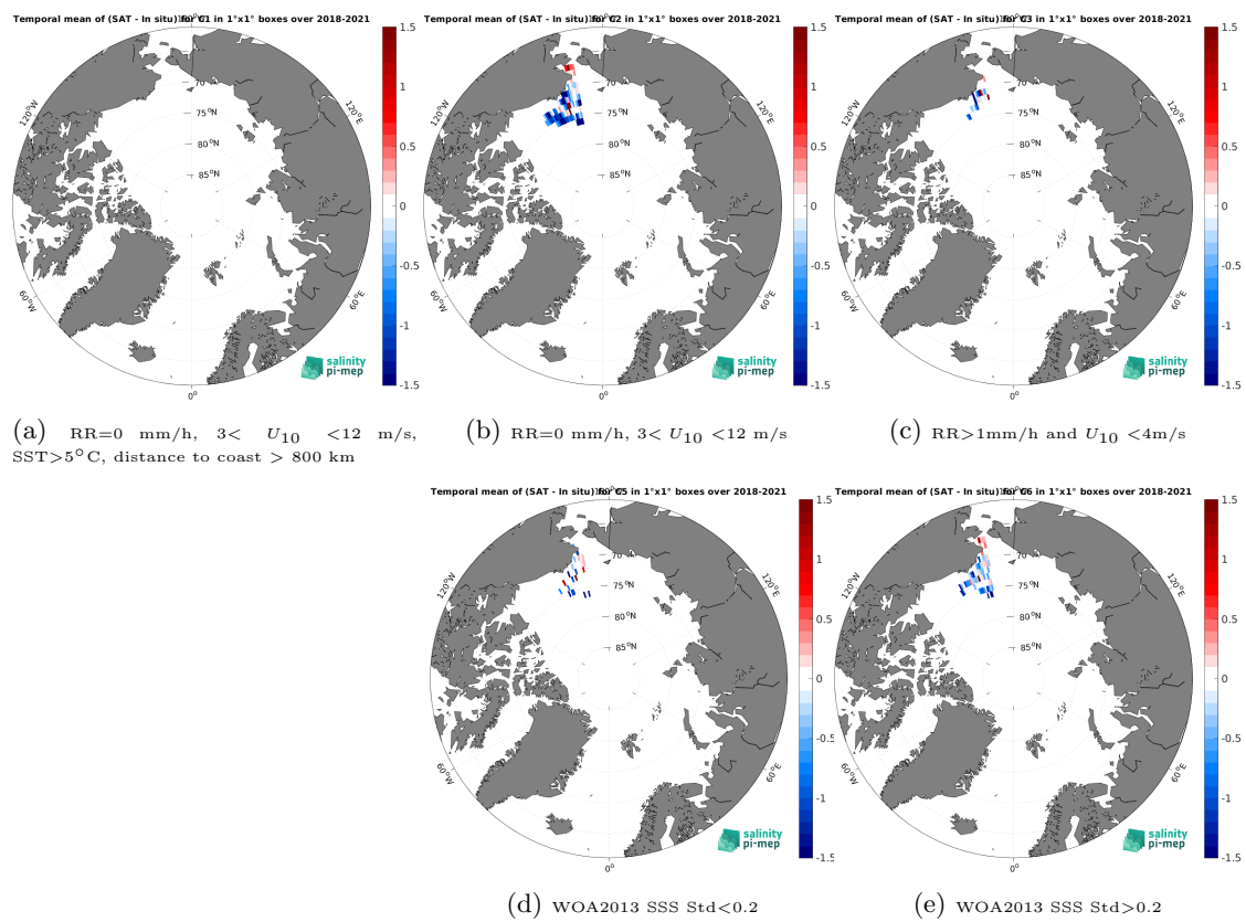
Figure 14: Temporal mean gridded over spatial boxes of size 1^\circ \times 1^\circ of \Delta SSS (SMAP SSS L3 v6 - Monthly (RSS) - Saildrone) for 5 different subdatasets corresponding to:RR=0 mm/h, 3 < U_{10} < 12 m/s, SST > 5^\circ\text{C} , distance to coast > 800 km (a), RR=0 mm/h, 3 < U_{10} < 12 m/s (b), RR > 1 mm/h and U_{10} < 4 m/s (c), WOA2013 SSS Std < 0.2 (d), WOA2013 SSS Std > 0.2 (e).
