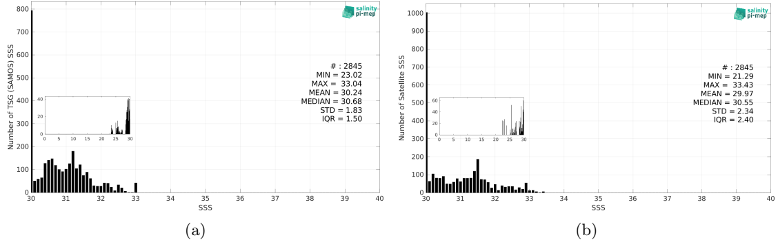
Figure 3: Histograms of SSS from TSG (SAMOS) (a) and SMAP SSS L3 v5.3 - 8-Day running (RSS) (b) considering all match-up pairs per bins of 0.1 over the Arctic Ocean Pi-MEP region and for the full satellite product period.
