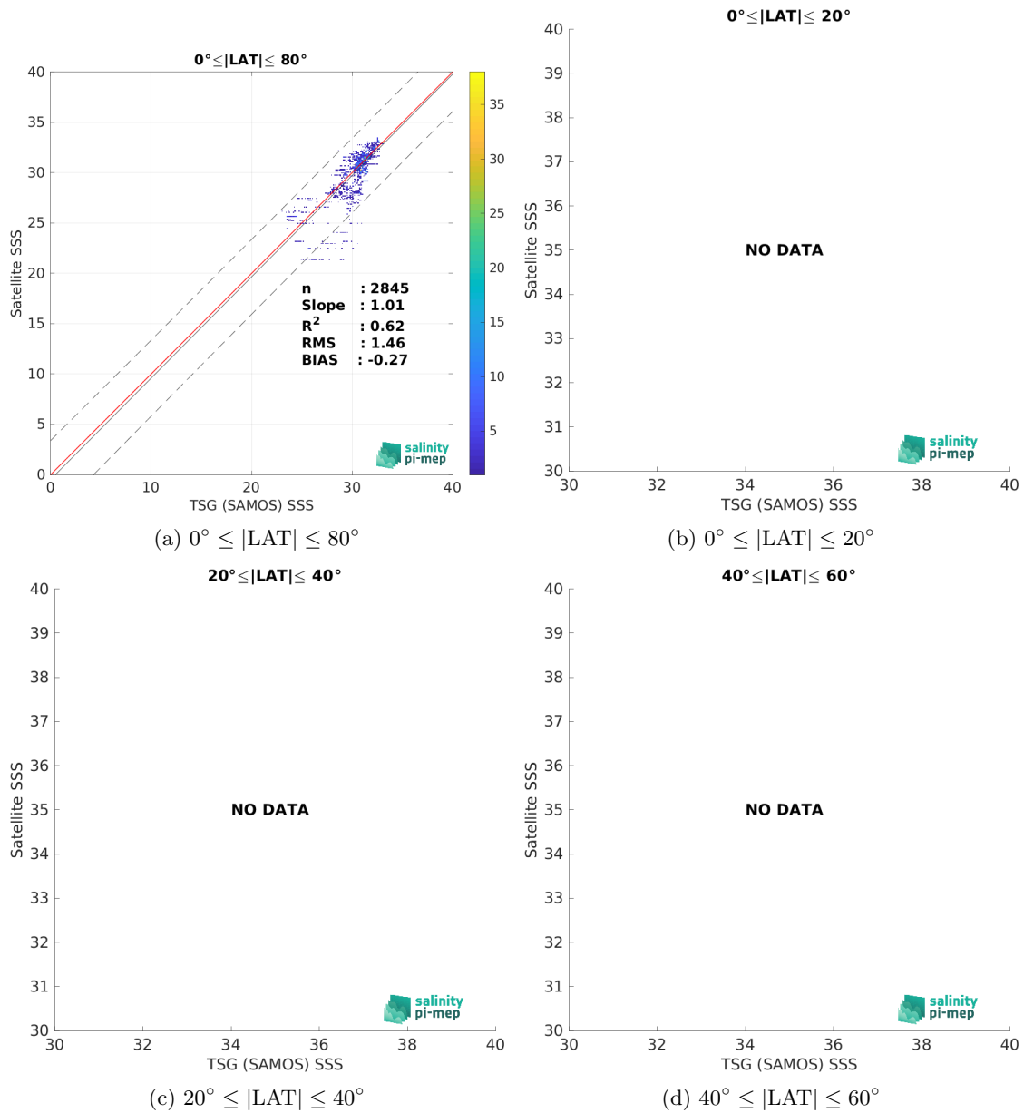
Figure 10: Contour maps of the concentration of SMAP SSS L3 v5.3 - 8-Day running (RSS) SSS (y-axis) versus TSG (SAMOS) SSS (x-axis) at match-up pairs for different latitude bands. For each plot, the red line shows x=y . The black thin and dashed lines indicate a linear fit through the data cloud and the \pm 95\% confidence levels, respectively. The number match-up pairs n , the slope and R^2 coefficient of the linear fit, the root mean square (RMS) and the mean bias between satellite and in situ data are indicated for each latitude band in each plots.
