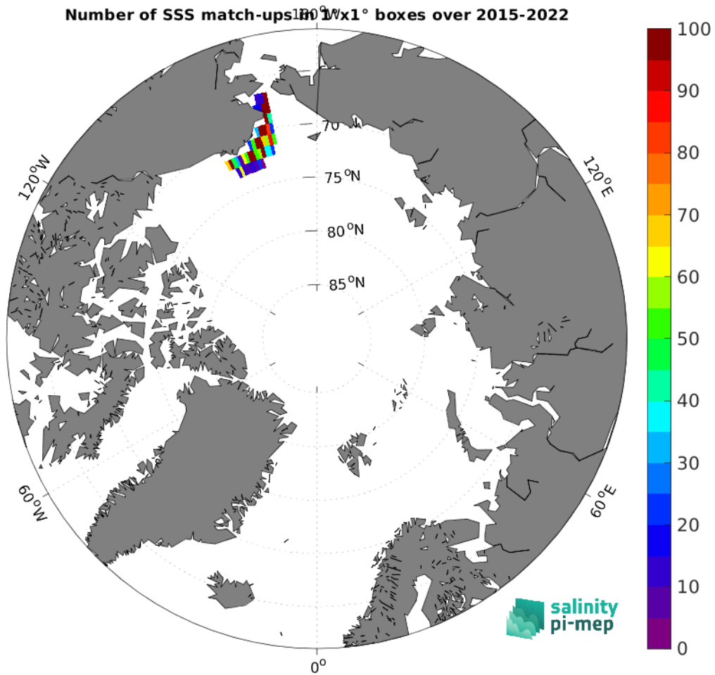
Figure 5: Number of SSS match-ups between TSG (SAMOS) SSS and the SMAP SSS L3 v5.3 - 8-Day running (RSS) SSS product for the Arctic Ocean Pi-MEP region over 1^\circ \times 1^\circ boxes and for the full satellite product period.
