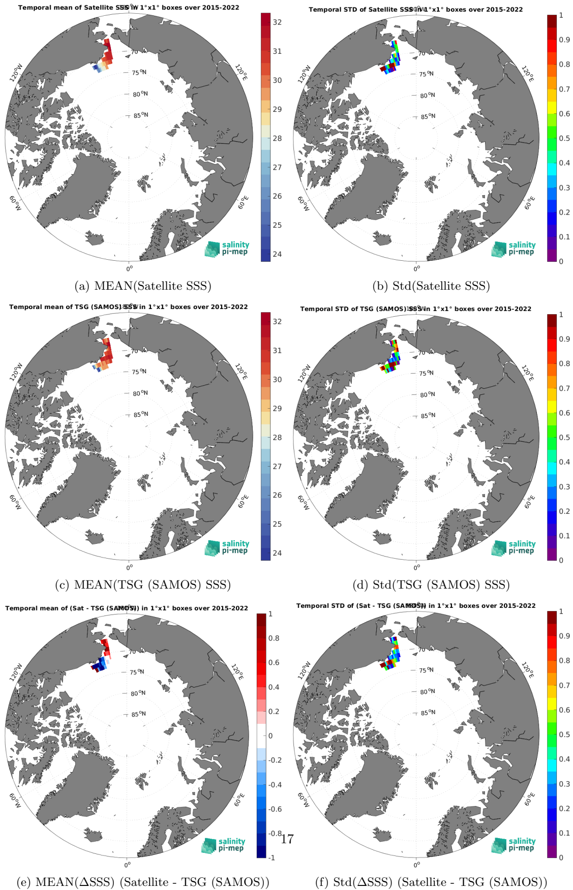
Figure 7: Temporal mean (left) and Std (right) of SSS from SMAP SSS L3 v5.3 - 8-Day running (RSS) (top), TSG (SAMOS) (middle), and of \Delta SSS (Satellite - TSG (SAMOS)). Only match-up pairs are used to generate these maps.
