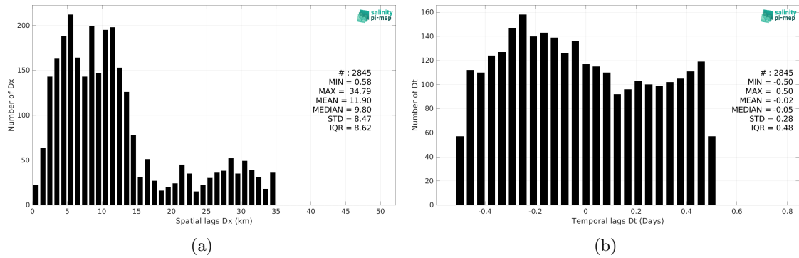
Figure 6: Histograms of the spatial (a) and temporal (b) lags between the location/time of the TSG (SAMOS) measurement and the date of the corresponding SMAP SSS L3 v5.3 - 8-Day running (RSS) SSS pixel.
