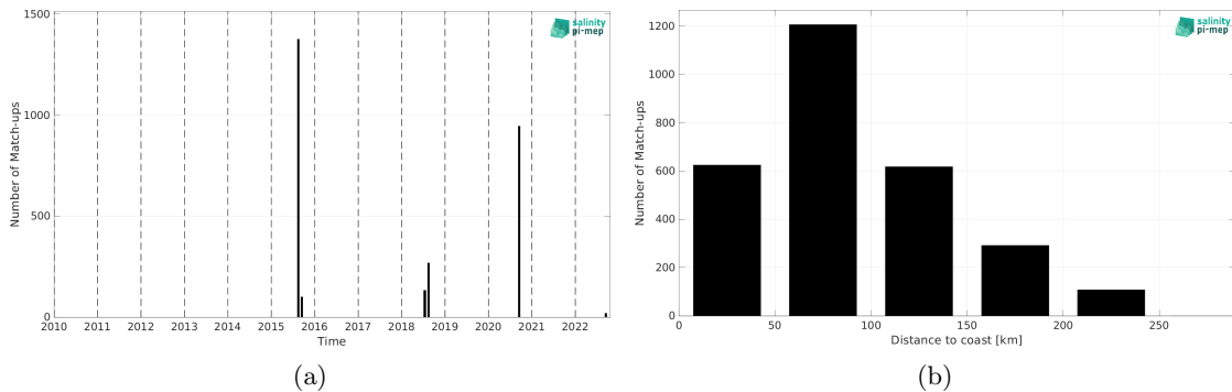
Figure 2: Number of match-ups between TSG (SAMOS) and SMAP SSS L3 v5.3 - 8-Day running (RSS) SSS as a function of time (a) and as function of the distance to coast (b) over the Arctic Ocean Pi-MEP region and for the full satellite product period.
