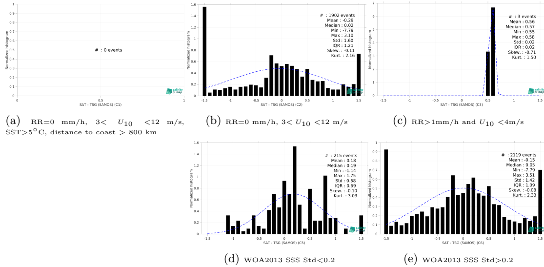
Figure 15: Normalized histogram of \Delta SSS (SMAP SSS L3 v5.3 - 8-Day running (RSS) - TSG (SAMOS)) for 5 different subdatasets corresponding to: RR=0 mm/h, 3 < U_{10} < 12 m/s, SST>5°C, distance to coast > 800 km (a), RR=0 mm/h, 3 < U_{10} < 12 m/s (b), RR>1mm/h and U_{10} < 4 m/s (c), WOA2013 SSS Std<0.2 (d), WOA2013 SSS Std>0.2 (e).
