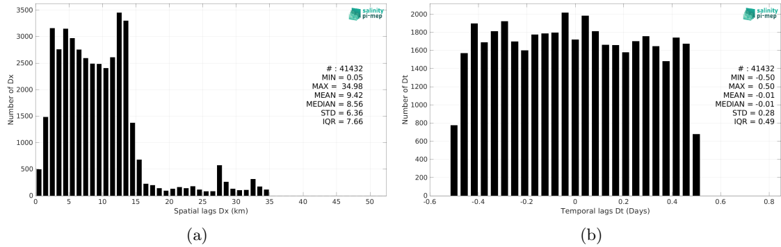
Figure 6: Histograms of the spatial (a) and temporal (b) lags between the location/time of the TSG (Polarstern) measurement and the date of the corresponding SMAP SSS L3 v5.3 - 8-Day running (RSS) SSS pixel.
