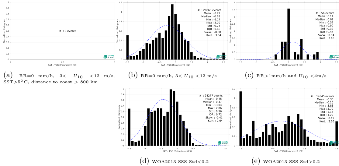
Figure 15: Normalized histogram of \Delta SSS (SMAP SSS L3 v5.3 - 8-Day running (RSS) - TSG (Polarstern)) for 5 different subdatasets corresponding to: RR=0 mm/h, 3 < U_{10} < 12 m/s, SST>5°C, distance to coast > 800 km (a), RR=0 mm/h, 3 < U_{10} < 12 m/s (b), RR>1mm/h and U_{10} < 4 m/s (c), WOA2013 SSS Std<0.2 (d), WOA2013 SSS Std>0.2 (e).
