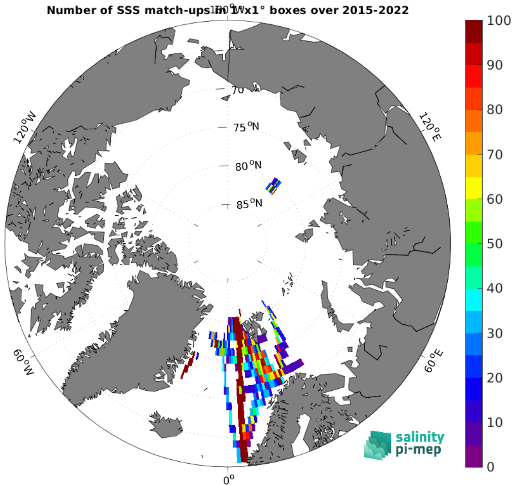
Figure 5: Number of SSS match-ups between TSG (Polarstern) SSS and the SMAP SSS L3 v5.3 - 8-Day running (RSS) SSS product for the Arctic Ocean Pi-MEP region over 1^\circ \times 1^\circ boxes and for the full satellite product period.
