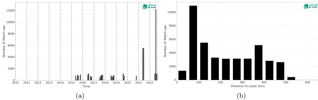
Figure 2: Number of match-ups between TSG (Polarstern) and SMAP SSS L3 v5.3 - 8-Day running (RSS) SSS as a function of time (a) and as function of the distance to coast (b) over the Arctic Ocean Pi-MEP region and for the full satellite product period.
