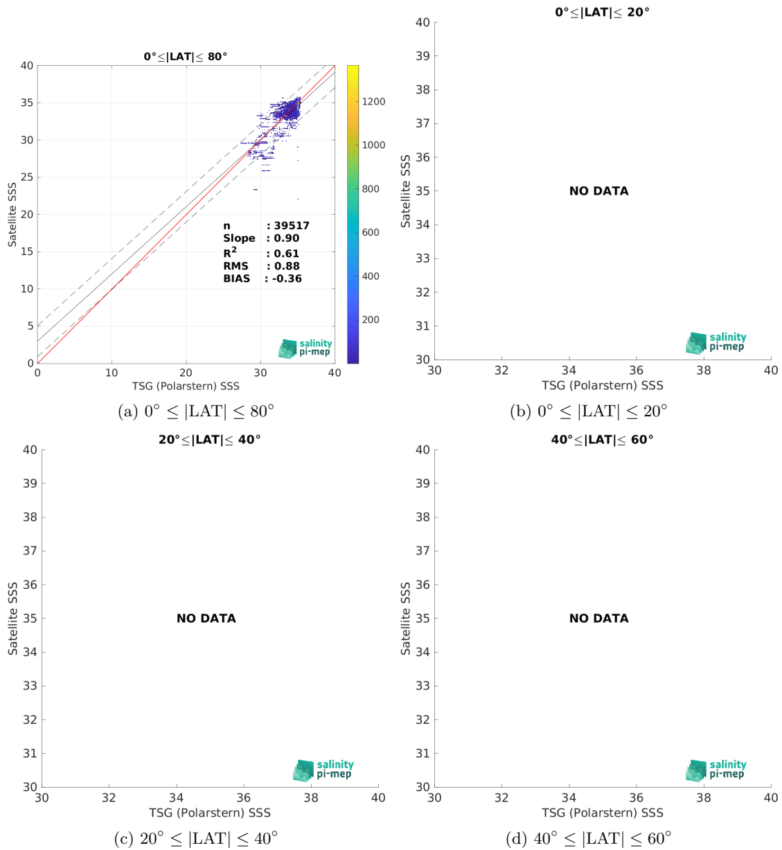
Figure 10: Contour maps of the concentration of SMAP SSS L3 v5.3 - 8-Day running (RSS) SSS (y-axis) versus TSG (Polarstern) SSS (x-axis) at match-up pairs for different latitude bands. For each plot, the red line shows x=y . The black thin and dashed lines indicate a linear fit through the data cloud and the \pm 95\% confidence levels, respectively. The number match-up pairs n , the slope and R^2 coefficient of the linear fit, the root mean square (RMS) and the mean bias between satellite and in situ data are indicated for each latitude band in each plots.
