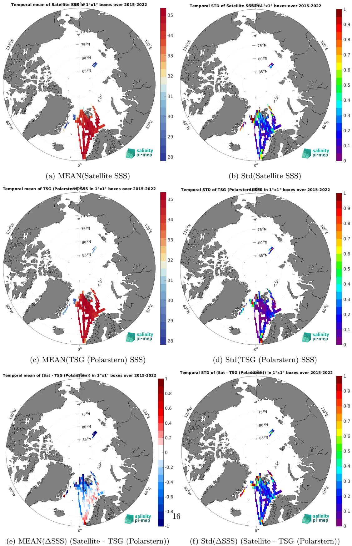
Figure 7: Temporal mean (left) and Std (right) of SSS from SMAP SSS L3 v5.3 - 8-Day running (RSS) (top), TSG (Polarstern) (middle), and of \Delta SSS (Satellite - TSG (Polarstern)). Only match-up pairs are used to generate these maps.
