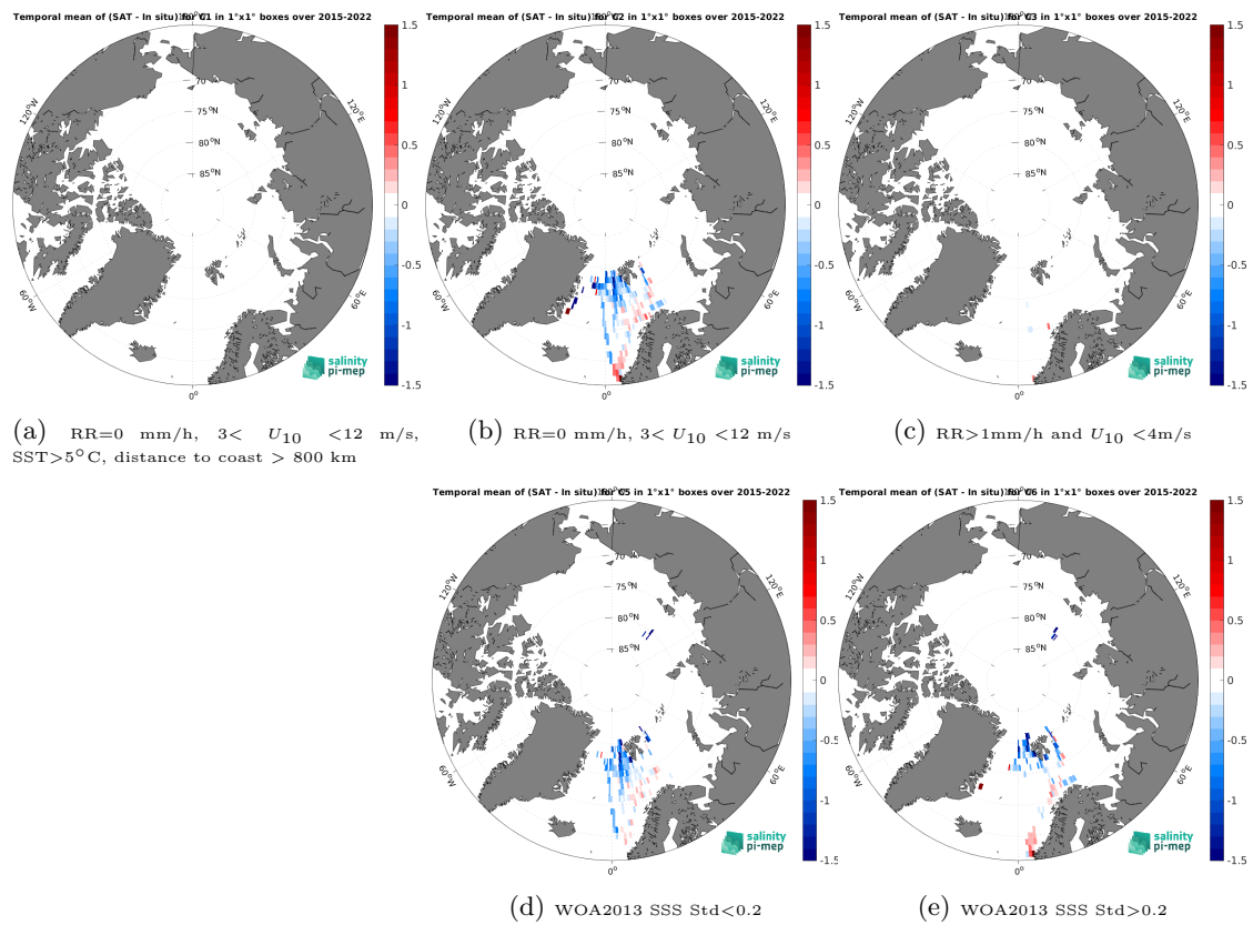
Figure 14: Temporal mean gridded over spatial boxes of size 1^\circ \times 1^\circ of \Delta\text{SSS} (SMAP SSS L3 v5.3 - 8-Day running (RSS) - TSG (Polarstern)) for 5 different subdatasets corresponding to:RR=0 mm/h, 3 < U_{10} < 12 m/s, SST > 5°C, distance to coast > 800 km (a), RR=0 mm/h, 3 < U_{10} < 12 m/s (b), RR > 1mm/h and U_{10} < 4 m/s (c), WOA2013 SSS Std < 0.2 (d), WOA2013 SSS Std > 0.2 (e).
