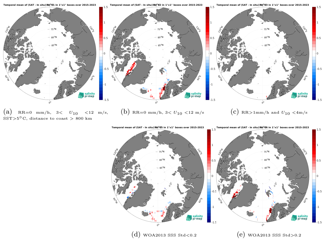
Figure 14: Temporal mean gridded over spatial boxes of size 1^\circ \times 1^\circ of \Delta SSS (SMAP SSS L3 v5.3 - 8-Day running (RSS) - TSG (LEGOS-DM)) for 5 different subdatasets corresponding to:RR=0 mm/h, 3 < U_{10} < 12 m/s, SST > 5^\circ\text{C} , distance to coast > 800 km (a), RR=0 mm/h, 3 < U_{10} < 12 m/s (b), RR > 1 mm/h and U_{10} < 4 m/s (c), WOA2013 SSS Std < 0.2 (d), WOA2013 SSS Std > 0.2 (e).
