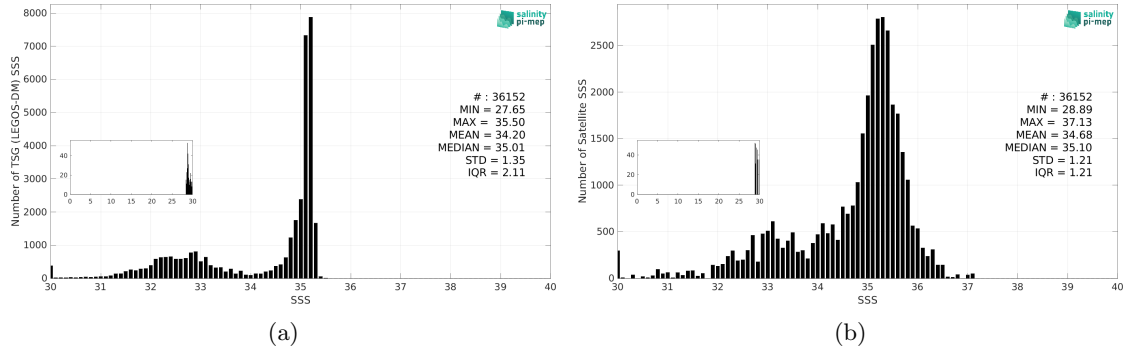
Figure 3: Histograms of SSS from TSG (LEGOS-DM) (a) and SMAP SSS L3 v5.3 - 8-Day running (RSS) (b) considering all match-up pairs per bins of 0.1 over the Arctic Ocean Pi-MEP region and for the full satellite product period.
