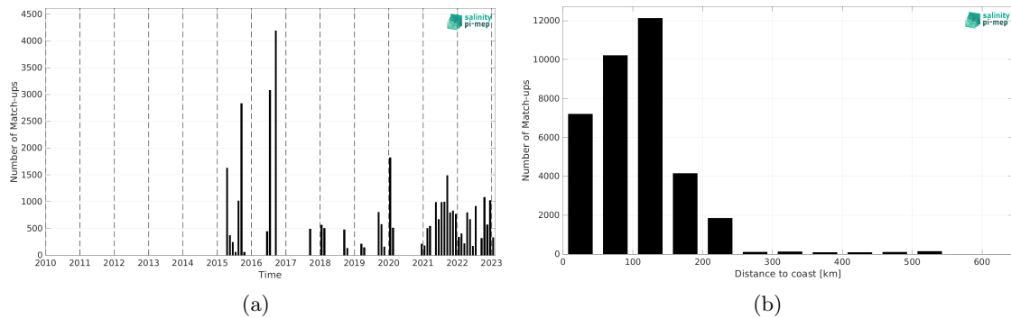
Figure 2: Number of match-ups between TSG (LEGOS-DM) and SMAP SSS L3 v5.3 - 8-Day running (RSS) SSS as a function of time (a) and as function of the distance to coast (b) over the Arctic Ocean Pi-MEP region and for the full satellite product period.
