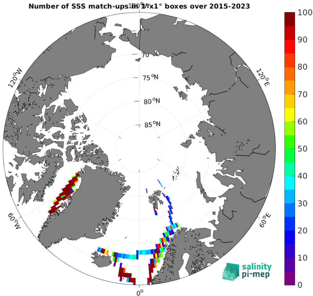
Figure 5: Number of SSS match-ups between TSG (LEGOS-DM) SSS and the SMAP SSS L3 v5.3 - 8-Day running (RSS) SSS product for the Arctic Ocean Pi-MEP region over 1^\circ \times 1^\circ boxes and for the full satellite product period.
