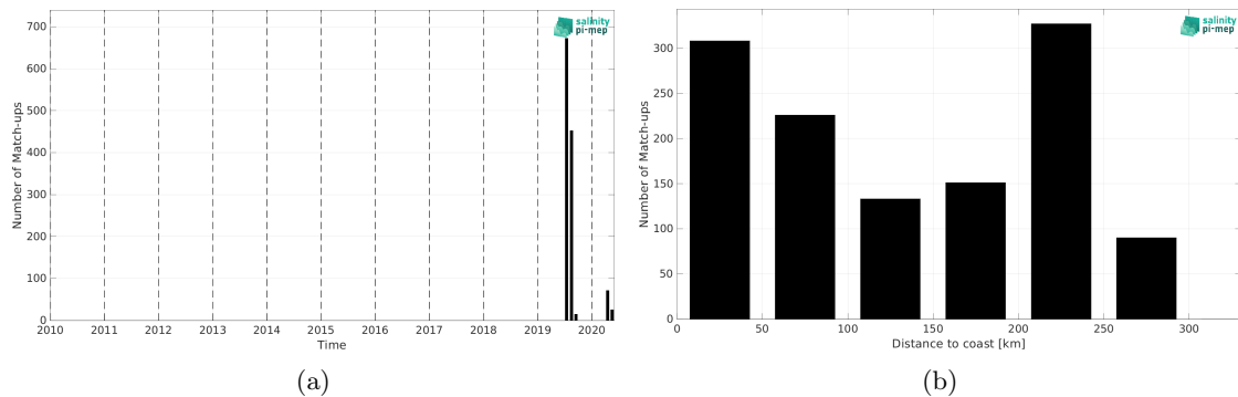
Figure 2: Number of match-ups between TSG (Lauge-Koch) and SMAP SSS L3 v5.3 - 8-Day running (RSS) SSS as a function of time (a) and as function of the distance to coast (b) over the Arctic Ocean Pi-MEP region and for the full satellite product period.
