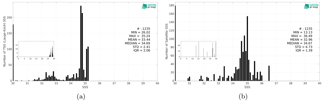
Figure 3: Histograms of SSS from TSG (Lauge-Koch) (a) and SMAP SSS L3 v5.3 - 8-Day running (RSS) (b) considering all match-up pairs per bins of 0.1 over the Arctic Ocean Pi-MEP region and for the full satellite product period.
