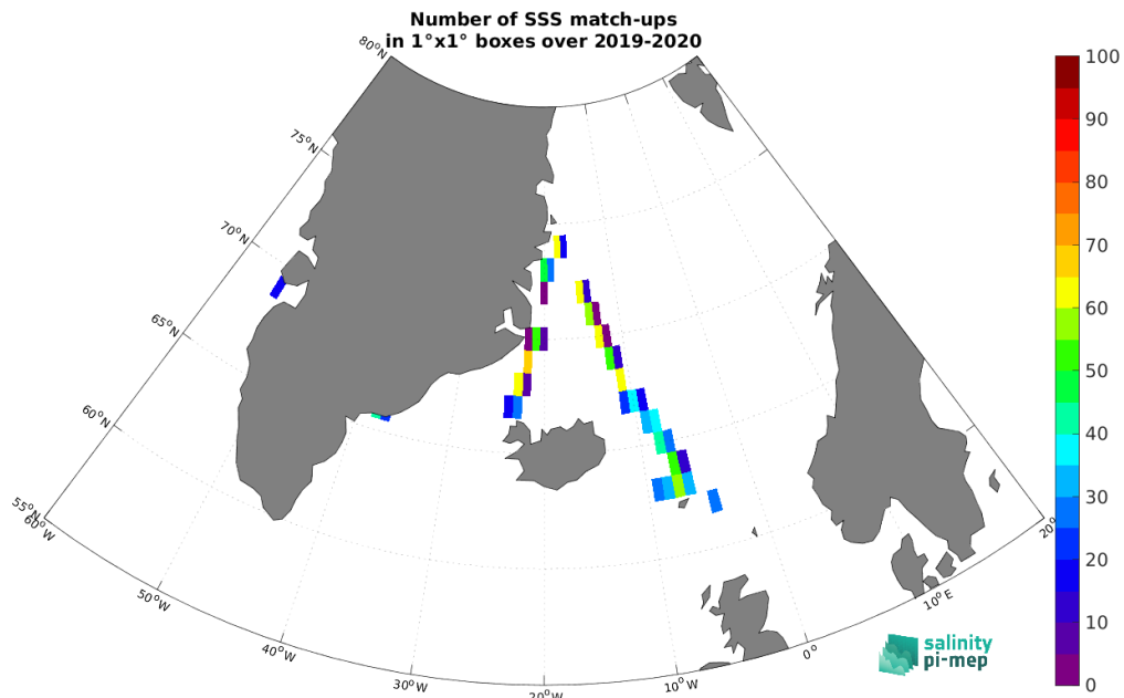
Figure 5: Number of SSS match-ups between TSG (Lauge-Koch) SSS and the SMAP SSS L3 v5.3 - 8-Day running (RSS) SSS product for the Arctic Ocean Pi-MEP region over 1^\circ \times 1^\circ boxes and for the full satellite product period.
