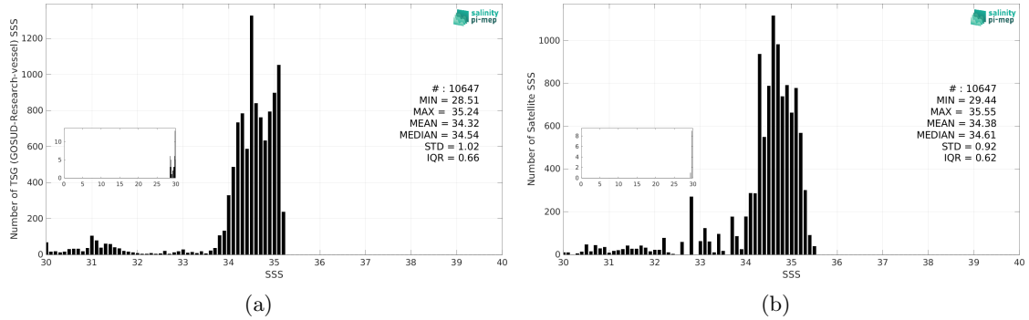
Figure 3: Histograms of SSS from TSG (GOSUD-Research-vessel) (a) and SMAP SSS L3 v5.3 - 8-Day running (RSS) (b) considering all match-up pairs per bins of 0.1 over the Arctic Ocean Pi-MEP region and for the full satellite product period.
