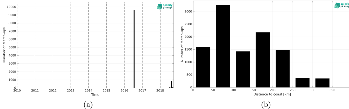
Figure 2: Number of match-ups between TSG (GOSUD-Research-vessel) and SMAP SSS L3 v5.3 - 8-Day running (RSS) SSS as a function of time (a) and as function of the distance to coast (b) over the Arctic Ocean Pi-MEP region and for the full satellite product period.
