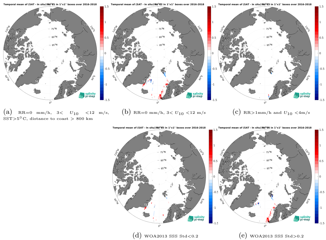
Figure 14: Temporal mean gridded over spatial boxes of size 1^\circ \times 1^\circ of \Delta\text{SSS} (SMAP SSS L3 v5.3 - 8-Day running (RSS) - TSG (GOSUD-Research-vessel)) for 5 different subdatasets corresponding to:RR=0 mm/h, 3 < U_{10} < 12 m/s, SST>5°C, distance to coast > 800 km (a), RR=0 mm/h, 3 < U_{10} < 12 m/s (b), RR>1mm/h and U_{10} < 4 m/s (c), WOA2013 SSS Std<0.2 (d), WOA2013 SSS Std>0.2 (e).
