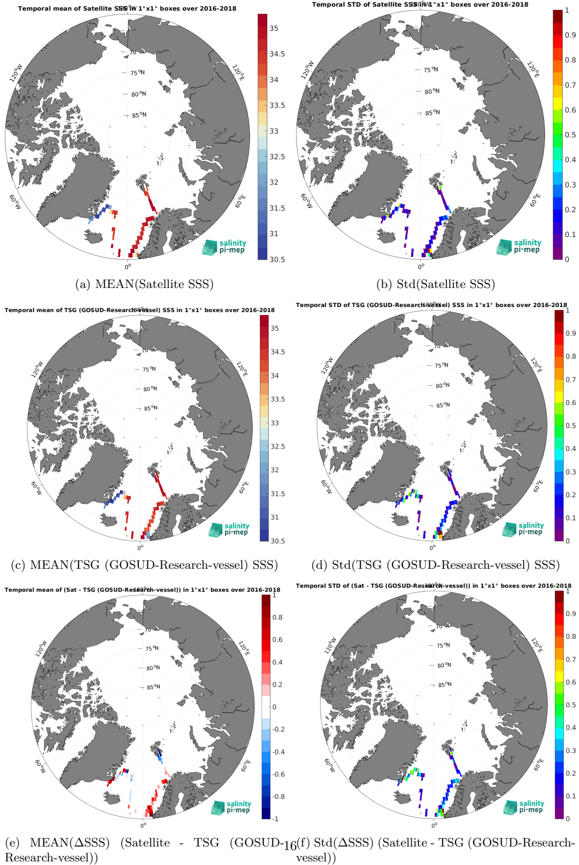
Figure 7: Temporal mean (left) and Std (right) of SSS from SMAP SSS L3 v5.3 - 8-Day running (RSS) (top), TSG (GOSUD-Research-vessel) (middle), and of \Delta SSS (Satellite - TSG (GOSUD-Research-vessel)). Only match-up pairs are used to generate these maps.
