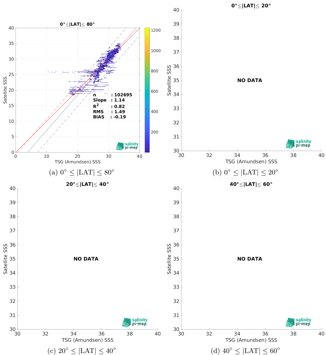
Figure 10: Contour maps of the concentration of SMAP SSS L3 v5.3 - 8-Day running (RSS) SSS (y-axis) versus TSG (Amundsen) SSS (x-axis) at match-up pairs for different latitude bands. For each plot, the red line shows x=y . The black thin and dashed lines indicate a linear fit through the data cloud and the \pm 95\% confidence levels, respectively. The number match-up pairs n , the slope and R^2 coefficient of the linear fit, the root mean square (RMS) and the mean bias between satellite and in situ data are indicated for each latitude band in each plots.
