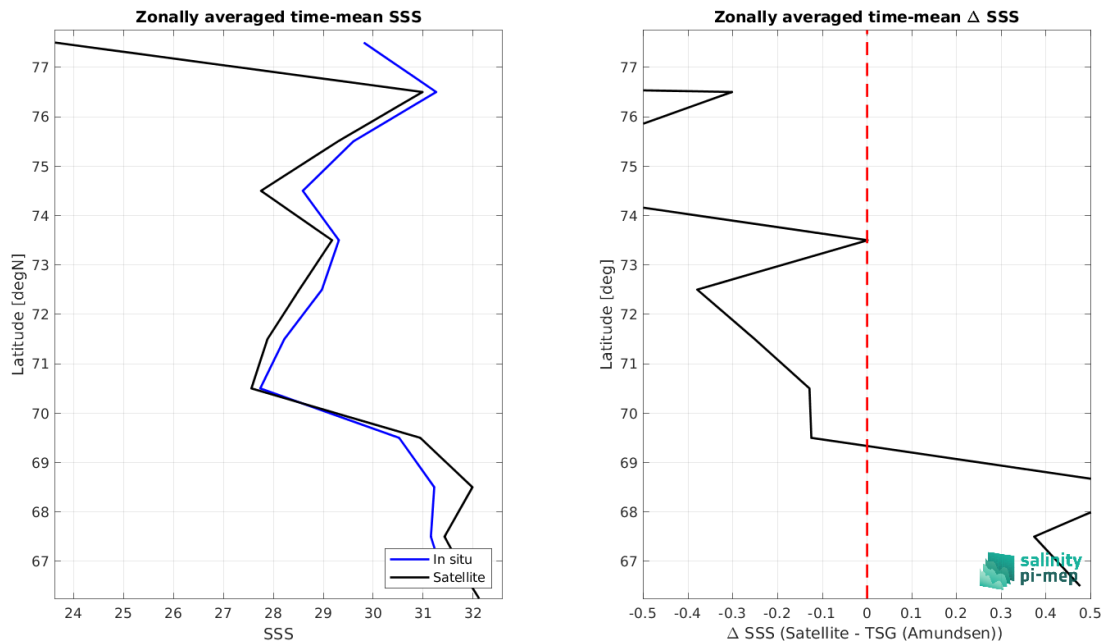
Figure 9: Left panel: Zonal mean SSS from SMAP SSS L3 v5.3 - 8-Day running (RSS) satellite product (black) and from TSG (Amundsen) (blue). Right panel: Zonal mean of \Delta SSS (Satellite - TSG (Amundsen)) for all the collected Pi-MEP match-up pairs estimated over the full satellite product period.
