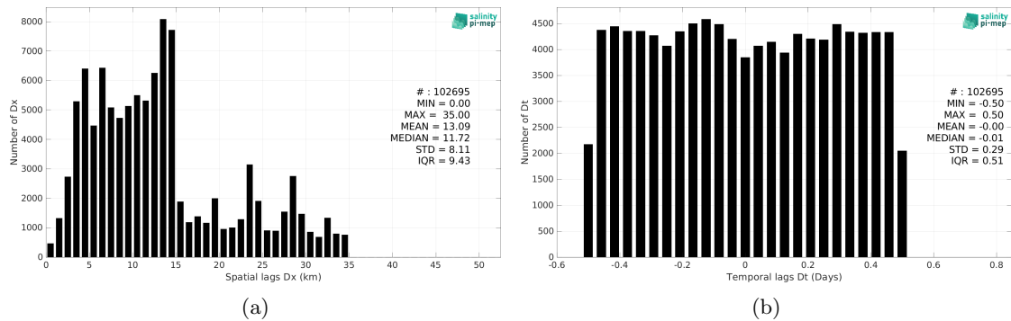
Figure 6: Histograms of the spatial (a) and temporal (b) lags between the location/time of the TSG (Amundsen) measurement and the date of the corresponding SMAP SSS L3 v5.3 - 8-Day running (RSS) SSS pixel.
