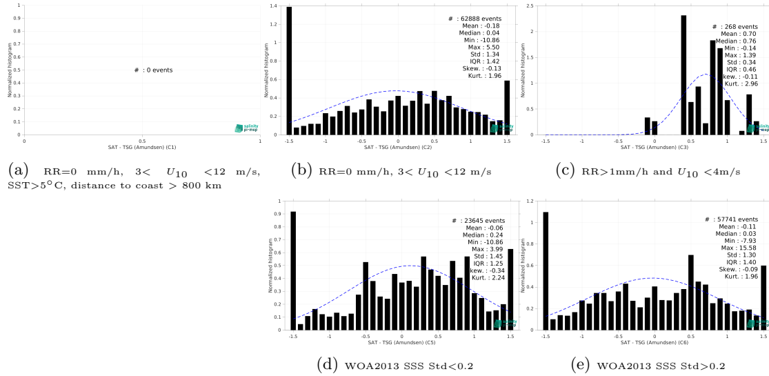
Figure 15: Normalized histogram of \Delta SSS (SMAP SSS L3 v5.3 - 8-Day running (RSS) - TSG (Amundsen)) for 5 different subdatasets corresponding to: RR=0 mm/h, 3 < U_{10} < 12 m/s, SST>5°C, distance to coast > 800 km (a), RR=0 mm/h, 3 < U_{10} < 12 m/s (b), RR>1mm/h and U_{10} < 4 m/s (c), WOA2013 SSS Std<0.2 (d), WOA2013 SSS Std>0.2 (e).
