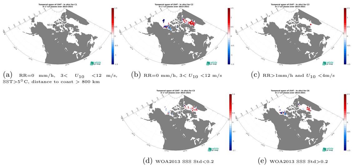
Figure 14: Temporal mean gridded over spatial boxes of size 1^\circ \times 1^\circ of \Delta SSS (SMAP SSS L3 v5.3 - 8-Day running (RSS) - TSG (Amundsen)) for 5 different subdatasets corresponding to:RR=0 mm/h, 3 < U_{10} < 12 m/s, SST > 5°C, distance to coast > 800 km (a), RR=0 mm/h, 3 < U_{10} < 12 m/s (b), RR > 1mm/h and U_{10} < 4 m/s (c), WOA2013 SSS Std < 0.2 (d), WOA2013 SSS Std > 0.2 (e).
