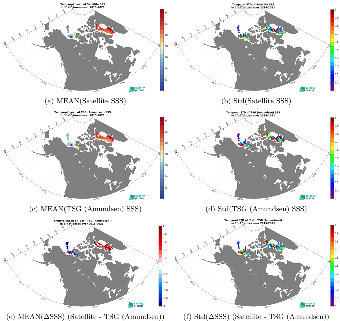
Figure 7: Temporal mean (left) and Std (right) of SSS from SMAP SSS L3 v5.3 - 8-Day running (RSS) (top), TSG (Amundsen) (middle), and of \Delta SSS (Satellite - TSG (Amundsen)). Only match-up pairs are used to generate these maps.
