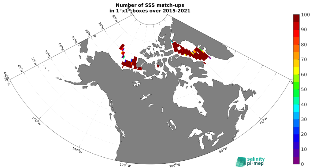
Figure 5: Number of SSS match-ups between TSG (Amundsen) SSS and the SMAP SSS L3 v5.3 - 8-Day running (RSS) SSS product for the Arctic Ocean Pi-MEP region over 1^\circ \times 1^\circ boxes and for the full satellite product period.
