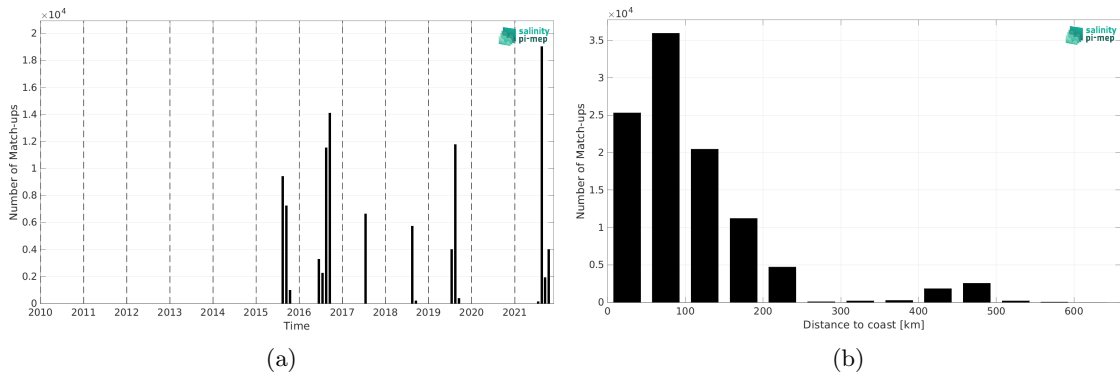
Figure 2: Number of match-ups between TSG (Amundsen) and SMAP SSS L3 v5.3 - 8-Day running (RSS) SSS as a function of time (a) and as function of the distance to coast (b) over the Arctic Ocean Pi-MEP region and for the full satellite product period.
