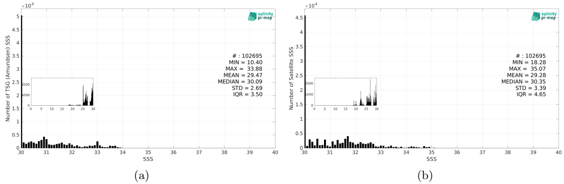
Figure 3: Histograms of SSS from TSG (Amundsen) (a) and SMAP SSS L3 v5.3 - 8-Day running (RSS) (b) considering all match-up pairs per bins of 0.1 over the Arctic Ocean Pi-MEP region and for the full satellite product period.
