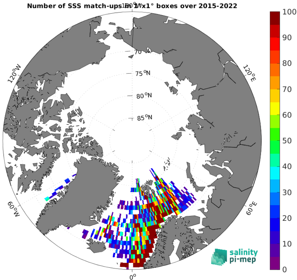
Figure 5: Number of SSS match-ups between ICES SSS and the SMAP SSS L3 v5.3 - 8-Day running (RSS) SSS product for the Arctic Ocean Pi-MEP region over 1^\circ \times 1^\circ boxes and for the full satellite product period.
