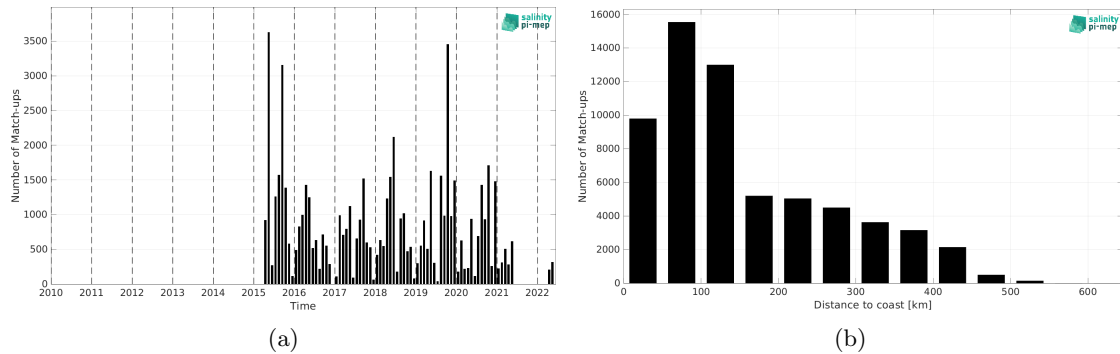
Figure 2: Number of match-ups between ICES and SMAP SSS L3 v5.3 - 8-Day running (RSS) SSS as a function of time (a) and as function of the distance to coast (b) over the Arctic Ocean Pi-MEP region and for the full satellite product period.
