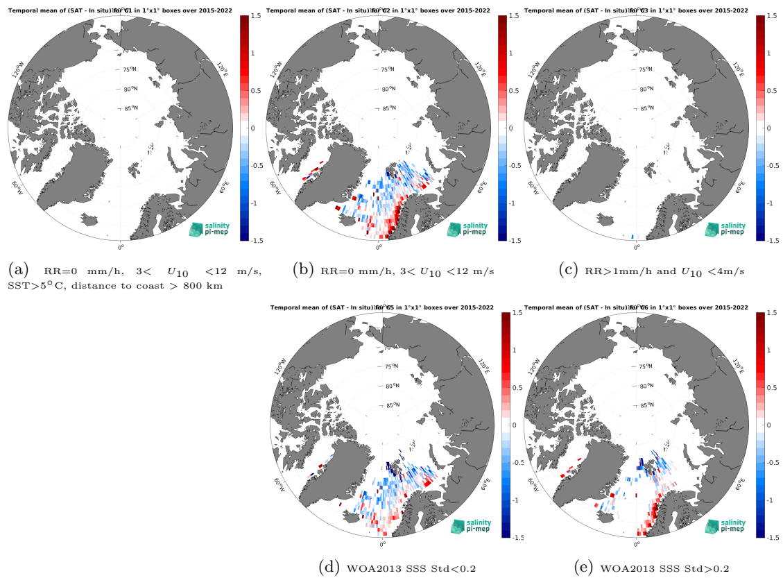
Figure 14: Temporal mean gridded over spatial boxes of size 1^\circ \times 1^\circ of \Delta SSS (SMAP SSS L3 v5.3 - 8-Day running (RSS) - ICES) for 5 different subdatasets corresponding to: RR=0 mm/h, 3 < U_{10} < 12 m/s, SST > 5°C, distance to coast > 800 km (a), RR=0 mm/h, 3 < U_{10} < 12 m/s (b), RR > 1mm/h and U_{10} < 4 m/s (c), WOA2013 SSS Std < 0.2 (d), WOA2013 SSS Std > 0.2 (e).
