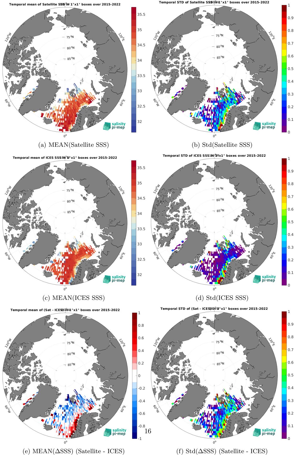
Figure 7: Temporal mean (left) and Std (right) of SSS from SMAP SSS L3 v5.3 - 8-Day running (RSS) (top), ICES (middle), and of \Delta SSS (Satellite - ICES). Only match-up pairs are used to generate these maps.
