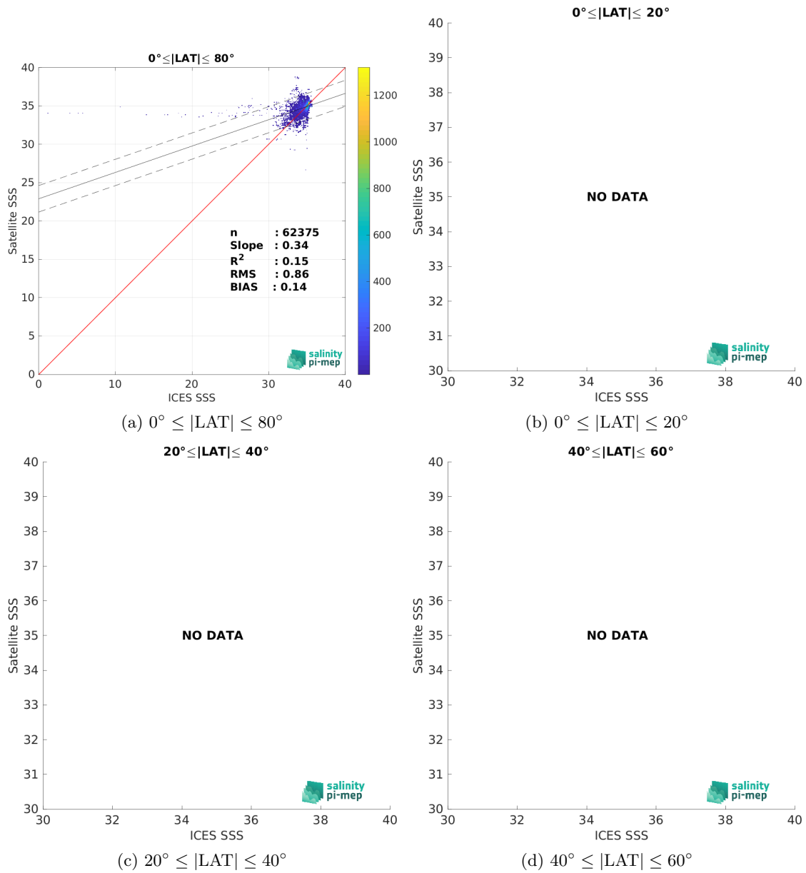
Figure 10: Contour maps of the concentration of SMAP SSS L3 v5.3 - 8-Day running (RSS) SSS (y-axis) versus ICES SSS (x-axis) at match-up pairs for different latitude bands. For each plot, the red line shows x=y . The black thin and dashed lines indicate a linear fit through the data cloud and the \pm 95\% confidence levels, respectively. The number match-up pairs n , the slope and R^2 coefficient of the linear fit, the root mean square (RMS) and the mean bias between satellite and in situ data are indicated for each latitude band in each plots.
