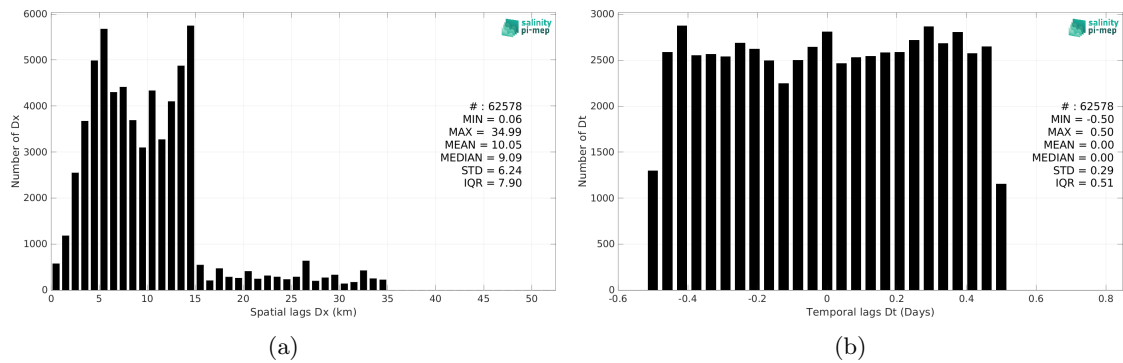
Figure 6: Histograms of the spatial (a) and temporal (b) lags between the location/time of the ICES measurement and the date of the corresponding SMAP SSS L3 v5.3 - 8-Day running (RSS) SSS pixel.
