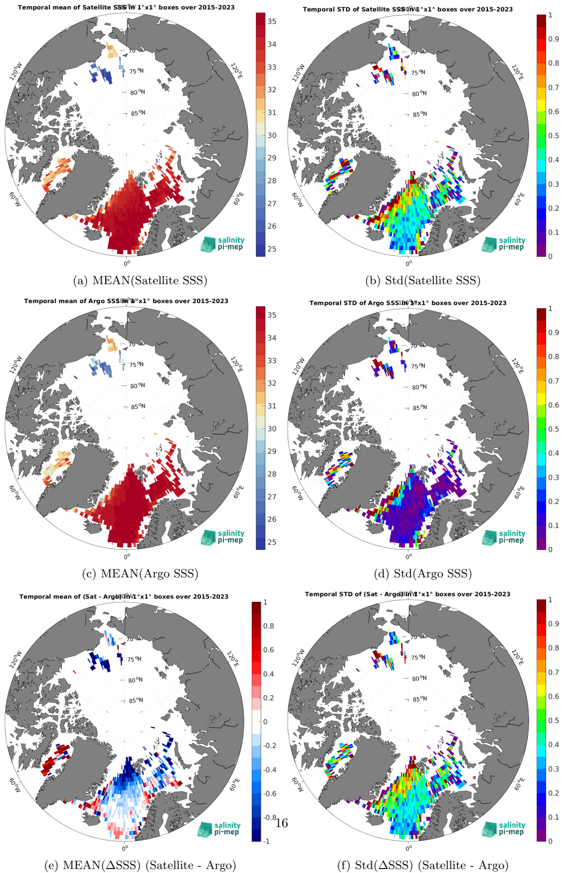
Figure 7: Temporal mean (left) and Std (right) of SSS from SMAP SSS L3 v5.3 - 8-Day running (RSS) (top), Argo (middle), and of \Delta SSS (Satellite - Argo). Only match-up pairs are used to generate these maps.
