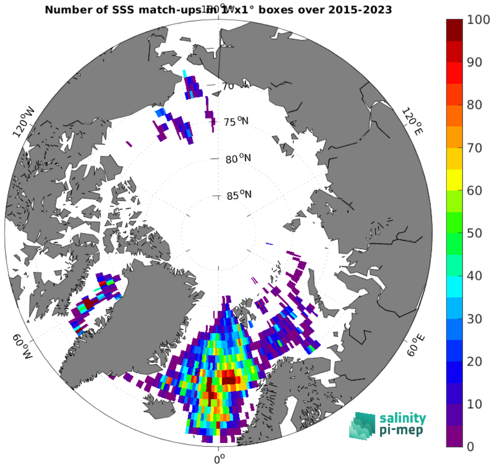
Figure 5: Number of SSS match-ups between Argo SSS and the SMAP SSS L3 v5.3 - 8-Day running (RSS) SSS product for the Arctic Ocean Pi-MEP region over 1^\circ \times 1^\circ boxes and for the full satellite product period.
