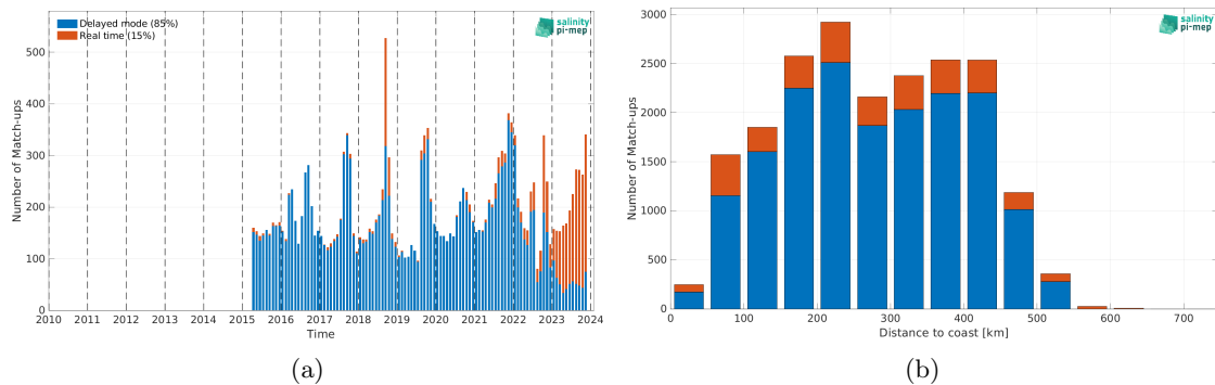
Figure 2: Number of match-ups between Argo and SMAP SSS L3 v5.3 - 8-Day running (RSS) SSS as a function of time (a) and as function of the distance to coast (b) over the Arctic Ocean Pi-MEP region and for the full satellite product period.
