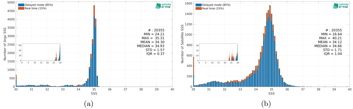
Figure 3: Histograms of SSS from Argo (a) and SMAP SSS L3 v5.3 - 8-Day running (RSS) (b) considering all match-up pairs per bins of 0.1 over the Arctic Ocean Pi-MEP region and for the full satellite product period.
