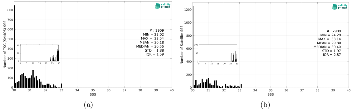
Figure 3: Histograms of SSS from TSG (SAMOS) (a) and SMAP SSS L3 v5.3 - Monthly (RSS) (b) considering all match-up pairs per bins of 0.1 over the Arctic Ocean Pi-MEP region and for the full satellite product period.
