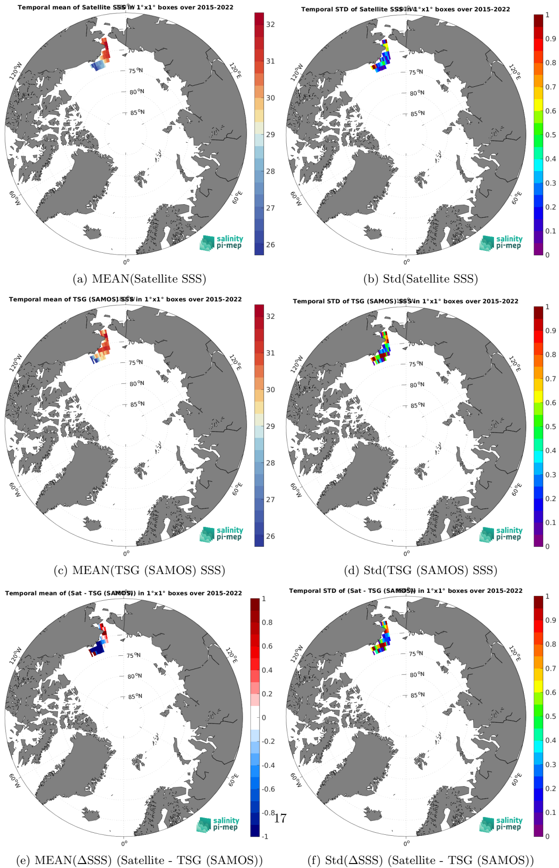
Figure 7: Temporal mean (left) and Std (right) of SSS from SMAP SSS L3 v5.3 - Monthly (RSS) (top), TSG (SAMOS) (middle), and of \Delta SSS (Satellite - TSG (SAMOS)). Only match-up pairs are used to generate these maps.
