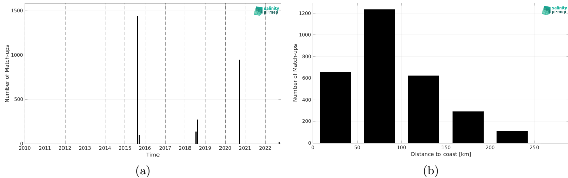
Figure 2: Number of match-ups between TSG (SAMOS) and SMAP SSS L3 v5.3 - Monthly (RSS) SSS as a function of time (a) and as function of the distance to coast (b) over the Arctic Ocean Pi-MEP region and for the full satellite product period.
