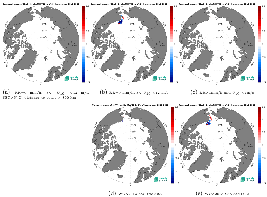
Figure 14: Temporal mean gridded over spatial boxes of size 1^\circ \times 1^\circ of \Delta SSS (SMAP SSS L3 v5.3 - Monthly (RSS) - TSG (SAMOS)) for 5 different subdatasets corresponding to:RR=0 mm/h, 3 < U_{10} < 12 m/s, SST>5°C, distance to coast > 800 km (a), RR=0 mm/h, 3 < U_{10} < 12 m/s (b), RR>1mm/h and U_{10} < 4 m/s (c), WOA2013 SSS Std<0.2 (d), WOA2013 SSS Std>0.2 (e).
