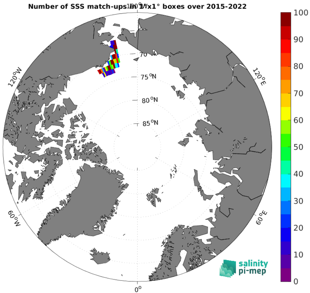
Figure 5: Number of SSS match-ups between TSG (SAMOS) SSS and the SMAP SSS L3 v5.3 - Monthly (RSS) SSS product for the Arctic Ocean Pi-MEP region over 1^\circ \times 1^\circ boxes and for the full satellite product period.
