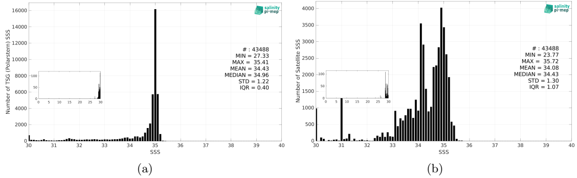
Figure 3: Histograms of SSS from TSG (Polarstern) (a) and SMAP SSS L3 v5.3 - Monthly (RSS) (b) considering all match-up pairs per bins of 0.1 over the Arctic Ocean Pi-MEP region and for the full satellite product period.
