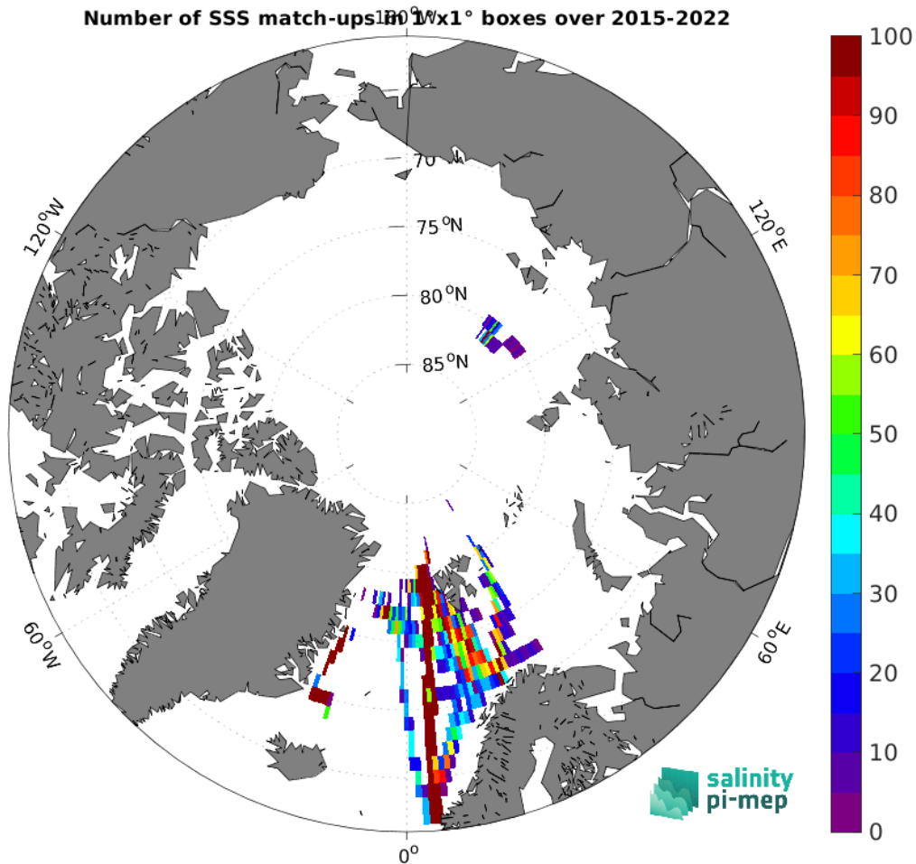
Figure 5: Number of SSS match-ups between TSG (Polarstern) SSS and the SMAP SSS L3 v5.3 - Monthly (RSS) SSS product for the Arctic Ocean Pi-MEP region over 1^\circ \times 1^\circ boxes and for the full satellite product period.
