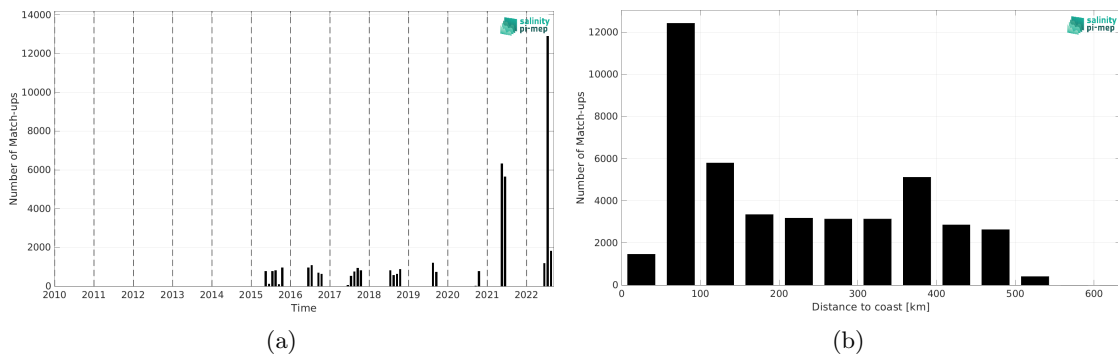
Figure 2: Number of match-ups between TSG (Polarstern) and SMAP SSS L3 v5.3 - Monthly (RSS) SSS as a function of time (a) and as function of the distance to coast (b) over the Arctic Ocean Pi-MEP region and for the full satellite product period.
