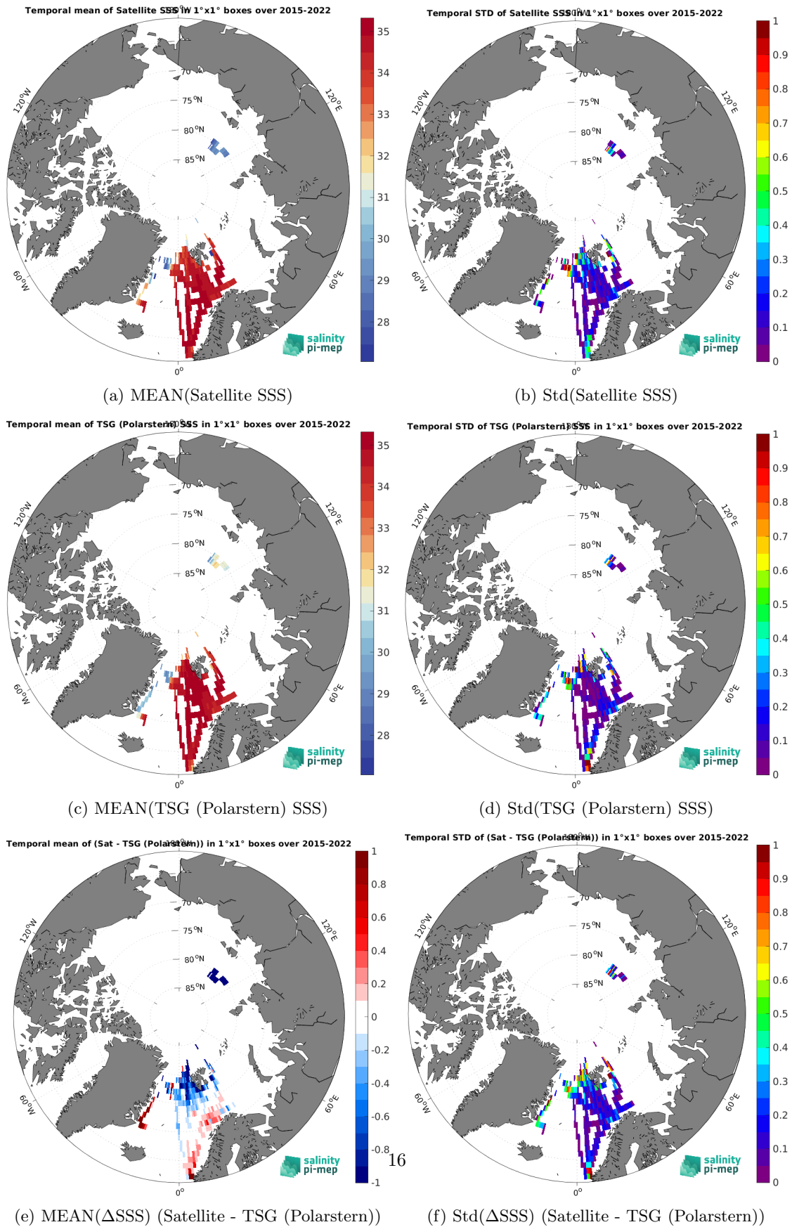
Figure 7: Temporal mean (left) and Std (right) of SSS from SMAP SSS L3 v5.3 - Monthly (RSS) (top), TSG (Polarstern) (middle), and of \Delta SSS (Satellite - TSG (Polarstern)). Only match-up pairs are used to generate these maps.
