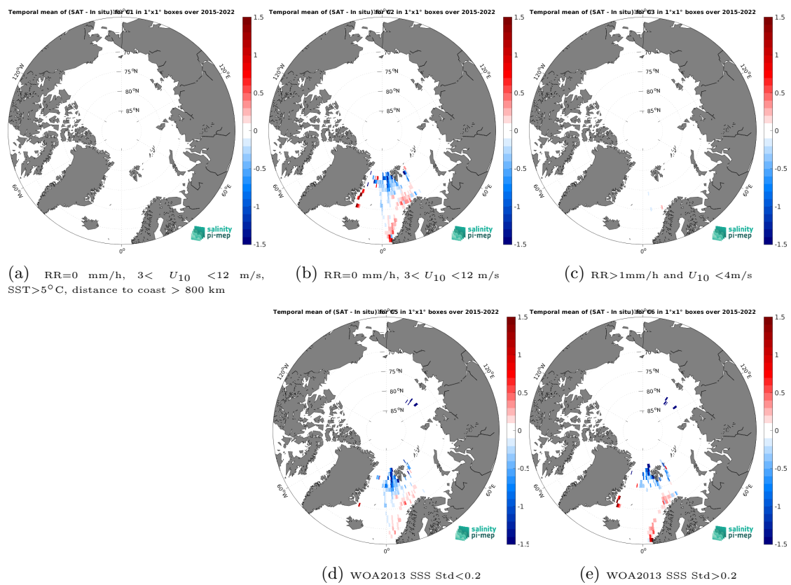
Figure 14: Temporal mean gridded over spatial boxes of size 1^\circ \times 1^\circ of \Delta SSS (SMAP SSS L3 v5.3 - Monthly (RSS) - TSG (Polarstern)) for 5 different subdatasets corresponding to: RR=0 mm/h, 3 < U_{10} < 12 m/s, SST > 5°C, distance to coast > 800 km (a), RR=0 mm/h, 3 < U_{10} < 12 m/s (b), RR > 1mm/h and U_{10} < 4 m/s (c), WOA2013 SSS Std < 0.2 (d), WOA2013 SSS Std > 0.2 (e).
