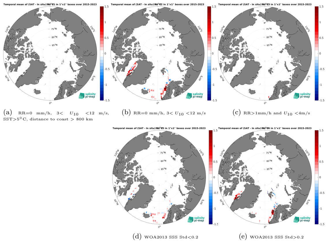
Figure 14: Temporal mean gridded over spatial boxes of size 1^\circ \times 1^\circ of \Delta SSS (SMAP SSS L3 v5.3 - Monthly (RSS) - TSG (LEGOS-DM)) for 5 different subdatasets corresponding to:RR=0 mm/h, 3 < U_{10} < 12 m/s, SST > 5°C, distance to coast > 800 km (a), RR=0 mm/h, 3 < U_{10} < 12 m/s (b), RR > 1mm/h and U_{10} < 4 m/s (c), WOA2013 SSS Std < 0.2 (d), WOA2013 SSS Std > 0.2 (e).
