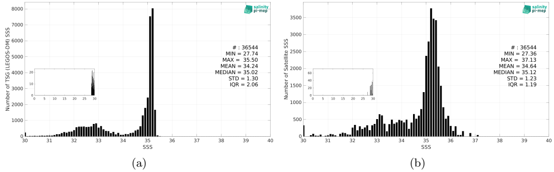
Figure 3: Histograms of SSS from TSG (LEGOS-DM) (a) and SMAP SSS L3 v5.3 - Monthly (RSS) (b) considering all match-up pairs per bins of 0.1 over the Arctic Ocean Pi-MEP region and for the full satellite product period.
