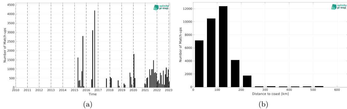
Figure 2: Number of match-ups between TSG (LEGOS-DM) and SMAP SSS L3 v5.3 - Monthly (RSS) SSS as a function of time (a) and as function of the distance to coast (b) over the Arctic Ocean Pi-MEP region and for the full satellite product period.
