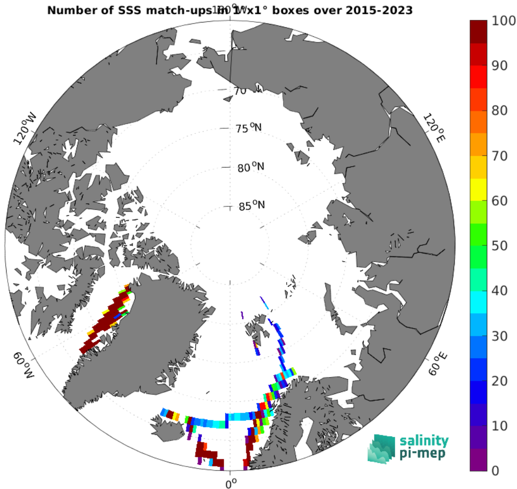
Figure 5: Number of SSS match-ups between TSG (LEGOS-DM) SSS and the SMAP SSS L3 v5.3 - Monthly (RSS) SSS product for the Arctic Ocean Pi-MEP region over 1^\circ \times 1^\circ boxes and for the full satellite product period.
