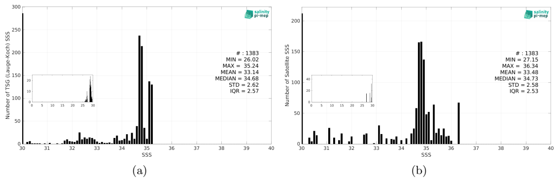
Figure 3: Histograms of SSS from TSG (Lauge-Koch) (a) and SMAP SSS L3 v5.3 - Monthly (RSS) (b) considering all match-up pairs per bins of 0.1 over the Arctic Ocean Pi-MEP region and for the full satellite product period.
