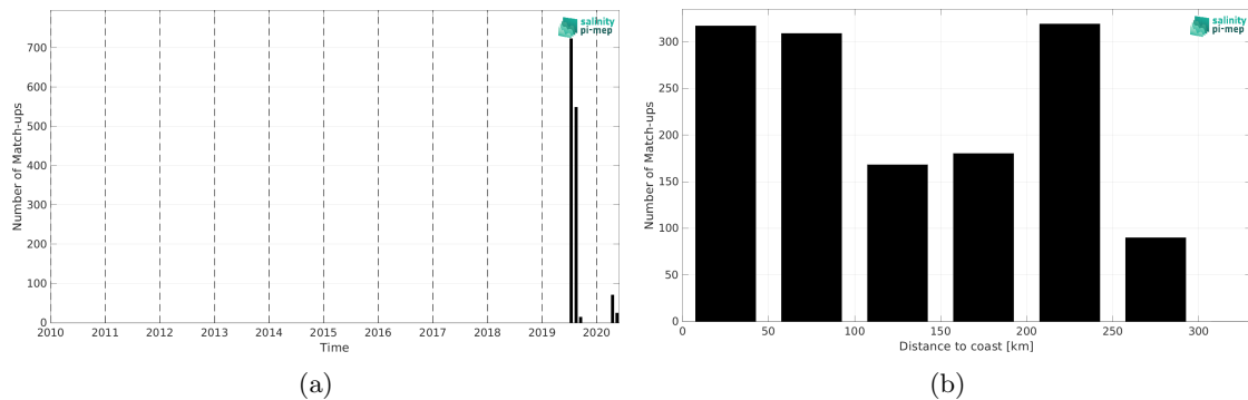
Figure 2: Number of match-ups between TSG (Lauge-Koch) and SMAP SSS L3 v5.3 - Monthly (RSS) SSS as a function of time (a) and as function of the distance to coast (b) over the Arctic Ocean Pi-MEP region and for the full satellite product period.
