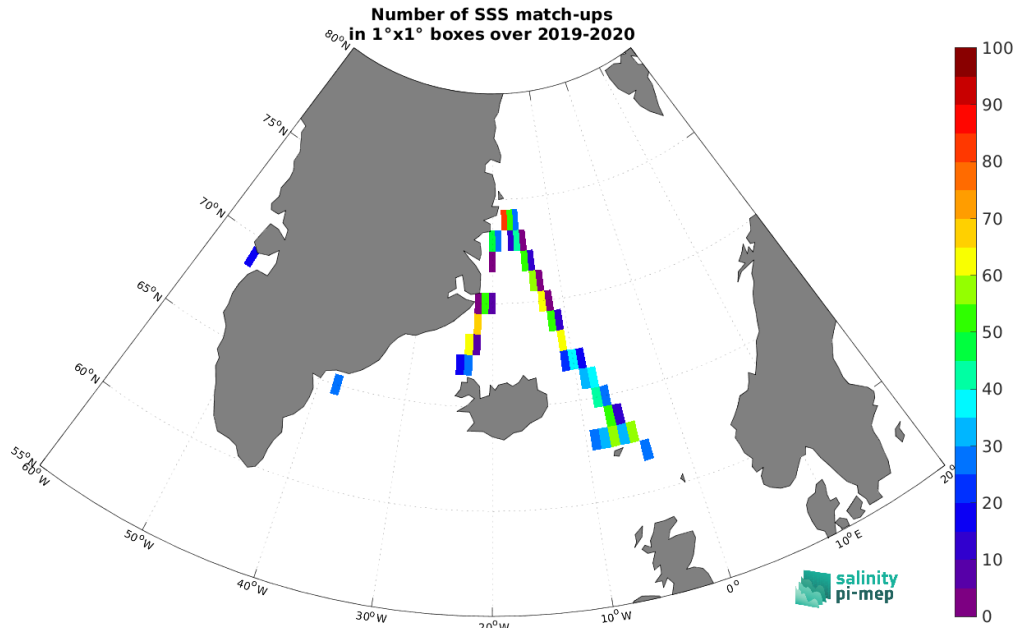
Figure 5: Number of SSS match-ups between TSG (Lauge-Koch) SSS and the SMAP SSS L3 v5.3 - Monthly (RSS) SSS product for the Arctic Ocean Pi-MEP region over 1^\circ \times 1^\circ boxes and for the full satellite product period.
