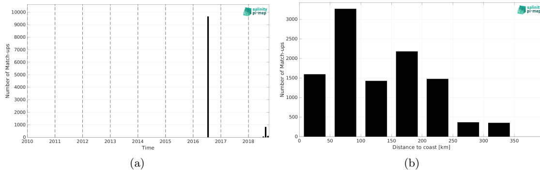
Figure 2: Number of match-ups between TSG (GOSUD-Research-vessel) and SMAP SSS L3 v5.3 - Monthly (RSS) SSS as a function of time (a) and as function of the distance to coast (b) over the Arctic Ocean Pi-MEP region and for the full satellite product period.
