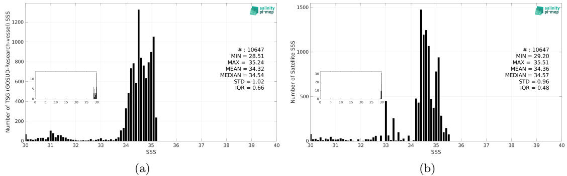
Figure 3: Histograms of SSS from TSG (GOSUD-Research-vessel) (a) and SMAP SSS L3 v5.3 - Monthly (RSS) (b) considering all match-up pairs per bins of 0.1 over the Arctic Ocean Pi-MEP region and for the full satellite product period.
