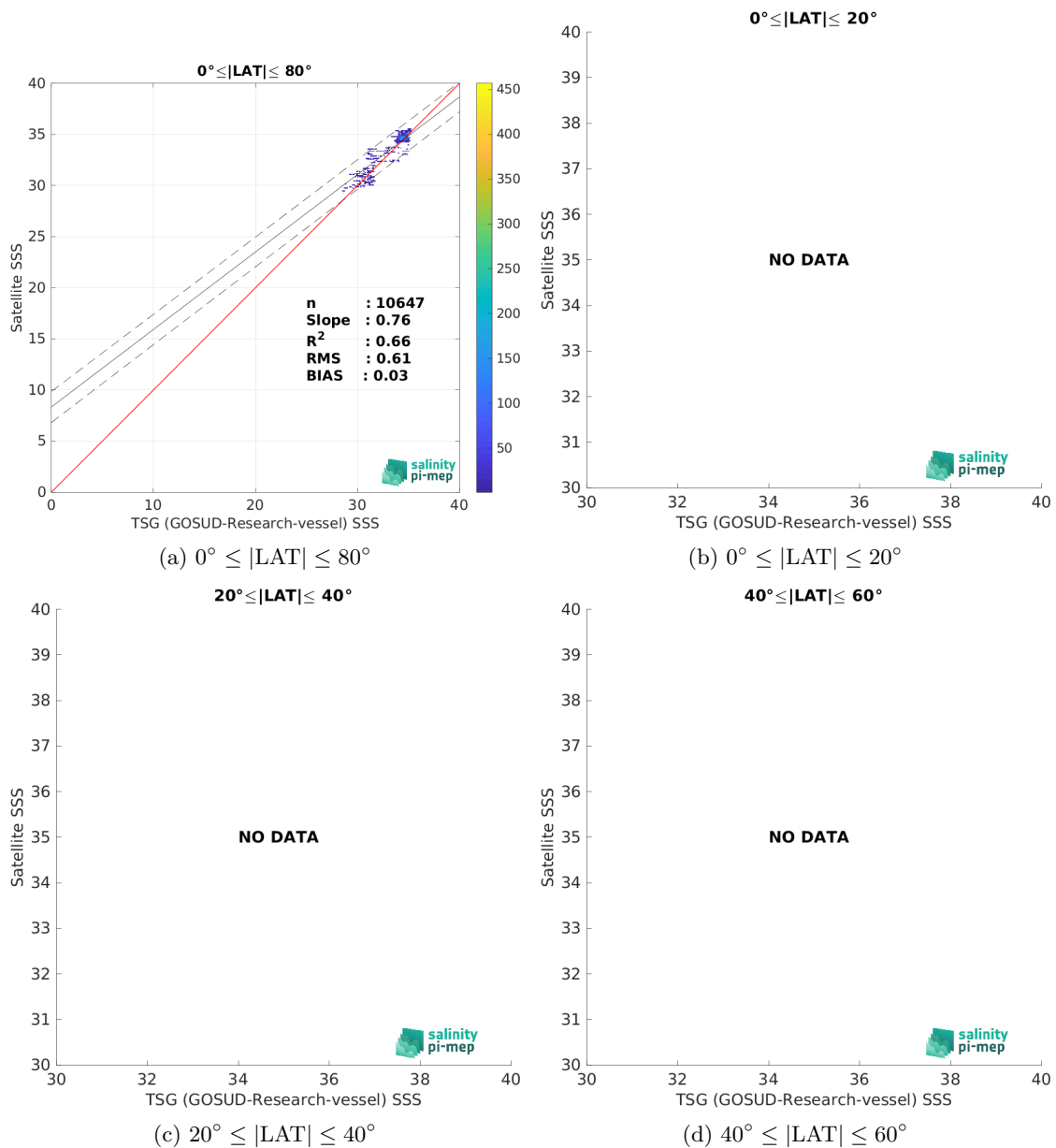
Figure 10: Contour maps of the concentration of SMAP SSS L3 v5.3 - Monthly (RSS) SSS (y-axis) versus TSG (GOSUD-Research-vessel) SSS (x-axis) at match-up pairs for different latitude bands. For each plot, the red line shows x=y . The black thin and dashed lines indicate a linear fit through the data cloud and the \pm 95\% confidence levels, respectively. The number match-up pairs n , the slope and R^2 coefficient of the linear fit, the root mean square (RMS) and the mean bias between satellite and in situ data are indicated for each latitude band in each plots.
