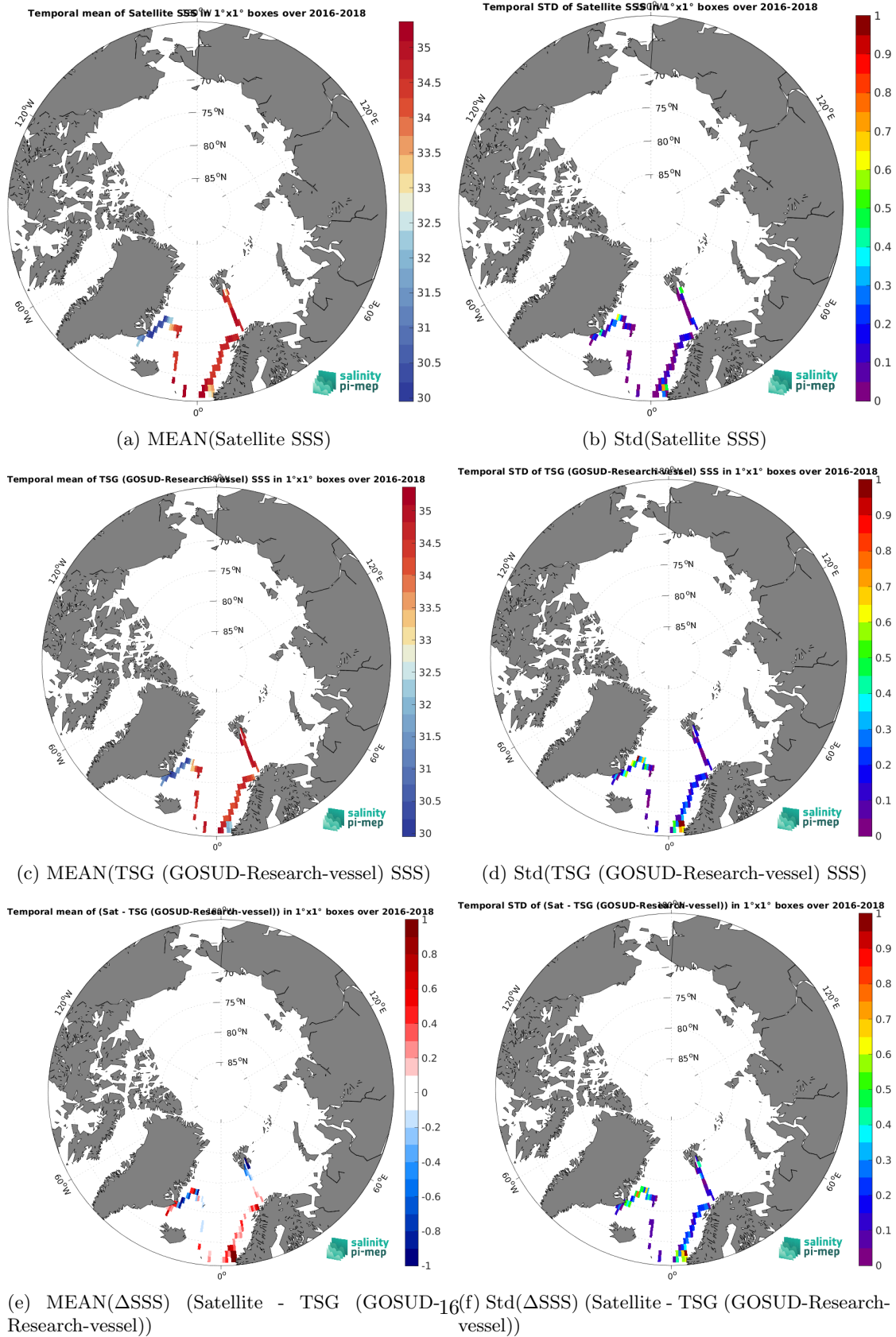
Figure 7: Temporal mean (left) and Std (right) of SSS from SMAP SSS L3 v5.3 - Monthly (RSS) (top), TSG (GOSUD-Research-vessel) (middle), and of \Delta SSS (Satellite - TSG (GOSUD-Research-vessel)). Only match-up pairs are used to generate these maps.
