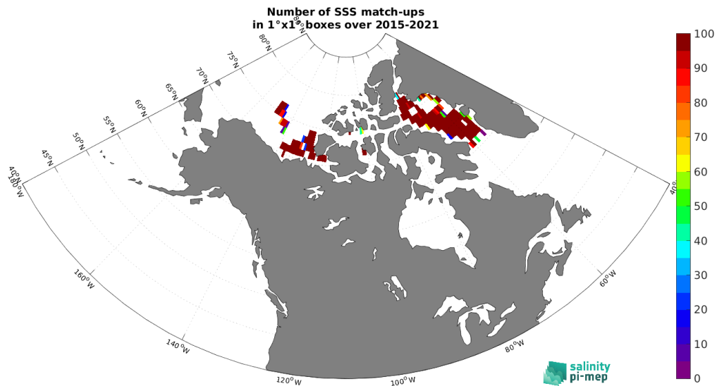
Figure 5: Number of SSS match-ups between TSG (Amundsen) SSS and the SMAP SSS L3 v5.3 - Monthly (RSS) SSS product for the Arctic Ocean Pi-MEP region over 1^\circ \times 1^\circ boxes and for the full satellite product period.
