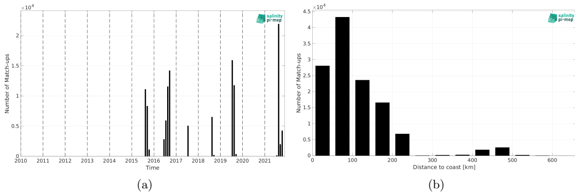
Figure 2: Number of match-ups between TSG (Amundsen) and SMAP SSS L3 v5.3 - Monthly (RSS) SSS as a function of time (a) and as function of the distance to coast (b) over the Arctic Ocean Pi-MEP region and for the full satellite product period.
