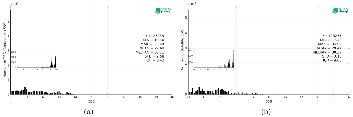
Figure 3: Histograms of SSS from TSG (Amundsen) (a) and SMAP SSS L3 v5.3 - Monthly (RSS) (b) considering all match-up pairs per bins of 0.1 over the Arctic Ocean Pi-MEP region and for the full satellite product period.
