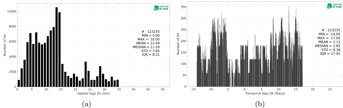
Figure 6: Histograms of the spatial (a) and temporal (b) lags between the location/time of the TSG (Amundsen) measurement and the date of the corresponding SMAP SSS L3 v5.3 - Monthly (RSS) SSS pixel.
