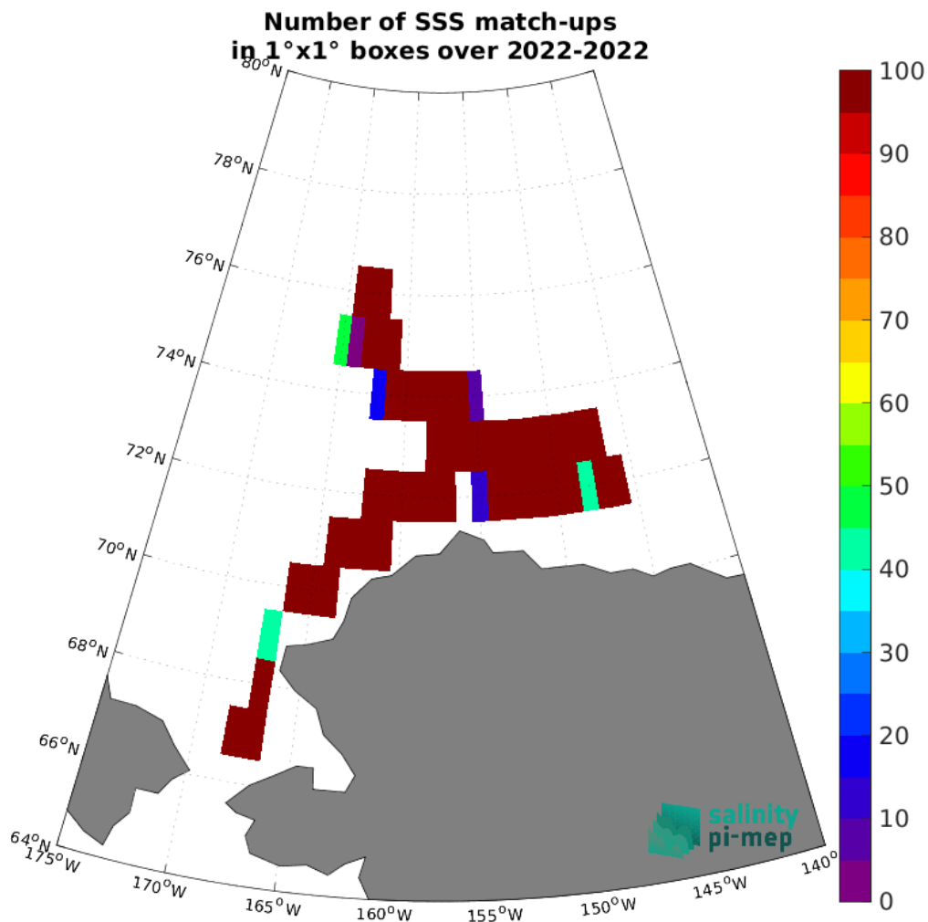
Figure 5: Number of SSS match-ups between SASSIE SSS and the SMAP SSS L3 v5.3 - Monthly (RSS) SSS product for the Arctic Ocean Pi-MEP region over 1^\circ \times 1^\circ boxes and for the full satellite product period.
