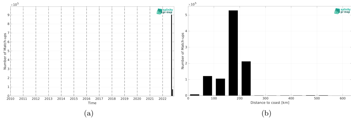
Figure 2: Number of match-ups between SASSIE and SMAP SSS L3 v5.3 - Monthly (RSS) SSS as a function of time (a) and as function of the distance to coast (b) over the Arctic Ocean Pi-MEP region and for the full satellite product period.
