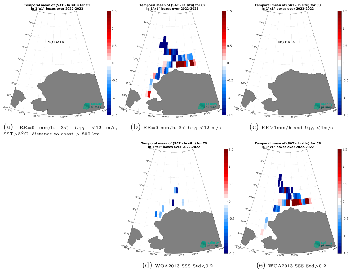
Figure 14: Temporal mean gridded over spatial boxes of size 1^\circ \times 1^\circ of \Delta\text{SSS} (SMAP SSS L3 v5.3 - Monthly (RSS) - SASSIE) for 5 different subdatasets corresponding to:RR=0 mm/h, 3 < U_{10} < 12 m/s, SST>5°C, distance to coast > 800 km (a), RR=0 mm/h, 3 < U_{10} < 12 m/s (b), RR>1mm/h and U_{10} < 4 m/s (c), WOA2013 SSS Std<0.2 (d), WOA2013 SSS Std>0.2 (e).
