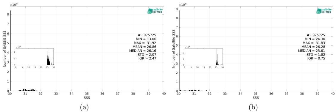
Figure 3: Histograms of SSS from SASSIE (a) and SMAP SSS L3 v5.3 - Monthly (RSS) (b) considering all match-up pairs per bins of 0.1 over the Arctic Ocean Pi-MEP region and for the full satellite product period.
