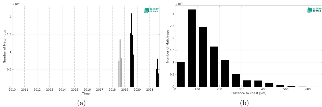
Figure 2: Number of match-ups between Saildrone and SMAP SSS L3 v5.3 - Monthly (RSS) SSS as a function of time (a) and as function of the distance to coast (b) over the Arctic Ocean Pi-MEP region and for the full satellite product period.
