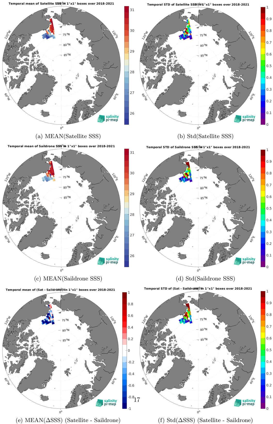
Figure 7: Temporal mean (left) and Std (right) of SSS from SMAP SSS L3 v5.3 - Monthly (RSS) (top), Saildrone (middle), and of \Delta SSS (Satellite - Saildrone). Only match-up pairs are used to generate these maps.
