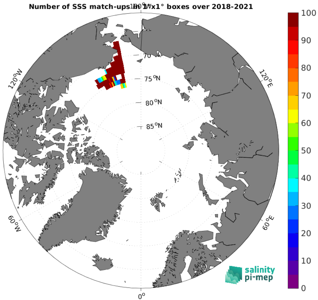
Figure 5: Number of SSS match-ups between Sailldrone SSS and the SMAP SSS L3 v5.3 - Monthly (RSS) SSS product for the Arctic Ocean Pi-MEP region over 1^\circ \times 1^\circ boxes and for the full satellite product period.
