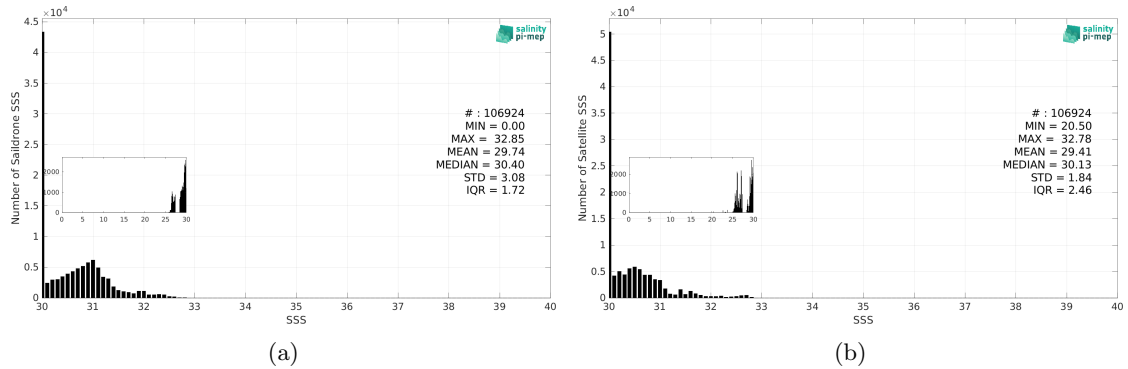
Figure 3: Histograms of SSS from Saildrone (a) and SMAP SSS L3 v5.3 - Monthly (RSS) (b) considering all match-up pairs per bins of 0.1 over the Arctic Ocean Pi-MEP region and for the full satellite product period.
