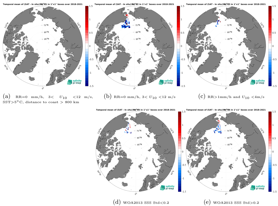
Figure 14: Temporal mean gridded over spatial boxes of size 1^\circ \times 1^\circ of \Delta SSS (SMAP SSS L3 v5.3 - Monthly (RSS) - Saildrone) for 5 different subdatasets corresponding to:RR=0 mm/h, 3 < U_{10} < 12 m/s, SST > 5°C, distance to coast > 800 km (a), RR=0 mm/h, 3 < U_{10} < 12 m/s (b), RR > 1mm/h and U_{10} < 4 m/s (c), WOA2013 SSS Std < 0.2 (d), WOA2013 SSS Std > 0.2 (e).
