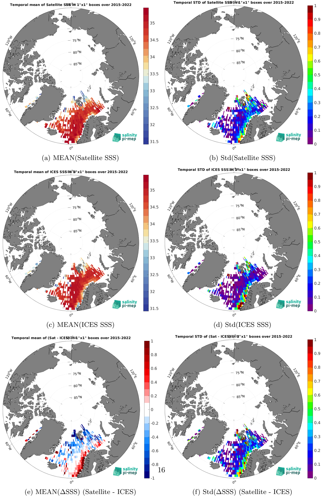
Figure 7: Temporal mean (left) and Std (right) of SSS from SMAP SSS L3 v5.3 - Monthly (RSS) (top), ICES (middle), and of \Delta SSS (Satellite - ICES). Only match-up pairs are used to generate these maps.
