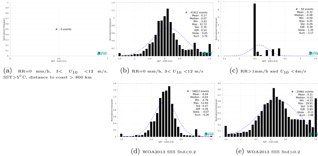
Figure 15: Normalized histogram of \Delta SSS (SMAP SSS L3 v5.3 - Monthly (RSS) - ICES) for 5 different subdatasets corresponding to: RR=0 mm/h, 3 < U_{10} < 12 m/s, SST > 5°C, distance to coast > 800 km (a), RR=0 mm/h, 3 < U_{10} < 12 m/s (b), RR > 1mm/h and U_{10} < 4 m/s (c), WOA2013 SSS Std < 0.2 (d), WOA2013 SSS Std > 0.2 (e).
