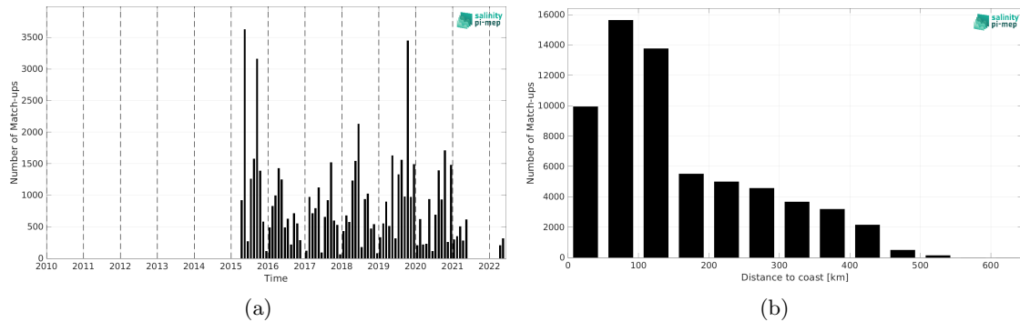
Figure 2: Number of match-ups between ICES and SMAP SSS L3 v5.3 - Monthly (RSS) SSS as a function of time (a) and as function of the distance to coast (b) over the Arctic Ocean Pi-MEP region and for the full satellite product period.
