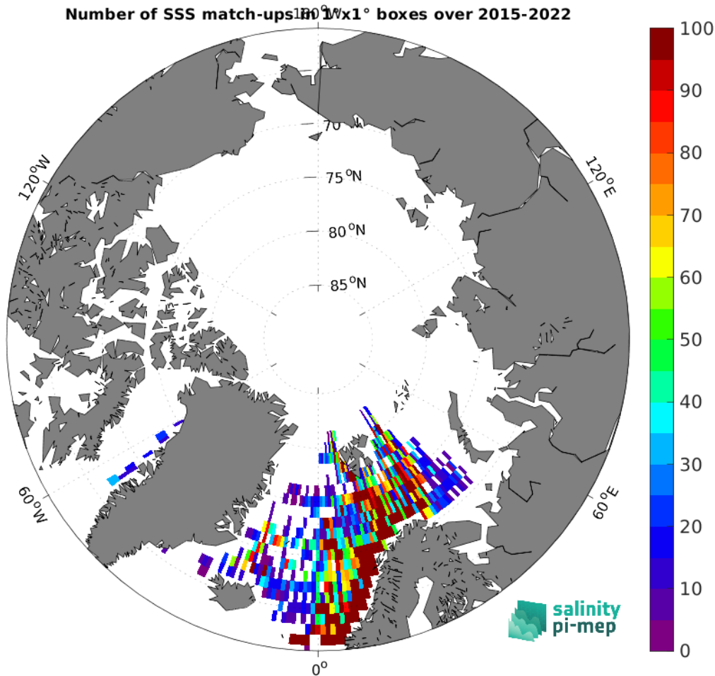
Figure 5: Number of SSS match-ups between ICES SSS and the SMAP SSS L3 v5.3 - Monthly (RSS) SSS product for the Arctic Ocean Pi-MEP region over 1^\circ \times 1^\circ boxes and for the full satellite product period.
