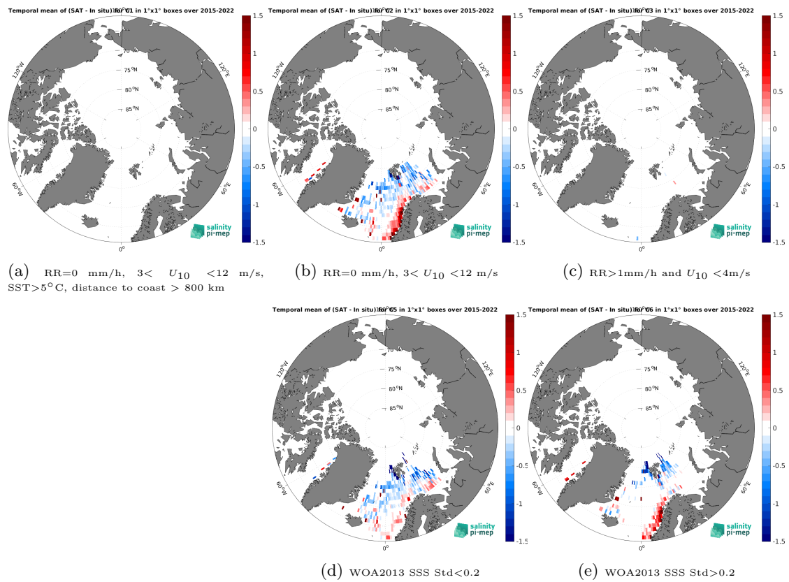
Figure 14: Temporal mean gridded over spatial boxes of size 1^\circ \times 1^\circ of \Delta SSS (SMAP SSS L3 v5.3 - Monthly (RSS) - ICES) for 5 different subdatasets corresponding to: RR=0 mm/h, 3 < U_{10} < 12 m/s, SST > 5°C, distance to coast > 800 km (a), RR=0 mm/h, 3 < U_{10} < 12 m/s (b), RR > 1mm/h and U_{10} < 4 m/s (c), WOA2013 SSS Std < 0.2 (d), WOA2013 SSS Std > 0.2 (e).
