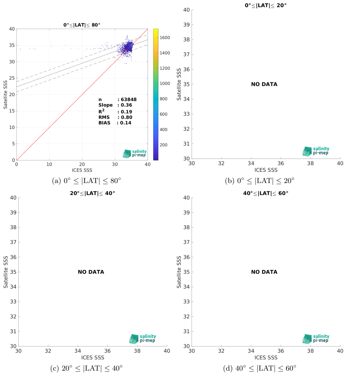
Figure 10: Contour maps of the concentration of SMAP SSS L3 v5.3 - Monthly (RSS) SSS (y-axis) versus ICES SSS (x-axis) at match-up pairs for different latitude bands. For each plot, the red line shows x=y . The black thin and dashed lines indicate a linear fit through the data cloud and the \pm 95\% confidence levels, respectively. The number match-up pairs n , the slope and R^2 coefficient of the linear fit, the root mean square (RMS) and the mean bias between satellite and in situ data are indicated for each latitude band in each plots.
