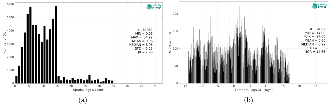
Figure 6: Histograms of the spatial (a) and temporal (b) lags between the location/time of the ICES measurement and the date of the corresponding SMAP SSS L3 v5.3 - Monthly (RSS) SSS pixel.
