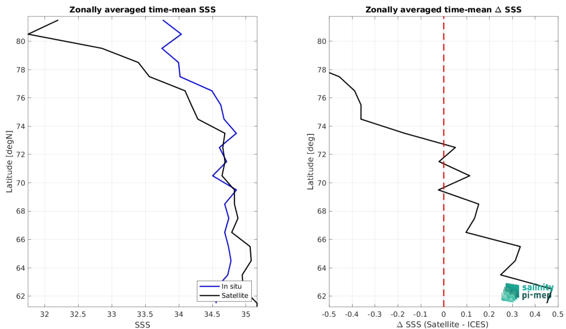
Figure 9: Left panel: Zonal mean SSS from SMAP SSS L3 v5.3 - Monthly (RSS) satellite product (black) and from ICES (blue). Right panel: Zonal mean of \Delta SSS (Satellite - ICES) for all the collected Pi-MEP match-up pairs estimated over the full satellite product period.
