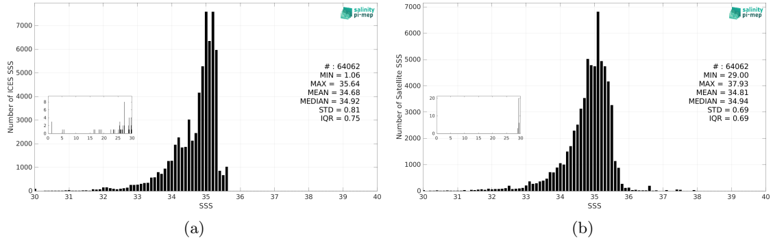
Figure 3: Histograms of SSS from ICES (a) and SMAP SSS L3 v5.3 - Monthly (RSS) (b) considering all match-up pairs per bins of 0.1 over the Arctic Ocean Pi-MEP region and for the full satellite product period.
