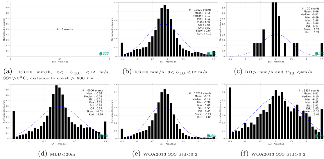
Figure 15: Normalized histogram of \Delta\text{SSS} (SMAP SSS L3 v5.3 - Monthly (RSS) - Argo) for 6 different subdatasets corresponding to: RR=0 mm/h, 3 < U_{10} < 12 m/s, SST>5°C, distance to coast > 800 km (a), RR=0 mm/h, 3 < U_{10} < 12 m/s (b), RR>1mm/h and U_{10} < 4 m/s (c), MLD<20m (d), WOA2013 SSS Std<0.2 (e), WOA2013 SSS Std>0.2 (f).
