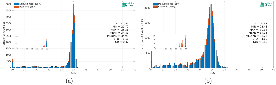
Figure 3: Histograms of SSS from Argo (a) and SMAP SSS L3 v5.3 - Monthly (RSS) (b) considering all match-up pairs per bins of 0.1 over the Arctic Ocean Pi-MEP region and for the full satellite product period.
