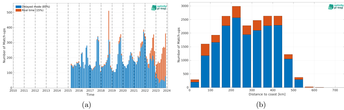
Figure 2: Number of match-ups between Argo and SMAP SSS L3 v5.3 - Monthly (RSS) SSS as a function of time (a) and as function of the distance to coast (b) over the Arctic Ocean Pi-MEP region and for the full satellite product period.
