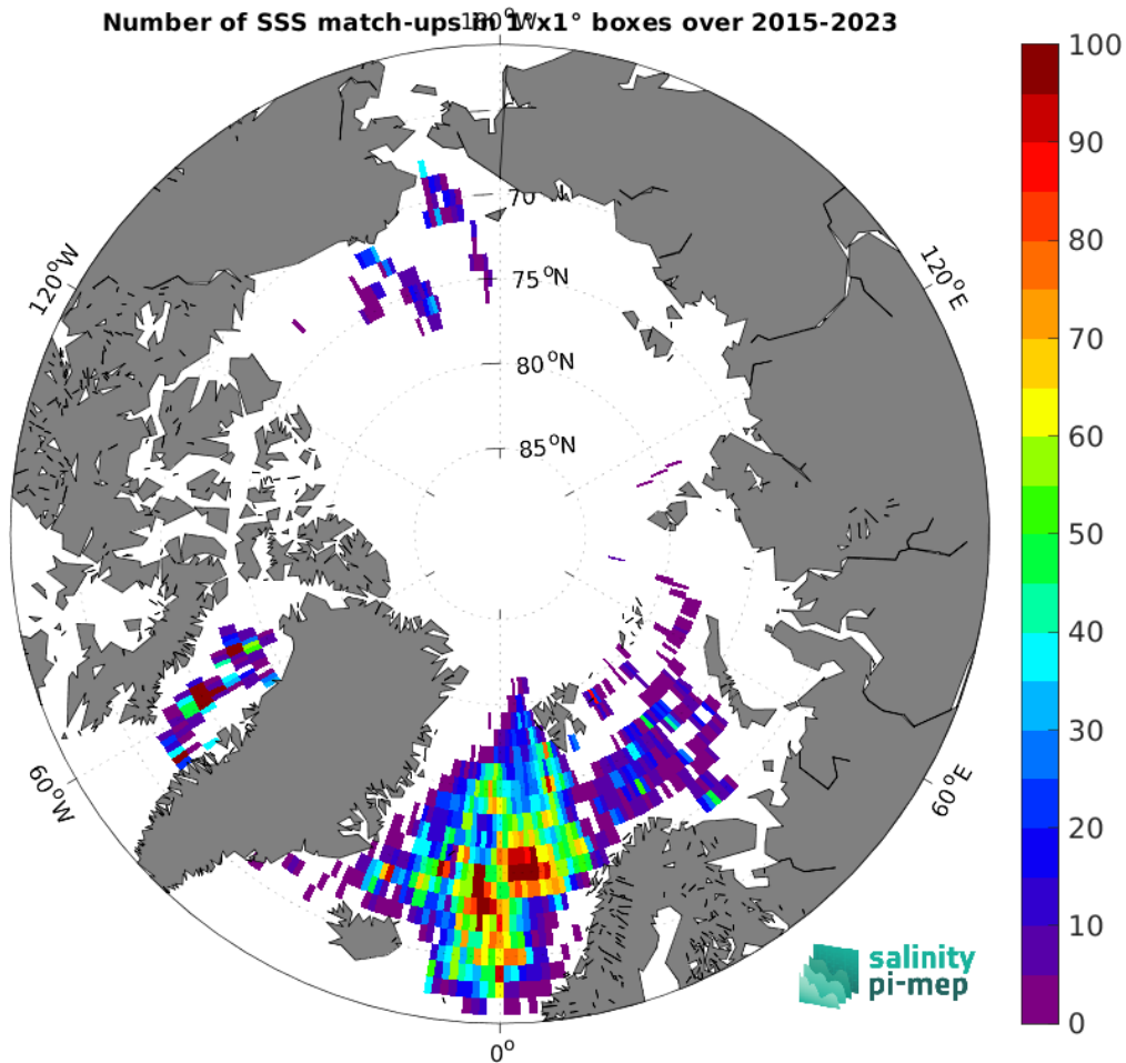
Figure 5: Number of SSS match-ups between Argo SSS and the SMAP SSS L3 v5.3 - Monthly (RSS) SSS product for the Arctic Ocean Pi-MEP region over 1^\circ \times 1^\circ boxes and for the full satellite product period.
