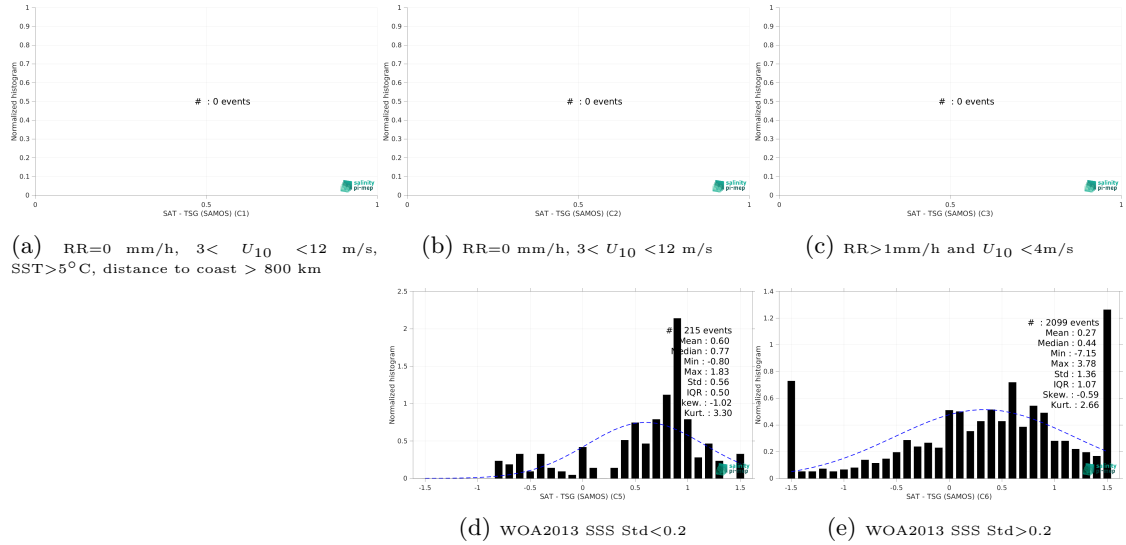
Figure 13: Normalized histogram of \Delta SSS (SMAP SSS L3 v5 - 8-Day running (RSS) - TSG (SAMOS)) for 5 different subdatasets corresponding to: RR=0 mm/h, 3 < U_{10} < 12 m/s, SST >5^{\circ} C, distance to coast > 800 km (a), RR=0 mm/h, 3 < U_{10} < 12 m/s (b), RR >1 mm/h and U_{10} < 4 m/s (c), WOA2013 SSS Std <0.2 (d), WOA2013 SSS Std >0.2 (e).
