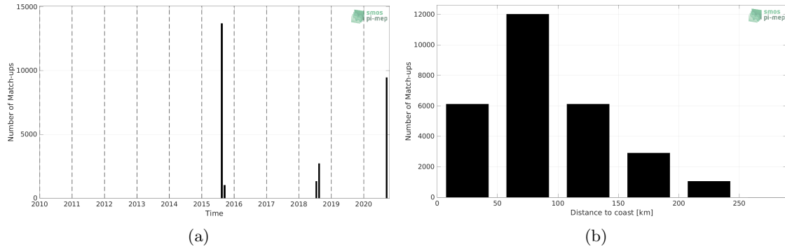
Figure 1: Number of match-ups between TSG (SAMOS) and SMAP SSS L3 v5 - 8-Day running (RSS) SSS as a function of time (a) and as function of the distance to coast (b) over the Arctic Ocean Pi-MEP region and for the full satellite product period.
