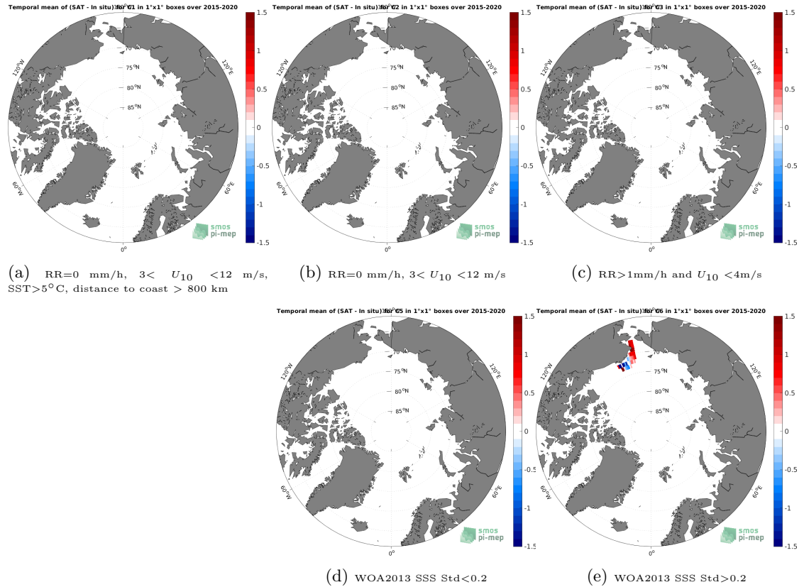
Figure 12: Temporal mean gridded over spatial boxes of size 1^{\circ}\times 1^{\circ} of \Delta\text{SSS} (SMAP SSS L3 v5 - 8-Day running (RSS) - TSG (SAMOS)) for 5 different subdatasets corresponding to:RR=0 mm/h, 3 < U_{10} < 12 m/s, SST >5^{\circ}\text{C} , distance to coast > 800 km (a), RR=0 mm/h, 3 < U_{10} < 12 m/s (b), RR >1 mm/h and U_{10} < 4 m/s (c), WOA2013 SSS Std <0.2 (d), WOA2013 SSS Std >0.2 (e).
