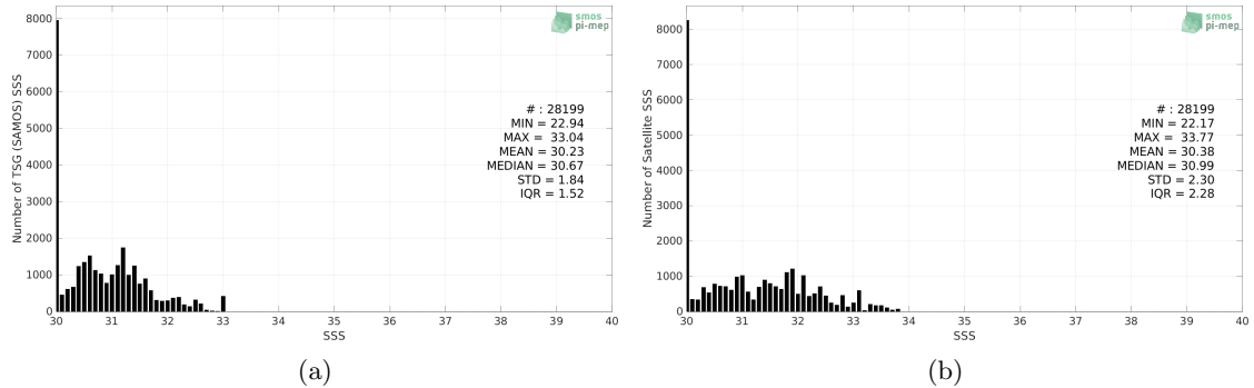
Figure 2: Histograms of SSS from TSG (SAMOS) (a) and SMAP SSS L3 v5 - 8-Day running (RSS) (b) considering all match-up pairs per bins of 0.1 over the Arctic Ocean Pi-MEP region and for the full satellite product period.
