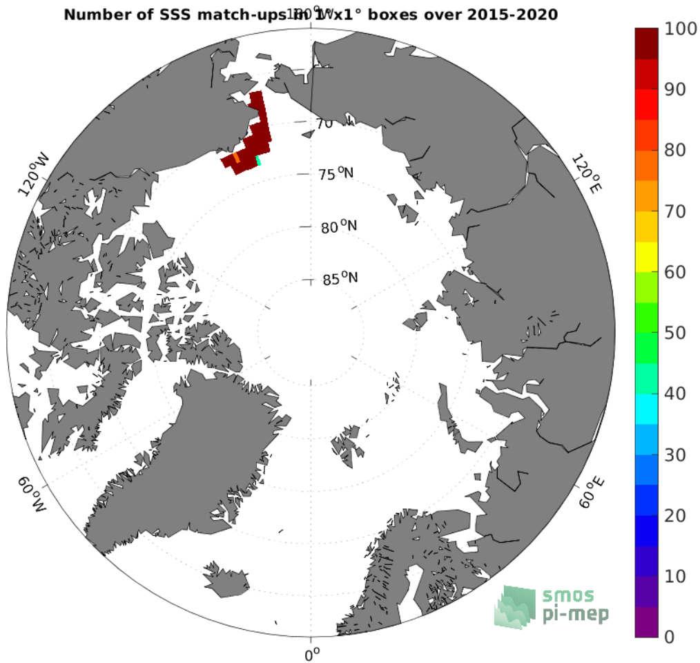
Figure 4: Number of SSS match-ups between TSG (SAMOS) SSS and the SMAP SSS L3 v5 - 8-Day running (RSS) SSS product for the Arctic Ocean Pi-MEP region over 1^\circ \times 1^\circ boxes and for the full satellite product period.
