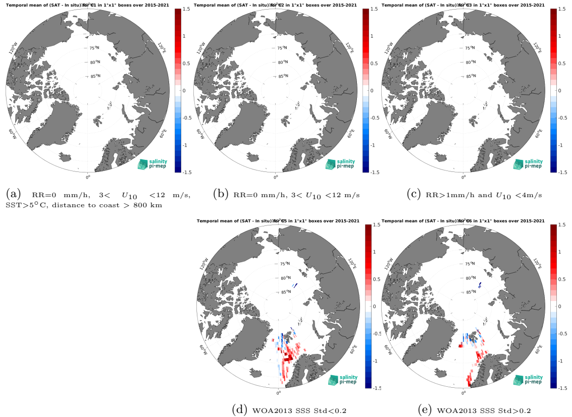
Figure 12: Temporal mean gridded over spatial boxes of size 1^{\circ}\times 1^{\circ} of \Delta\text{SSS} (SMAP SSS L3 v5 - 8-Day running (RSS) - TSG (Polarstern)) for 5 different subdatasets corresponding to:RR=0 mm/h, 3 < U_{10} < 12 m/s, SST >5^{\circ}\text{C} , distance to coast > 800 km (a), RR=0 mm/h, 3 < U_{10} < 12 m/s (b), RR >1 mm/h and U_{10} < 4 m/s (c), WOA2013 SSS Std <0.2 (d), WOA2013 SSS Std >0.2 (e).
