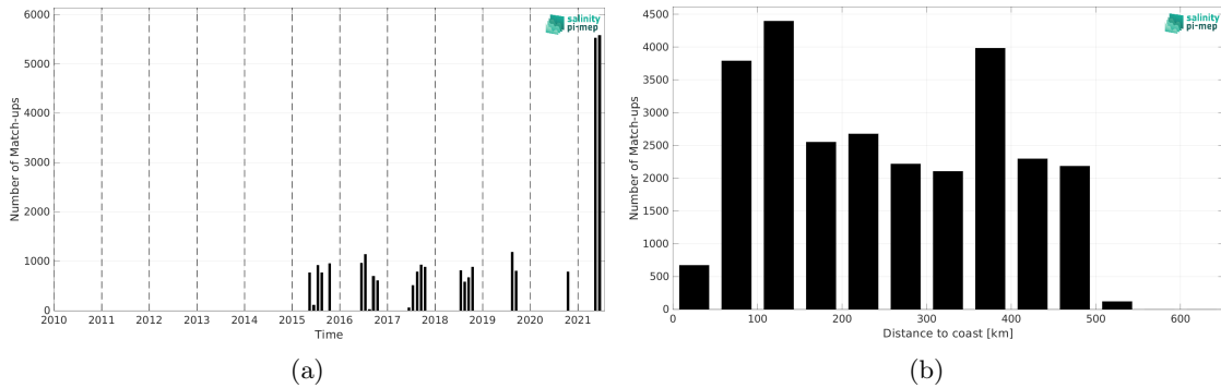
Figure 1: Number of match-ups between TSG (Polarstern) and SMAP SSS L3 v5 - 8-Day running (RSS) SSS as a function of time (a) and as function of the distance to coast (b) over the Arctic Ocean Pi-MEP region and for the full satellite product period.
