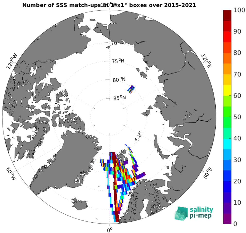
Figure 4: Number of SSS match-ups between TSG (Polarstern) SSS and the SMAP SSS L3 v5 - 8-Day running (RSS) SSS product for the Arctic Ocean Pi-MEP region over 1^\circ \times 1^\circ boxes and for the full satellite product period.
