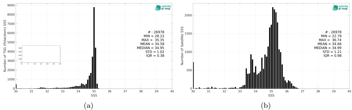
Figure 2: Histograms of SSS from TSG (Polarstern) (a) and SMAP SSS L3 v5 - 8-Day running (RSS) (b) considering all match-up pairs per bins of 0.1 over the Arctic Ocean Pi-MEP region and for the full satellite product period.
