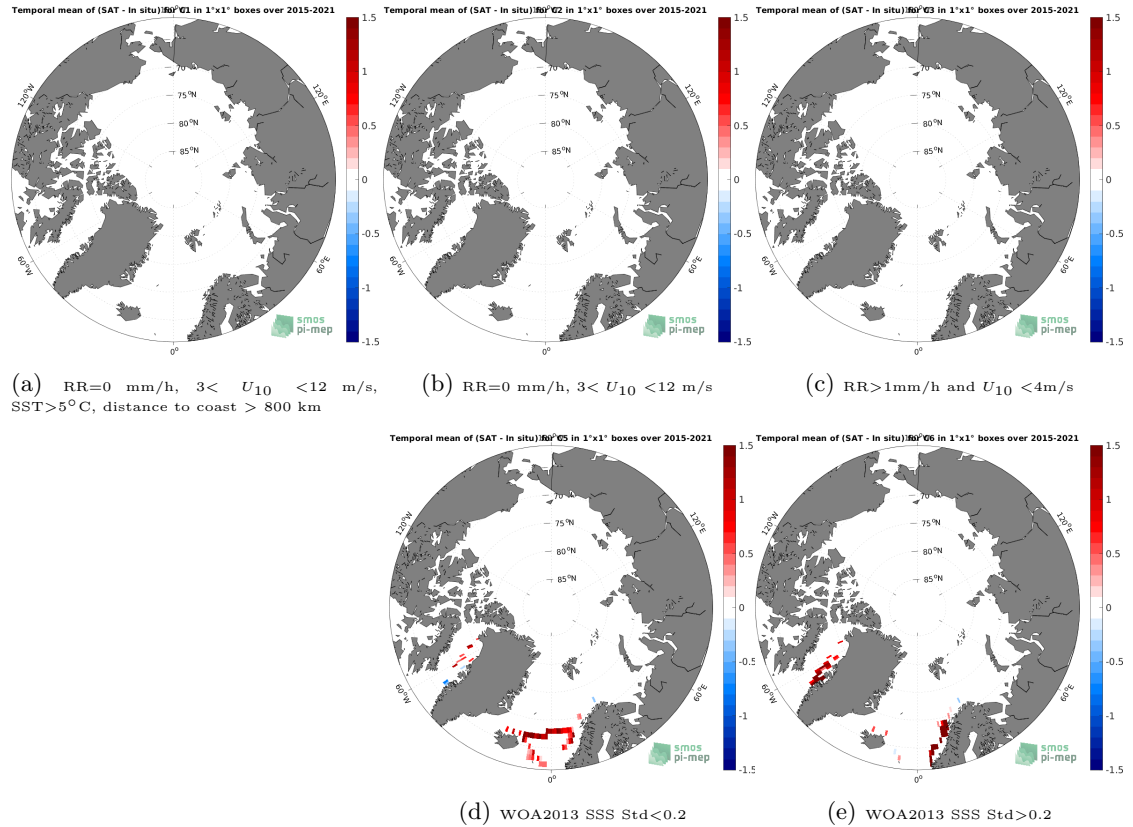
Figure 12: Temporal mean gridded over spatial boxes of size 1^{\circ}\times 1^{\circ} of \Delta\text{SSS} (SMAP SSS L3 v5 - 8-Day running (RSS) - TSG (LEGOS-DM)) for 5 different subdatasets corresponding to:RR=0 mm/h, 3 < U_{10} < 12 m/s, SST >5^{\circ}\text{C} , distance to coast > 800 km (a), RR=0 mm/h, 3 < U_{10} < 12 m/s (b), RR >1 mm/h and U_{10} < 4 m/s (c), WOA2013 SSS Std <0.2 (d), WOA2013 SSS Std >0.2 (e).
