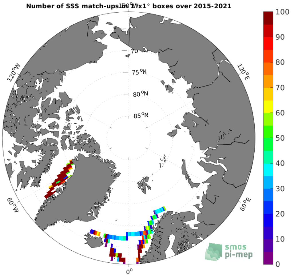
Figure 4: Number of SSS match-ups between TSG (LEGOS-DM) SSS and the SMAP SSS L3 v5 - 8-Day running (RSS) SSS product for the Arctic Ocean Pi-MEP region over 1^{\circ} \times 1^{\circ} boxes and for the full satellite product period.
