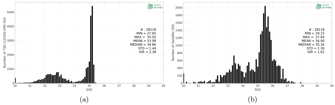
Figure 2: Histograms of SSS from TSG (LEGOS-DM) (a) and SMAP SSS L3 v5 - 8-Day running (RSS) (b) considering all match-up pairs per bins of 0.1 over the Arctic Ocean Pi-MEP region and for the full satellite product period.
