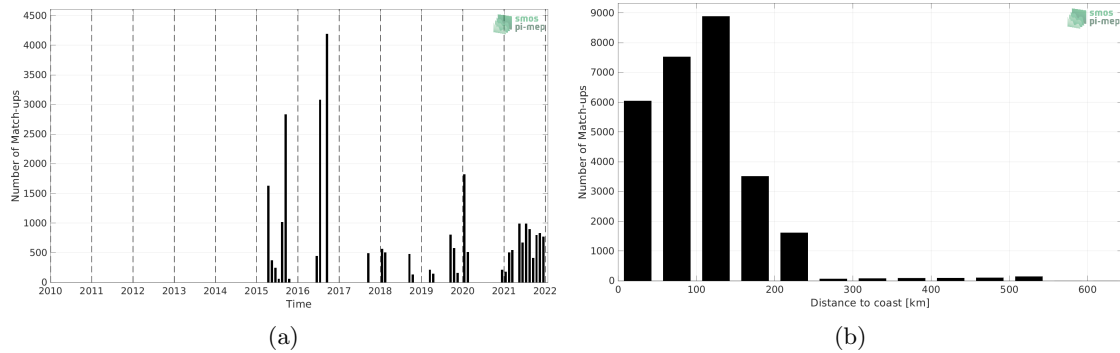
Figure 1: Number of match-ups between TSG (LEGOS-DM) and SMAP SSS L3 v5 - 8-Day running (RSS) SSS as a function of time (a) and as function of the distance to coast (b) over the Arctic Ocean Pi-MEP region and for the full satellite product period.
