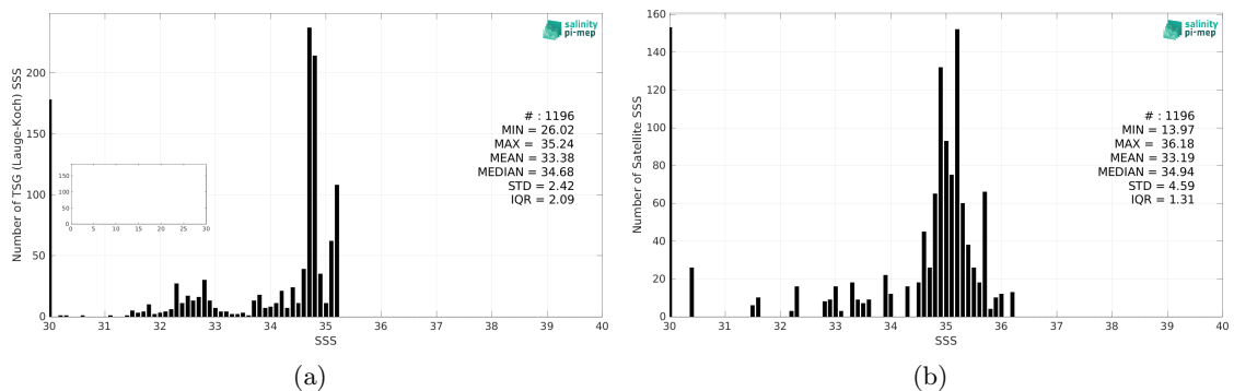
Figure 2: Histograms of SSS from TSG (Lauge-Koch) (a) and SMAP SSS L3 v5 - 8-Day running (RSS) (b) considering all match-up pairs per bins of 0.1 over the Arctic Ocean Pi-MEP region and for the full satellite product period.
