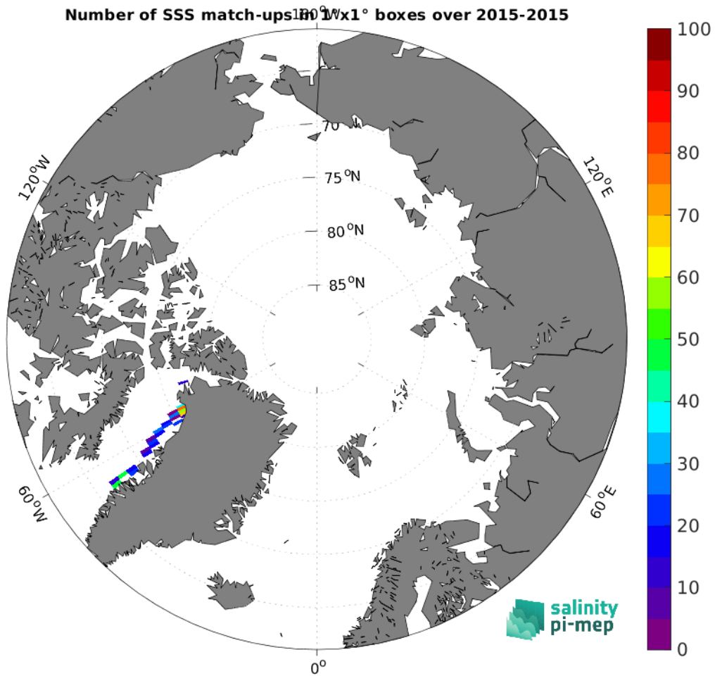
Figure 4: Number of SSS match-ups between TSG (GOSUD-Sailing-ship) SSS and the SMAP SSS L3 v5 - 8-Day running (RSS) SSS product for the Arctic Ocean Pi-MEP region over 1^\circ \times 1^\circ boxes and for the full satellite product period.
