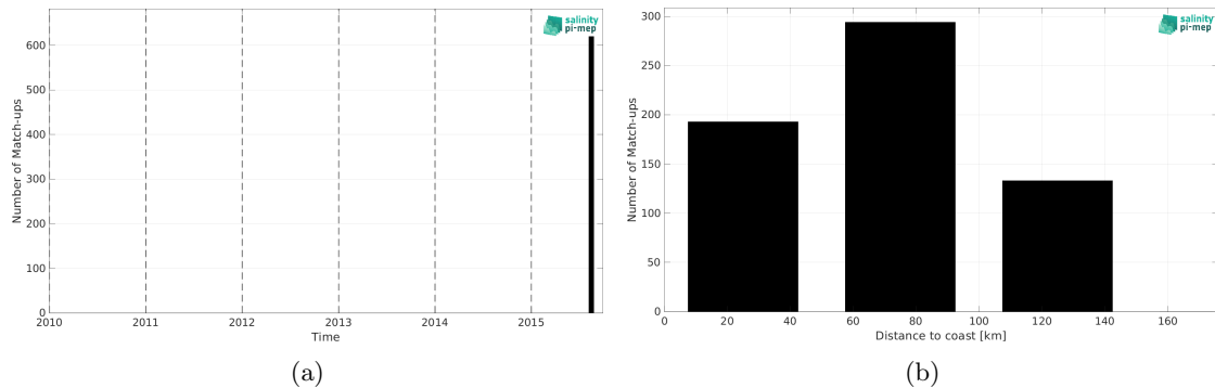
Figure 1: Number of match-ups between TSG (GOSUD-Sailing-ship) and SMAP SSS L3 v5 - 8-Day running (RSS) SSS as a function of time (a) and as function of the distance to coast (b) over the Arctic Ocean Pi-MEP region and for the full satellite product period.
