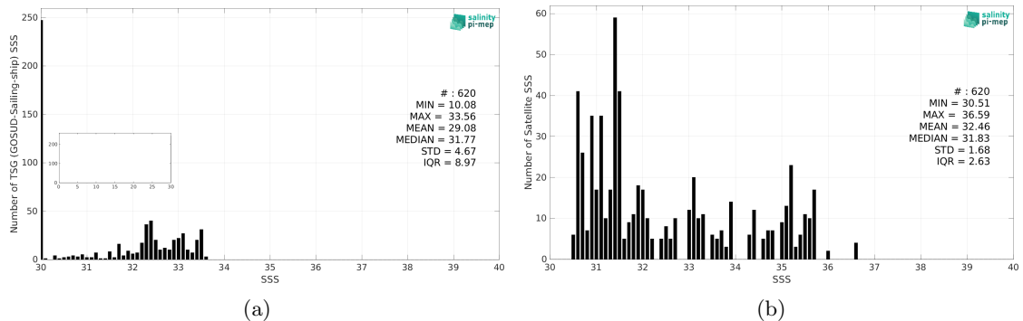
Figure 2: Histograms of SSS from TSG (GOSUD-Sailing-ship) (a) and SMAP SSS L3 v5 - 8-Day running (RSS) (b) considering all match-up pairs per bins of 0.1 over the Arctic Ocean Pi-MEP region and for the full satellite product period.
