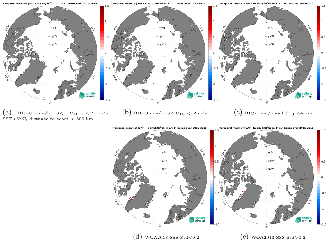
Figure 12: Temporal mean gridded over spatial boxes of size 1^{\circ} \times 1^{\circ} of \Delta SSS (SMAP SSS L3 v5 - 8-Day running (RSS) - TSG (GOSUD-Sailing-ship)) for 5 different subdatasets corresponding to: RR=0 mm/h, 3 < U_{10} < 12 m/s, SST > 5^{\circ}C , distance to coast > 800 km (a), RR=0 mm/h, 3 < U_{10} < 12 m/s (b), RR > 1 mm/h and U_{10} < 4 m/s (c), WOA2013 SSS Std < 0.2 (d), WOA2013 SSS Std > 0.2 (e).
