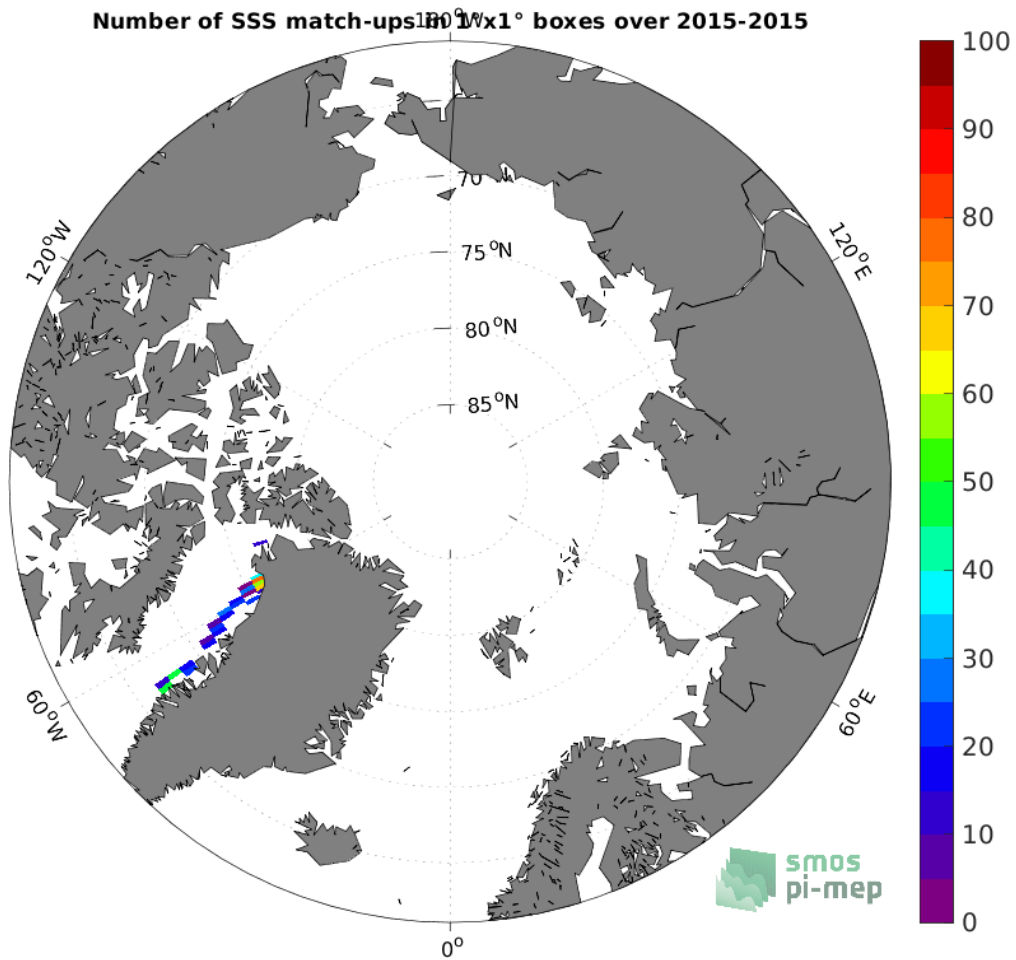
Figure 4: Number of SSS match-ups between TSG (GOSUD-Sailing-ship) SSS and the SMAP SSS L3 v5 - 8-Day running (RSS) SSS product for the Arctic Ocean Pi-MEP region over 1^{\circ} \times 1^{\circ} boxes and for the full satellite product period.
