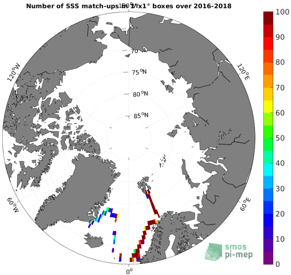
Figure 4: Number of SSS match-ups between TSG (GOSUD-Research-vessel) SSS and the SMAP SSS L3 v5 - 8-Day running (RSS) SSS product for the Arctic Ocean Pi-MEP region over 1^\circ \times 1^\circ boxes and for the full satellite product period.
