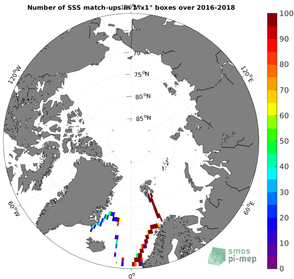
Figure 4: Number of SSS match-ups between TSG (GOSUD-Research-vessel) SSS and the SMAP SSS L3 v5 - 8-Day running (RSS) SSS product for the Arctic Ocean Pi-MEP region over 1^{\circ} \times 1^{\circ} boxes and for the full satellite product period.
