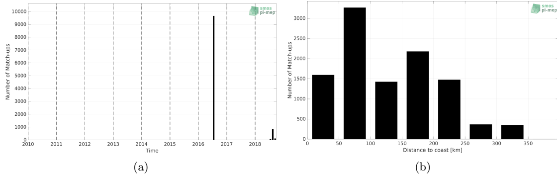
Figure 1: Number of match-ups between TSG (GOSUD-Research-vessel) and SMAP SSS L3 v5 - 8-Day running (RSS) SSS as a function of time (a) and as function of the distance to coast (b) over the Arctic Ocean Pi-MEP region and for the full satellite product period.
