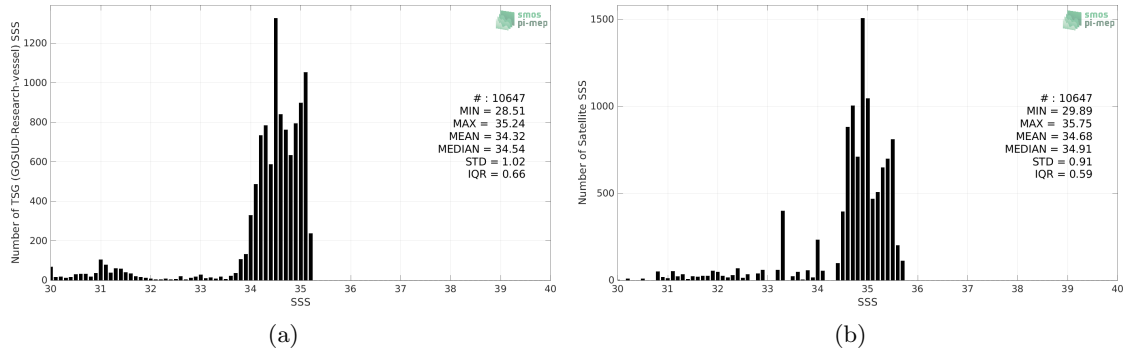
Figure 2: Histograms of SSS from TSG (GOSUD-Research-vessel) (a) and SMAP SSS L3 v5 - 8-Day running (RSS) (b) considering all match-up pairs per bins of 0.1 over the Arctic Ocean Pi-MEP region and for the full satellite product period.
