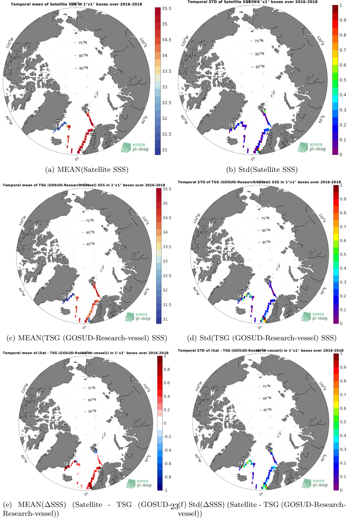
Figure 6: Temporal mean (left) and Std (right) of SSS from SMAP SSS L3 v5 - 8-Day running (RSS) (top), TSG (GOSUD-Research-vessel) (middle), and of \Delta SSS (Satellite - TSG (GOSUD-Research-vessel)). Only match-up pairs are used to generate these maps.
