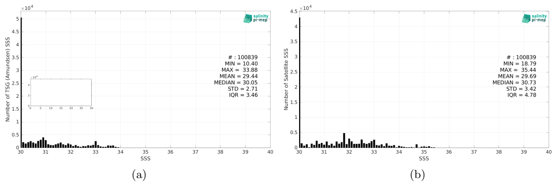
Figure 2: Histograms of SSS from TSG (Amundsen) (a) and SMAP SSS L3 v5 - 8-Day running (RSS) (b) considering all match-up pairs per bins of 0.1 over the Arctic Ocean Pi-MEP region and for the full satellite product period.
