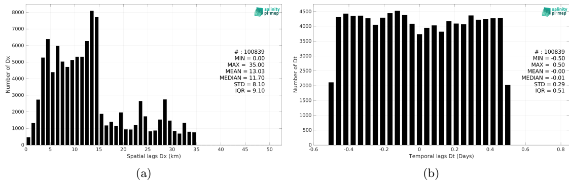
Figure 5: Histograms of the spatial (a) and temporal (b) lags between the location/time of the TSG (Amundsen) measurement and the date of the corresponding SMAP SSS L3 v5 - 8-Day running (RSS) SSS pixel.
