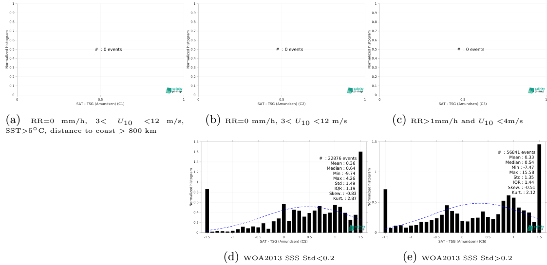
Figure 13: Normalized histogram of \Delta SSS (SMAP SSS L3 v5 - 8-Day running (RSS) - TSG (Amundsen)) for 5 different subdatasets corresponding to: RR=0 mm/h, 3 < U_{10} < 12 m/s, SST>5°C, distance to coast > 800 km (a), RR=0 mm/h, 3 < U_{10} < 12 m/s (b), RR>1mm/h and U_{10} < 4 m/s (c), WOA2013 SSS Std<0.2 (d), WOA2013 SSS Std>0.2 (e).
