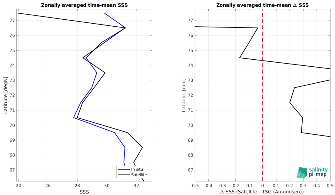
Figure 8: Left panel: Zonal mean SSS from SMAP SSS L3 v5 - 8-Day running (RSS) satellite product (black) and from TSG (Amundsen) (blue). Right panel: Zonal mean of \Delta SSS (Satellite - TSG (Amundsen)) for all the collected Pi-MEP match-up pairs estimated over the full satellite product period.
