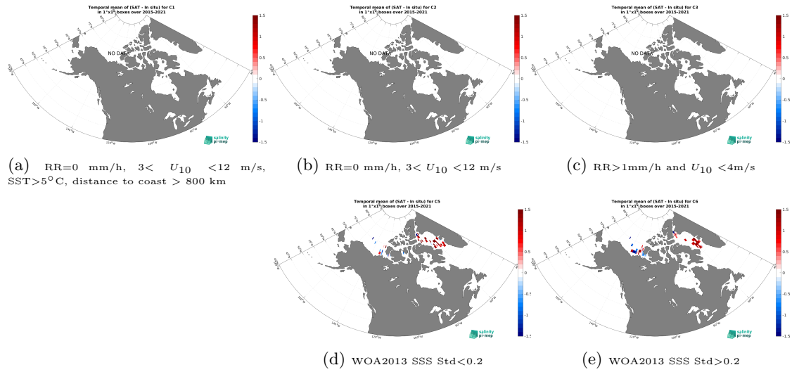
Figure 12: Temporal mean gridded over spatial boxes of size 1^{\circ}\times 1^{\circ} of \Delta\text{SSS} (SMAP SSS L3 v5 - 8-Day running (RSS) - TSG (Amundsen)) for 5 different subdatasets corresponding to:RR=0 mm/h, 3 < U_{10} < 12 m/s, SST >5^{\circ}\text{C} , distance to coast > 800 km (a), RR=0 mm/h, 3 < U_{10} < 12 m/s (b), RR >1 mm/h and U_{10} < 4 m/s (c), WOA2013 SSS Std <0.2 (d), WOA2013 SSS Std >0.2 (e).
