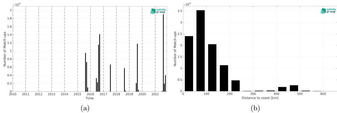
Figure 1: Number of match-ups between TSG (Amundsen) and SMAP SSS L3 v5 - 8-Day running (RSS) SSS as a function of time (a) and as function of the distance to coast (b) over the Arctic Ocean Pi-MEP region and for the full satellite product period.
