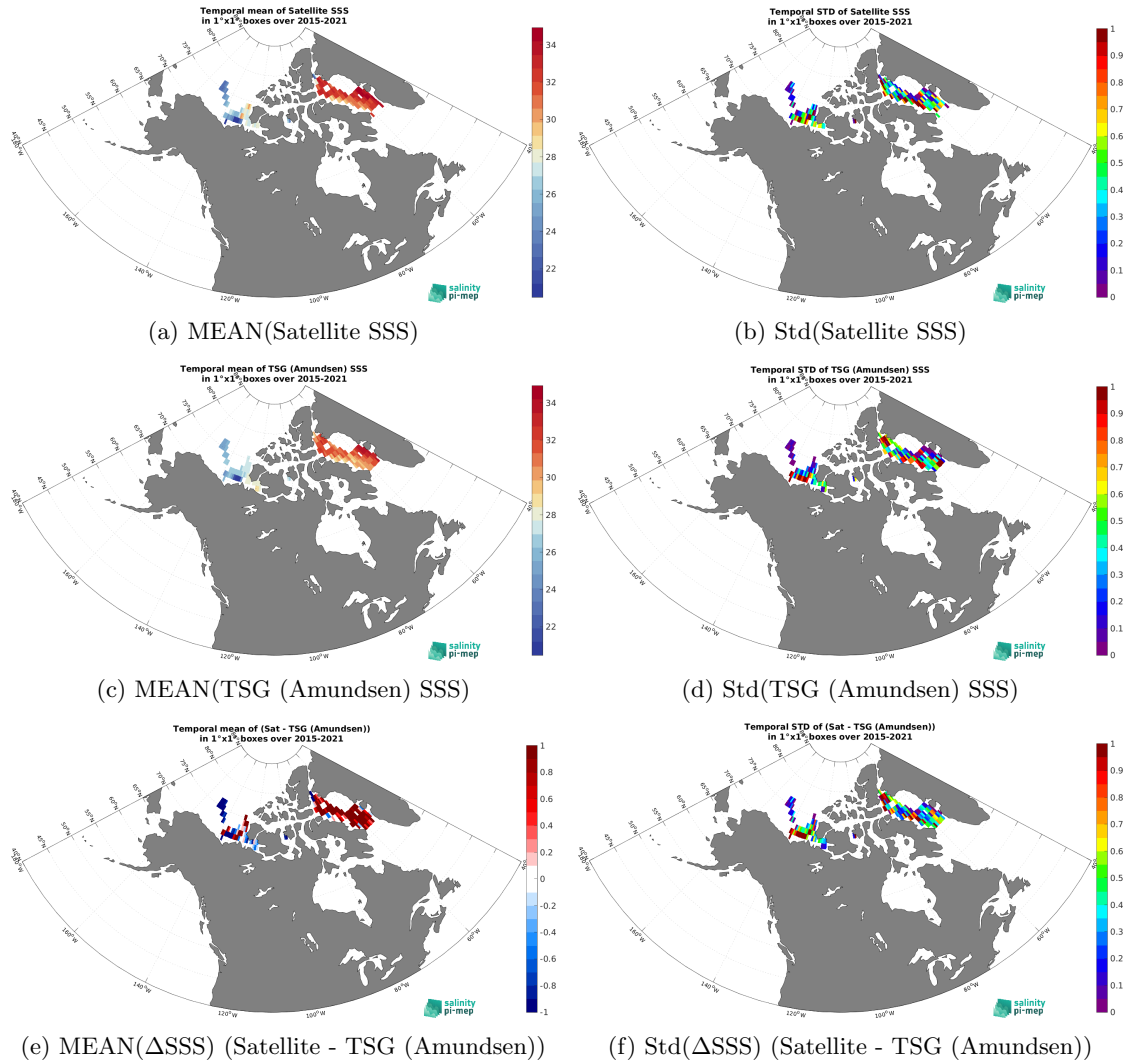
Figure 6: Temporal mean (left) and Std (right) of SSS from SMAP SSS L3 v5 - 8-Day running (RSS) (top), TSG (Amundsen) (middle), and of \Delta SSS (Satellite - TSG (Amundsen)). Only match-up pairs are used to generate these maps.
