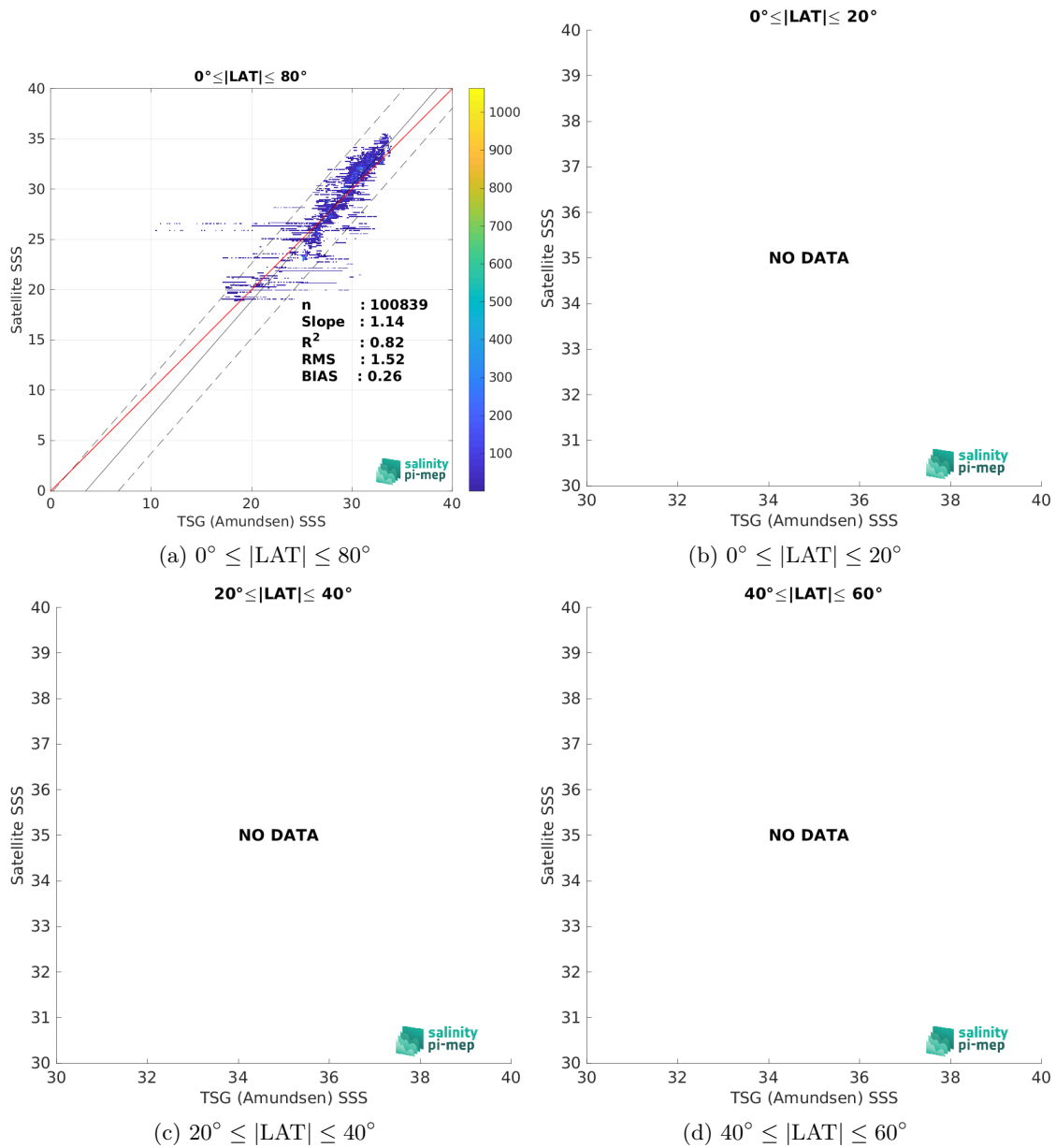
Figure 9: Contour maps of the concentration of SMAP SSS L3 v5 - 8-Day running (RSS) SSS (y-axis) versus TSG (Amundsen) SSS (x-axis) at match-up pairs for different latitude bands. For each plot, the red line shows x=y . The black thin and dashed lines indicate a linear fit through the data cloud and the \pm 95\% confidence levels, respectively. The number match-up pairs n , the slope and R^2 coefficient of the linear fit, the root mean square (RMS) and the mean bias between satellite and in situ data are indicated for each latitude band in each plots.
