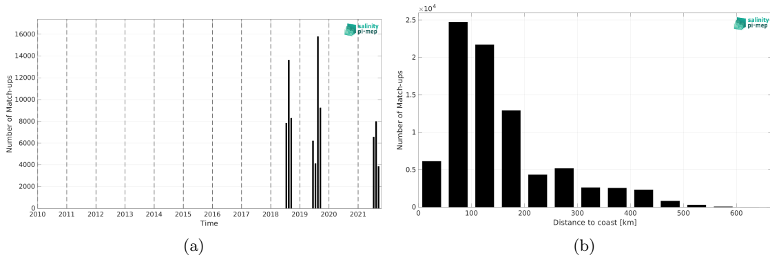
Figure 1: Number of match-ups between Saildrone and SMAP SSS L3 v5 - 8-Day running (RSS) SSS as a function of time (a) and as function of the distance to coast (b) over the Arctic Ocean Pi-MEP region and for the full satellite product period.
