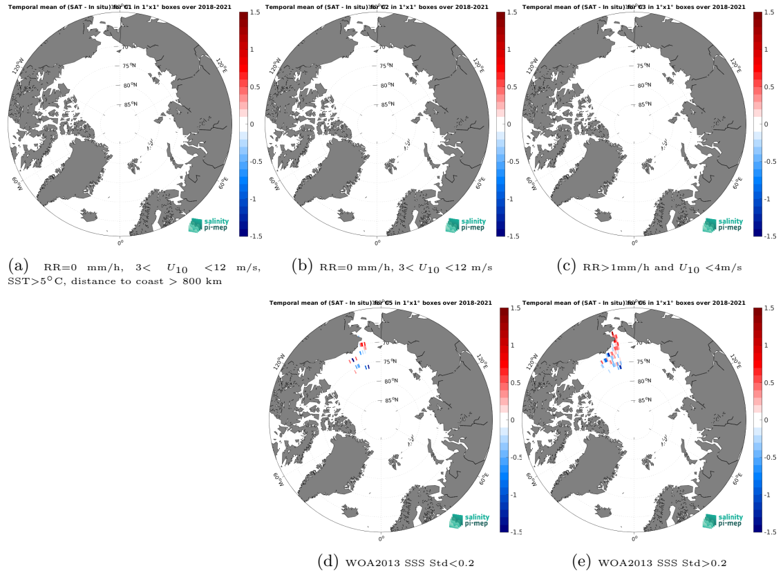
Figure 12: Temporal mean gridded over spatial boxes of size 1^{\circ}\times 1^{\circ} of \Delta\text{SSS} (SMAP SSS L3 v5 - 8-Day running (RSS) - Sairdrone) for 5 different subdatasets corresponding to:RR=0 mm/h, 3 < U_{10} < 12 m/s, SST >5^{\circ}\text{C} , distance to coast > 800 km (a), RR=0 mm/h, 3 < U_{10} < 12 m/s (b), RR >1 mm/h and U_{10} < 4 m/s (c), WOA2013 SSS Std <0.2 (d), WOA2013 SSS Std >0.2 (e).
