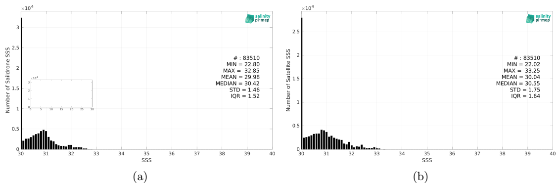
Figure 2: Histograms of SSS from Saildrone (a) and SMAP SSS L3 v5 - 8-Day running (RSS) (b) considering all match-up pairs per bins of 0.1 over the Arctic Ocean Pi-MEP region and for the full satellite product period.
