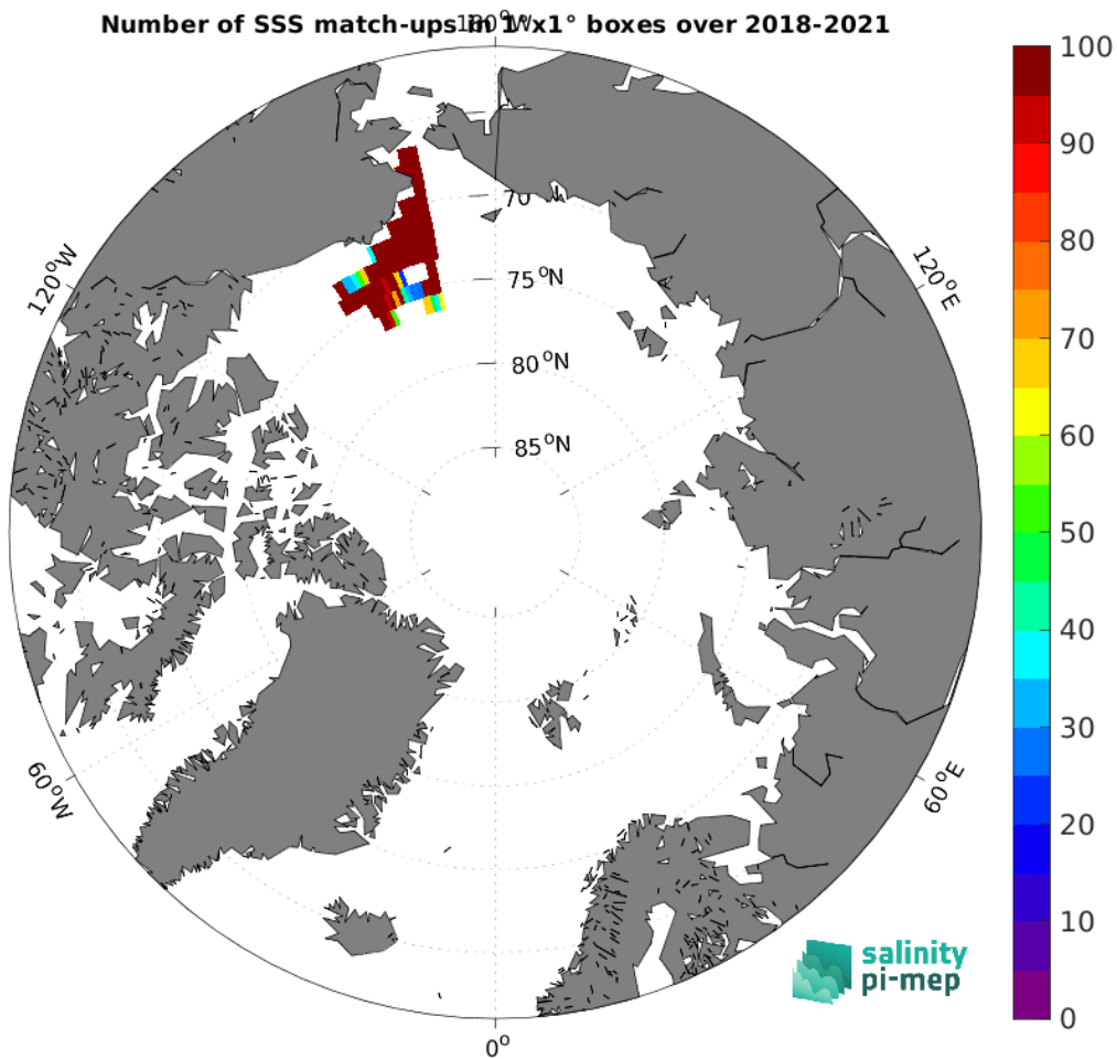
Figure 4: Number of SSS match-ups between Saildrone SSS and the SMAP SSS L3 v5 - 8-Day running (RSS) SSS product for the Arctic Ocean Pi-MEP region over 1^\circ \times 1^\circ boxes and for the full satellite product period.
