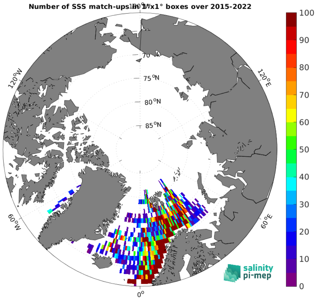
Figure 4: Number of SSS match-ups between ICES SSS and the SMAP SSS L3 v5 - 8-Day running (RSS) SSS product for the Arctic Ocean Pi-MEP region over 1^\circ \times 1^\circ boxes and for the full satellite product period.
