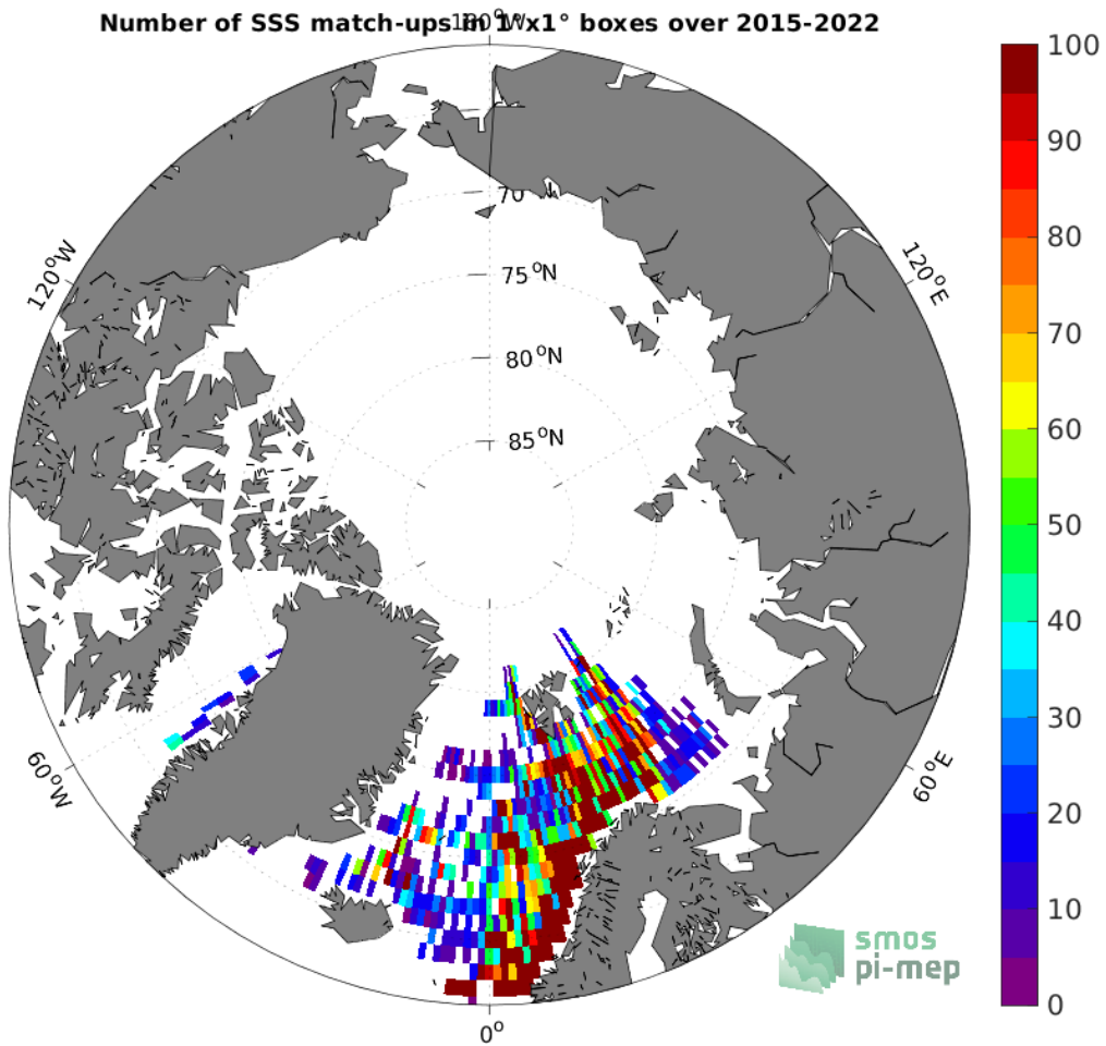
Figure 4: Number of SSS match-ups between ICES SSS and the SMAP SSS L3 v5 - 8-Day running (RSS) SSS product for the Arctic Ocean Pi-MEP region over 1^{\circ} \times 1^{\circ} boxes and for the full satellite product period.
