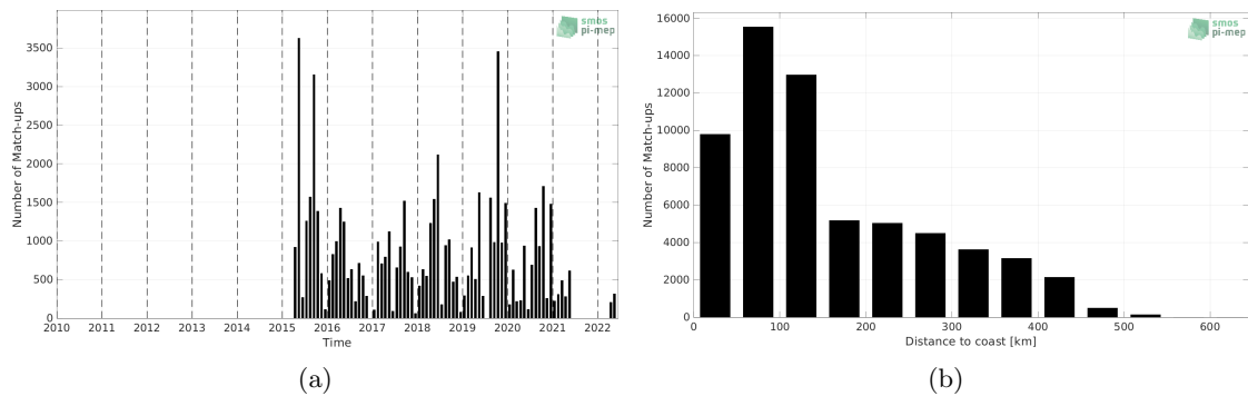
Figure 1: Number of match-ups between ICES and SMAP SSS L3 v5 - 8-Day running (RSS) SSS as a function of time (a) and as function of the distance to coast (b) over the Arctic Ocean Pi-MEP region and for the full satellite product period.
