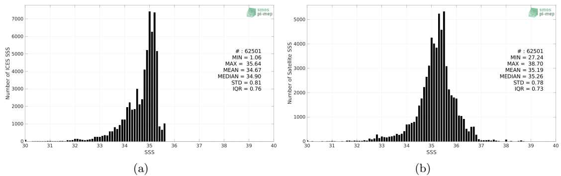
Figure 2: Histograms of SSS from ICES (a) and SMAP SSS L3 v5 - 8-Day running (RSS) (b) considering all match-up pairs per bins of 0.1 over the Arctic Ocean Pi-MEP region and for the full satellite product period.
