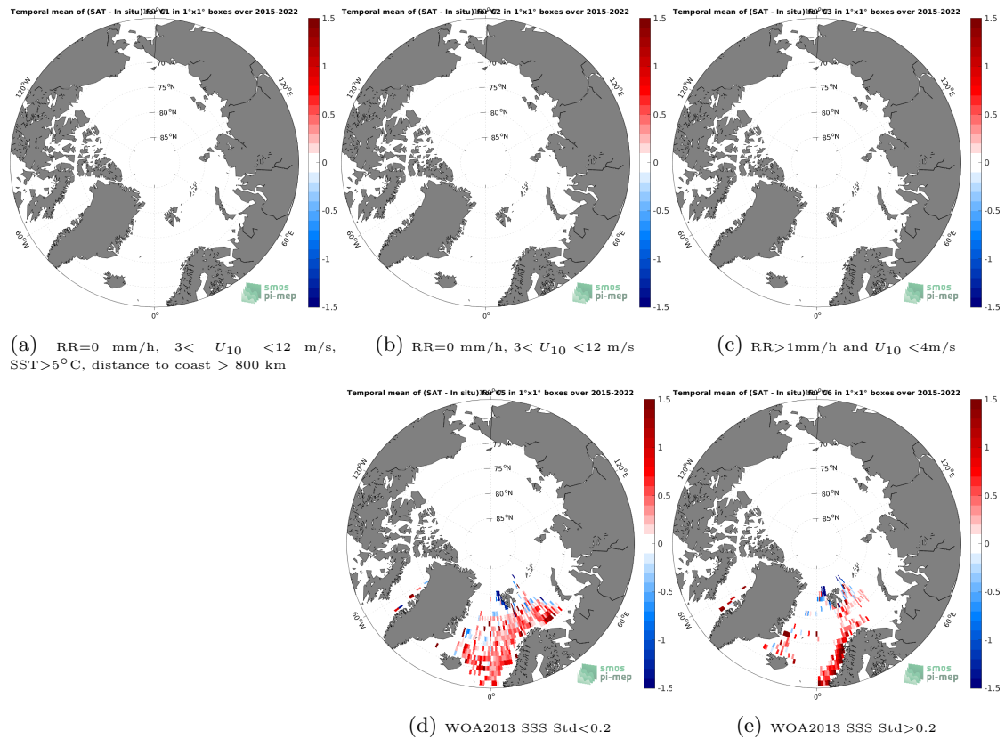
Figure 12: Temporal mean gridded over spatial boxes of size 1^{\circ}\times 1^{\circ} of \Delta\text{SSS} (SMAP SSS L3 v5 - 8-Day running (RSS) - ICES) for 5 different subdatasets corresponding to:RR=0 mm/h, 3 < U_{10} < 12 m/s, SST >5^{\circ}\text{C} , distance to coast > 800 km (a), RR=0 mm/h, 3 < U_{10} < 12 m/s (b), RR >1 mm/h and U_{10} < 4 m/s (c), WOA2013 SSS Std <0.2 (d), WOA2013 SSS Std >0.2 (e).
