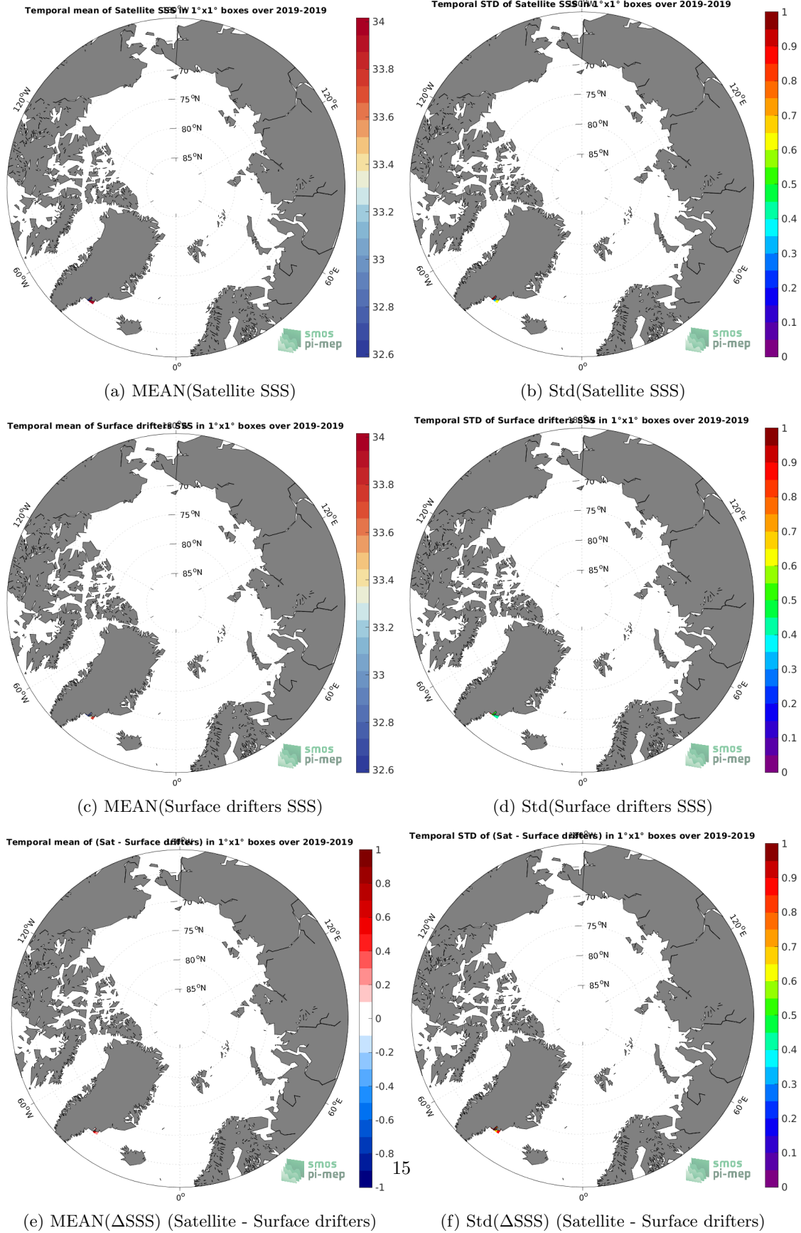
Figure 5: Temporal mean (left) and Std (right) of SSS from SMAP SSS L3 v5 - 8-Day running (RSS) (top), Surface drifters (middle), and of \Delta SSS (Satellite - Surface drifters). Only match-up pairs are used to generate these maps.
