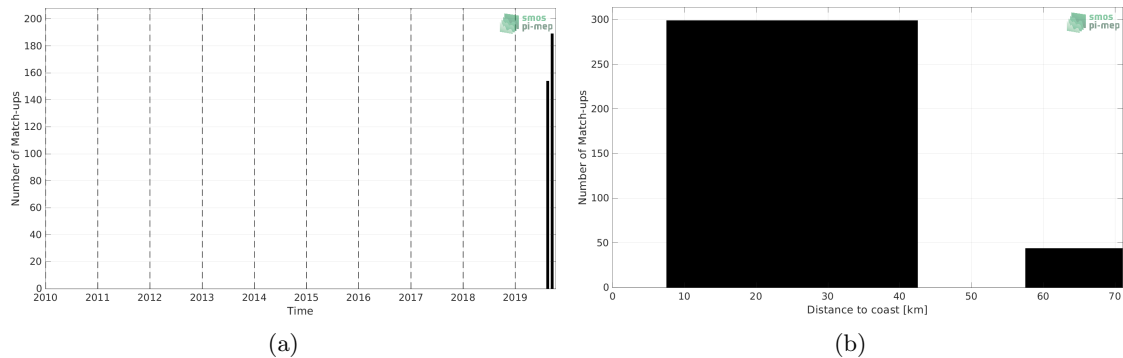
Figure 1: Number of match-ups between Surface drifters and SMAP SSS L3 v5 - 8-Day running (RSS) SSS as a function of time (a) and as function of the distance to coast (b) over the Arctic Ocean Pi-MEP region and for the full satellite product period.
