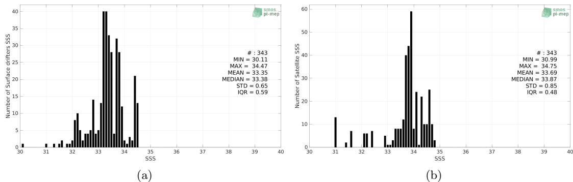
Figure 2: Histograms of SSS from Surface drifters (a) and SMAP SSS L3 v5 - 8-Day running (RSS) (b) considering all match-up pairs per bins of 0.1 over the Arctic Ocean Pi-MEP region and for the full satellite product period.
