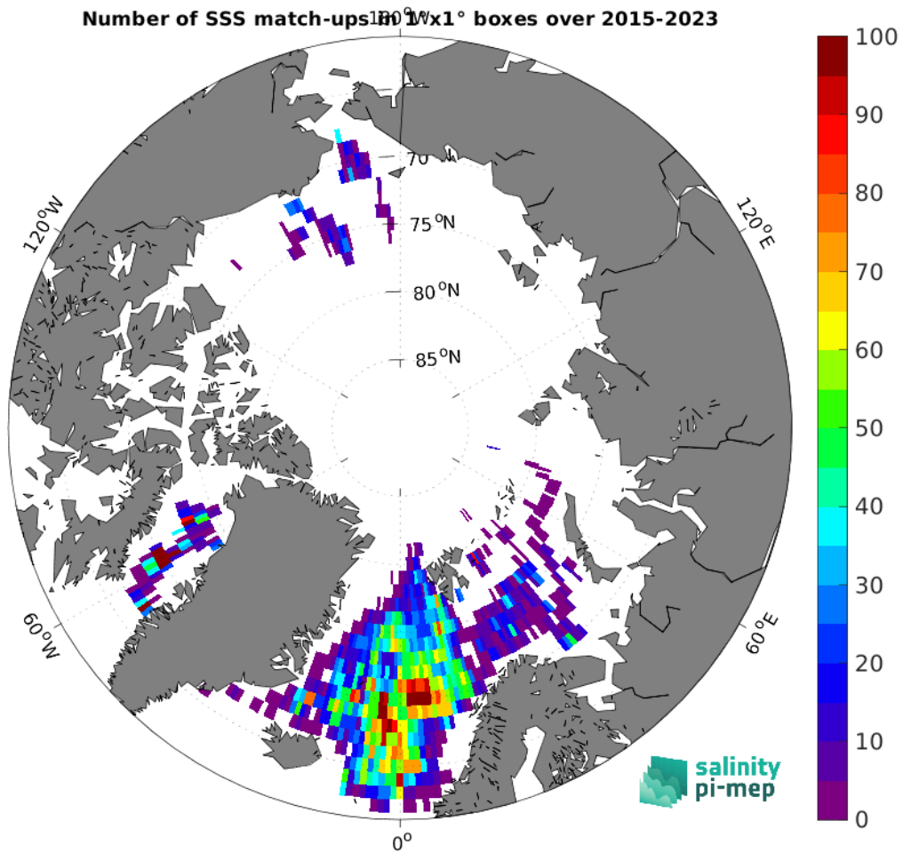
Figure 4: Number of SSS match-ups between Argo SSS and the SMAP SSS L3 v5 - 8-Day running (RSS) SSS product for the Arctic Ocean Pi-MEP region over 1^\circ \times 1^\circ boxes and for the full satellite product period.
