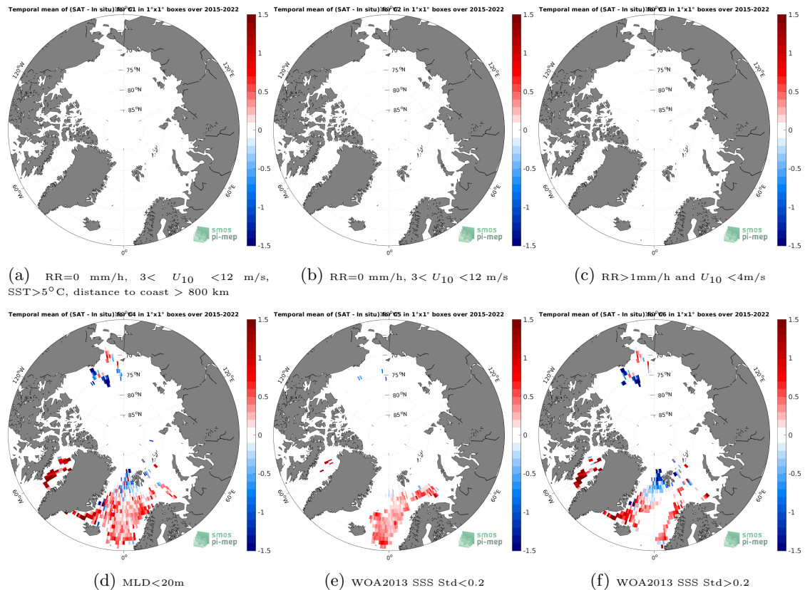
Figure 12: Temporal mean gridded over spatial boxes of size 1^{\circ}\times 1^{\circ} of \Delta\text{SSS} (SMAP SSS L3 v5 - 8-Day running (RSS) - Argo) for 6 different subdatasets corresponding to: \text{RR}=0 mm/h, 3 < U_{10} < 12 m/s, \text{SST} > 5^{\circ}\text{C} , distance to coast > 800 km (a), \text{RR}=0 mm/h, 3 < U_{10} < 12 m/s (b), \text{RR} > 1\text{mm/h} and U_{10} < 4\text{m/s} (c), \text{MLD} < 20\text{m} (d), WOA2013 SSS Std < 0.2 (e), WOA2013 SSS Std > 0.2 (f).
