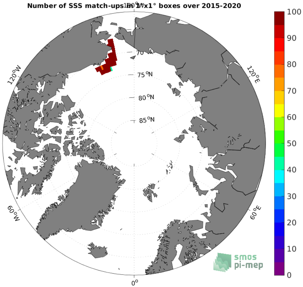
Figure 4: Number of SSS match-ups between TSG (SAMOS) SSS and the SMAP SSS L3 v5 - Monthly (RSS) SSS product for the Arctic Ocean Pi-MEP region over 1^\circ \times 1^\circ boxes and for the full satellite product period.
