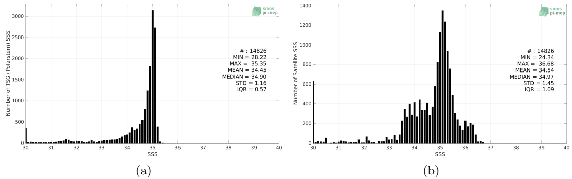
Figure 2: Histograms of SSS from TSG (Polarstern) (a) and SMAP SSS L3 v5 - Monthly (RSS) (b) considering all match-up pairs per bins of 0.1 over the Arctic Ocean Pi-MEP region and for the full satellite product period.
