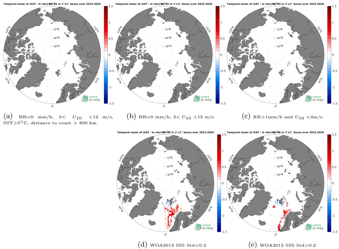
Figure 12: Temporal mean gridded over spatial boxes of size 1^{\circ}\times 1^{\circ} of \Delta\text{SSS} (SMAP SSS L3 v5 - Monthly (RSS) - TSG (Polarstern)) for 5 different subdatasets corresponding to: \text{RR}=0 mm/h, 3 < U_{10} < 12 m/s, \text{SST}>5^{\circ}\text{C} , distance to coast > 800 km (a), \text{RR}=0 mm/h, 3 < U_{10} < 12 m/s (b), \text{RR}>1 mm/h and U_{10} < 4 m/s (c), WOA2013 SSS Std <0.2 (d), WOA2013 SSS Std >0.2 (e).
