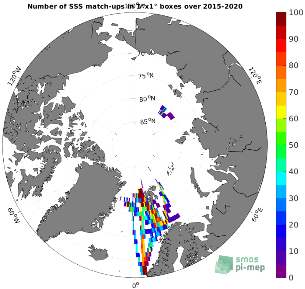
Figure 4: Number of SSS match-ups between TSG (Polarstern) SSS and the SMAP SSS L3 v5 - Monthly (RSS) SSS product for the Arctic Ocean Pi-MEP region over 1^\circ \times 1^\circ boxes and for the full satellite product period.
