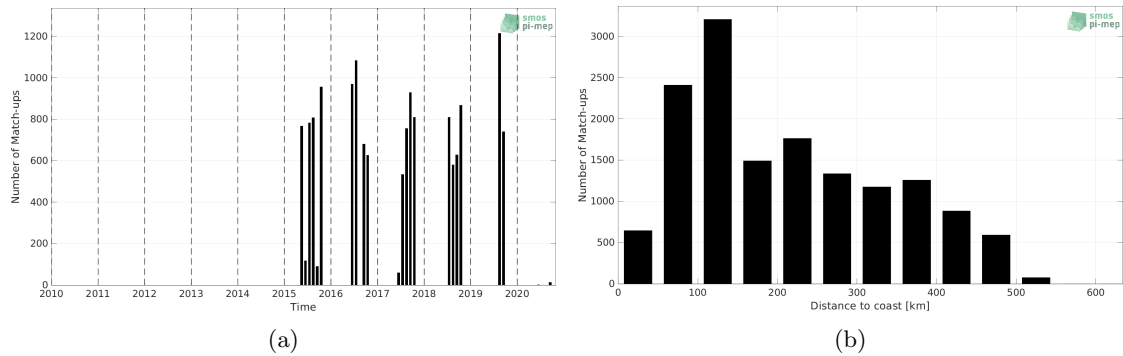
Figure 1: Number of match-ups between TSG (Polarstern) and SMAP SSS L3 v5 - Monthly (RSS) SSS as a function of time (a) and as function of the distance to coast (b) over the Arctic Ocean Pi-MEP region and for the full satellite product period.
