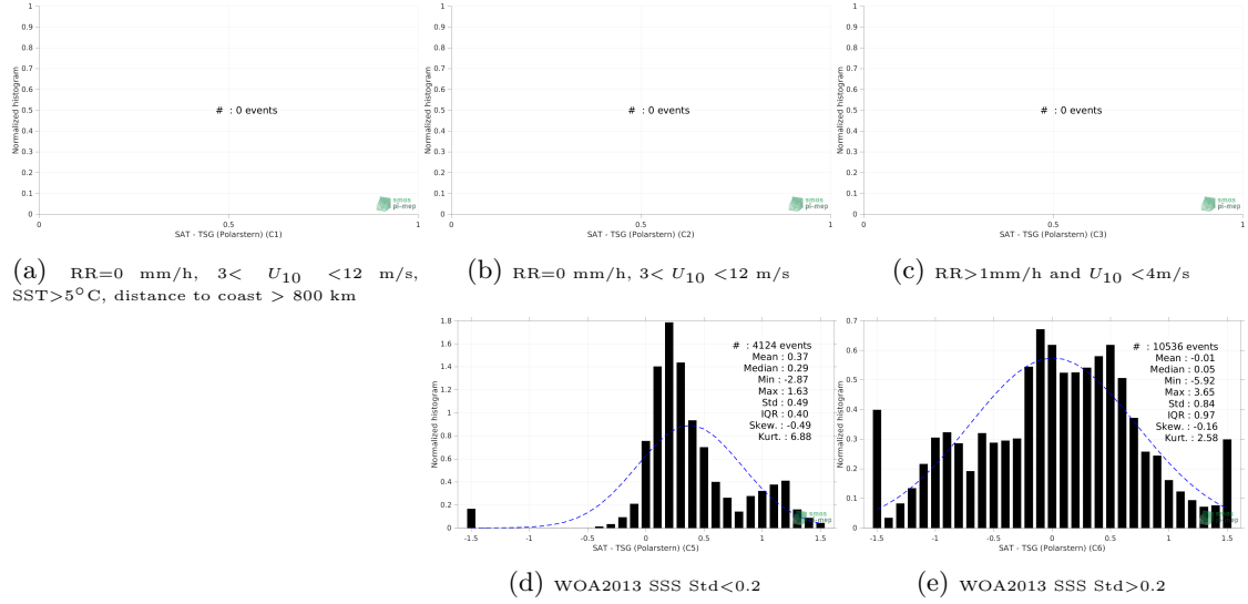
Figure 13: Normalized histogram of \Delta SSS (SMAP SSS L3 v5 - Monthly (RSS) - TSG (Polarstern)) for 5 different subdatasets corresponding to: RR=0 mm/h, 3 < U_{10} < 12 m/s, SST >5^{\circ}\text{C} , distance to coast > 800 km (a), RR=0 mm/h, 3 < U_{10} < 12 m/s (b), RR >1 mm/h and U_{10} < 4 m/s (c), WOA2013 SSS Std <0.2 (d), WOA2013 SSS Std >0.2 (e).
