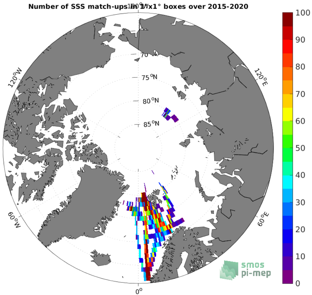
Figure 4: Number of SSS match-ups between TSG (Polarstern) SSS and the SMAP SSS L3 v5 - Monthly (RSS) SSS product for the Arctic Ocean Pi-MEP region over 1^{\circ} \times 1^{\circ} boxes and for the full satellite product period.
