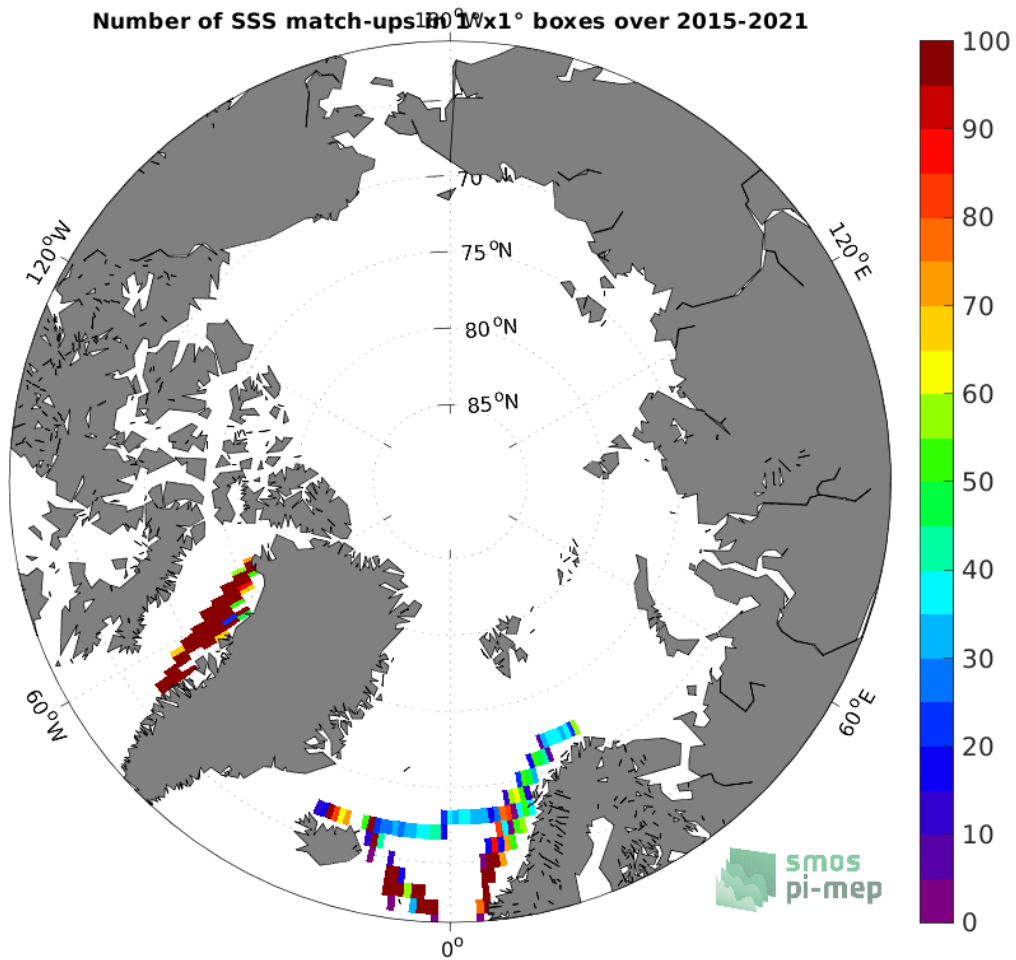
Figure 4: Number of SSS match-ups between TSG (LEGOS-DM) SSS and the SMAP SSS L3 v5 - Monthly (RSS) SSS product for the Arctic Ocean Pi-MEP region over 1^\circ \times 1^\circ boxes and for the full satellite product period.
