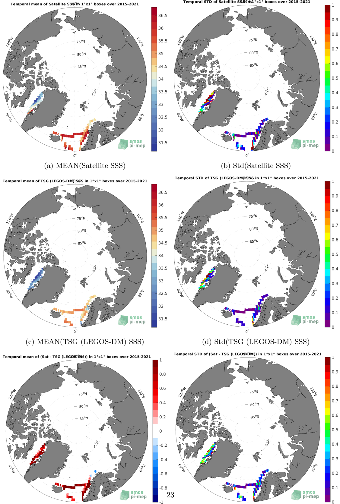
(e) MEAN( \Delta SSS) (Satellite - TSG (LEGOS-DM)) (f) Std( \Delta SSS) (Satellite - TSG (LEGOS-DM)) Figure 6: Temporal mean (left) and Std (right) of SSS from SMAP SSS L3 v5 - Monthly (RSS) (top), TSG (LEGOS-DM) (middle), and of \Delta SSS (Satellite - TSG (LEGOS-DM)). Only match-up pairs are used to generate these maps.
