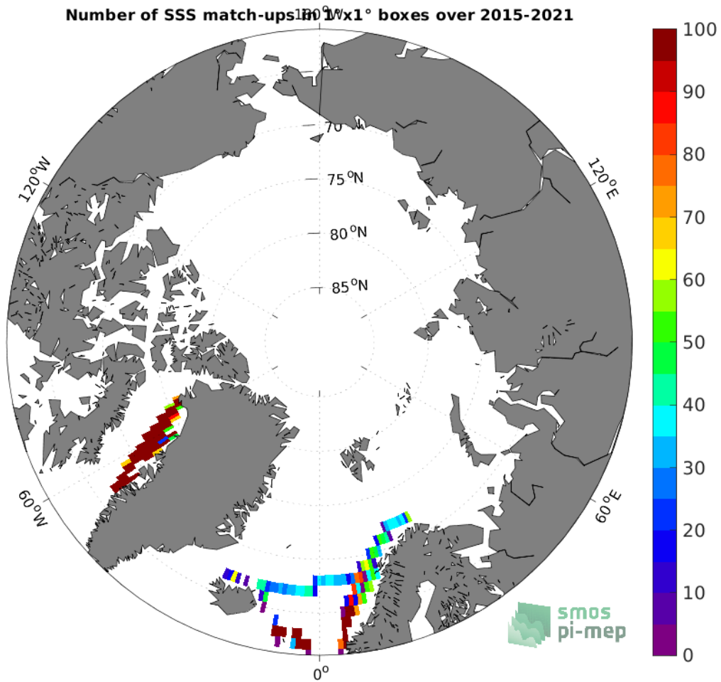
Figure 4: Number of SSS match-ups between TSG (LEGOS-DM) SSS and the SMAP SSS L3 v5 - Monthly (RSS) SSS product for the Arctic Ocean Pi-MEP region over 1^{\circ} \times 1^{\circ} boxes and for the full satellite product period.
