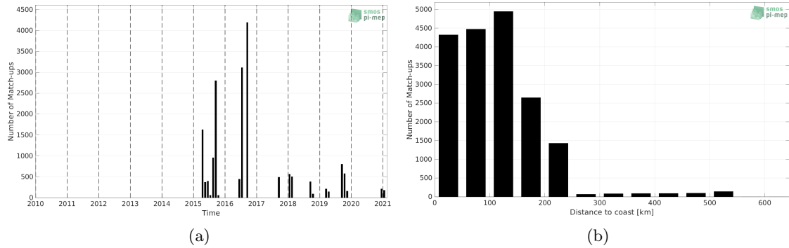
Figure 1: Number of match-ups between TSG (LEGOS-DM) and SMAP SSS L3 v5 - Monthly (RSS) SSS as a function of time (a) and as function of the distance to coast (b) over the Arctic Ocean Pi-MEP region and for the full satellite product period.
