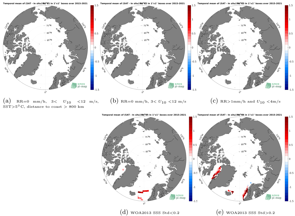
Figure 12: Temporal mean gridded over spatial boxes of size 1^{\circ}\times 1^{\circ} of \Delta\text{SSS} (SMAP SSS L3 v5 - Monthly (RSS) - TSG (LEGOS-DM)) for 5 different subdatasets corresponding to:RR=0 mm/h, 3 < U_{10} < 12 m/s, SST >5^{\circ}\text{C} , distance to coast > 800 km (a), RR=0 mm/h, 3 < U_{10} < 12 m/s (b), RR >1 mm/h and U_{10} < 4 m/s (c), WOA2013 SSS Std <0.2 (d), WOA2013 SSS Std >0.2 (e).
