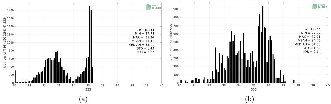
Figure 2: Histograms of SSS from TSG (LEGOS-DM) (a) and SMAP SSS L3 v5 - Monthly (RSS) (b) considering all match-up pairs per bins of 0.1 over the Arctic Ocean Pi-MEP region and for the full satellite product period.
