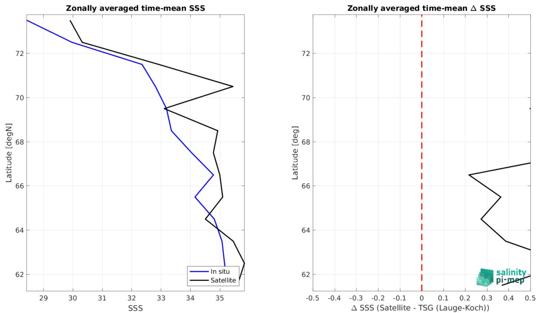
Figure 8: Left panel: Zonal mean SSS from SMAP SSS L3 v5 - Monthly (RSS) satellite product (black) and from TSG (Lauge-Koch) (blue). Right panel: Zonal mean of \Delta SSS (Satellite - TSG (Lauge-Koch)) for all the collected Pi-MEP match-up pairs estimated over the full satellite product period.
