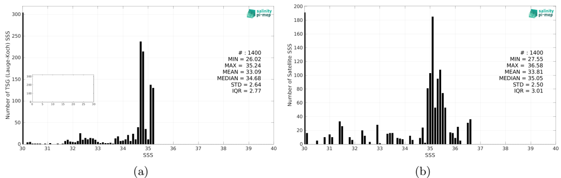
Figure 2: Histograms of SSS from TSG (Lauge-Koch) (a) and SMAP SSS L3 v5 - Monthly (RSS) (b) considering all match-up pairs per bins of 0.1 over the Arctic Ocean Pi-MEP region and for the full satellite product period.
