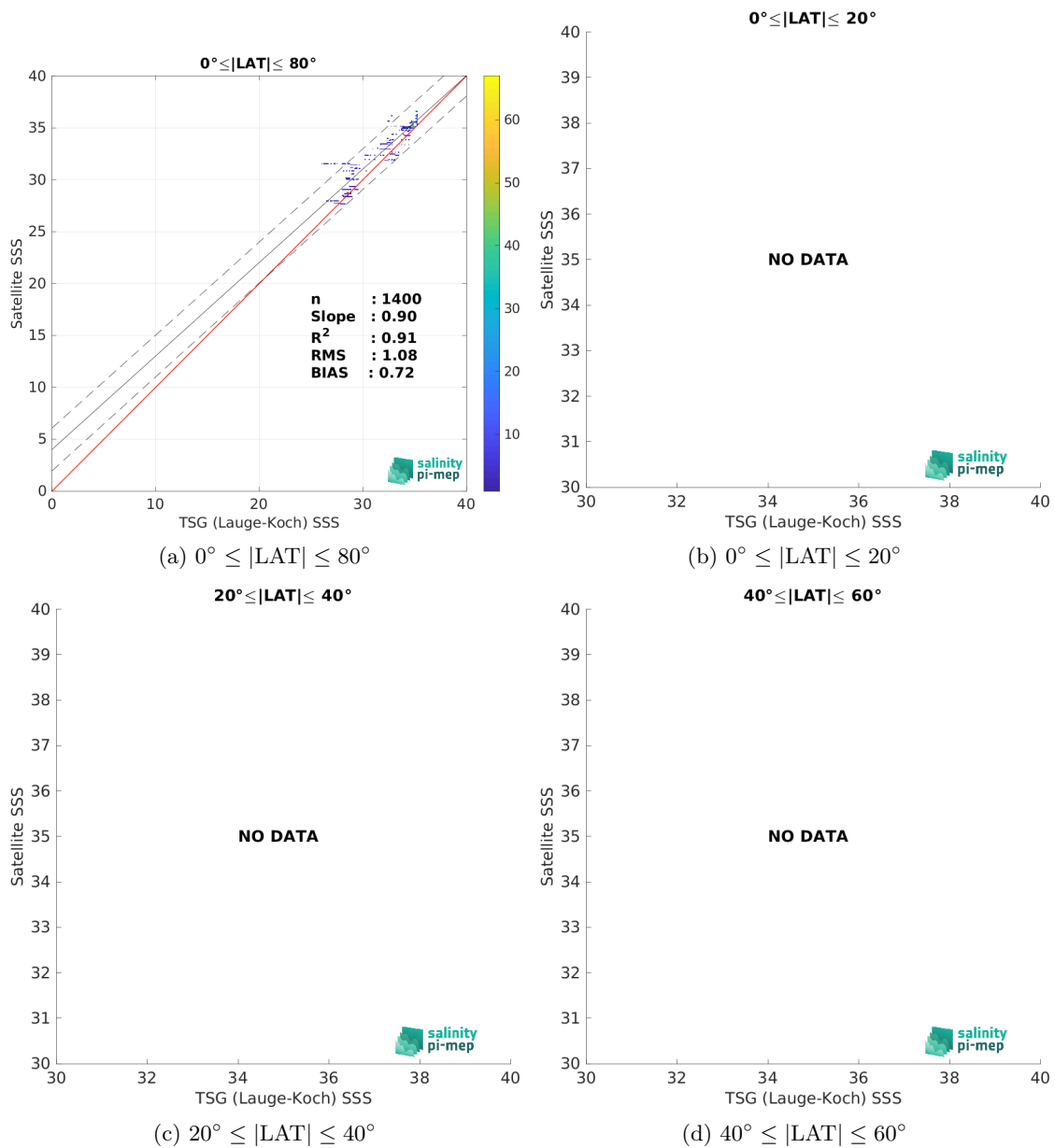
Figure 9: Contour maps of the concentration of SMAP SSS L3 v5 - Monthly (RSS) SSS (y-axis) versus TSG (Lauge-Koch) SSS (x-axis) at match-up pairs for different latitude bands. For each plot, the red line shows x=y . The black thin and dashed lines indicate a linear fit through the data cloud and the \pm 95\% confidence levels, respectively. The number match-up pairs n , the slope and R^2 coefficient of the linear fit, the root mean square (RMS) and the mean bias between satellite and in situ data are indicated for each latitude band in each plots.
