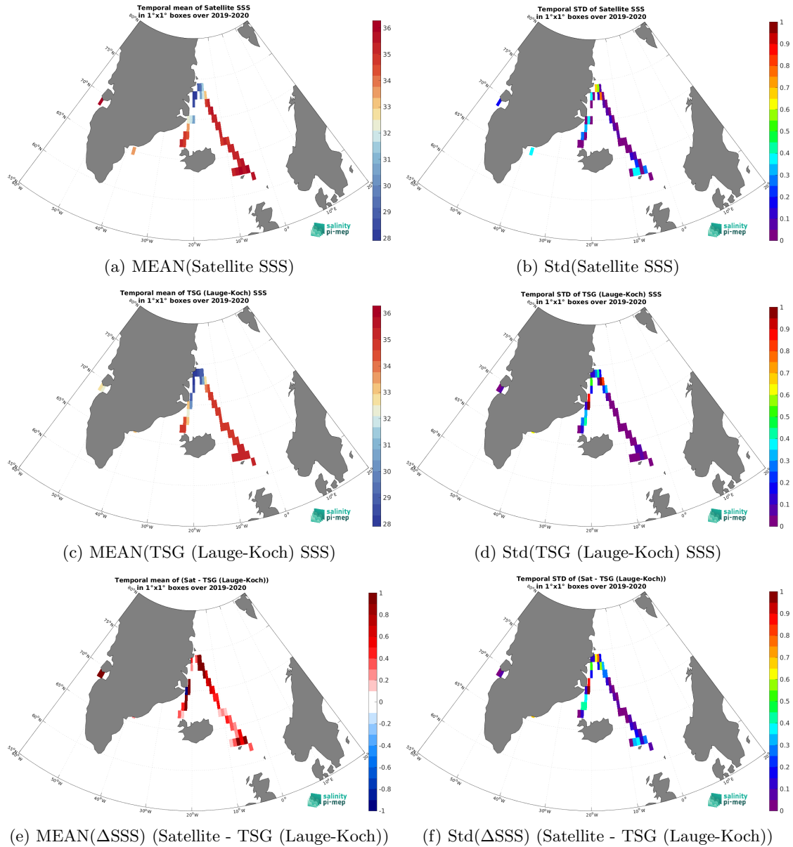
Figure 6: Temporal mean (left) and Std (right) of SSS from SMAP SSS L3 v5 - Monthly (RSS) (top), TSG (Lauge-Koch) (middle), and of \Delta SSS (Satellite - TSG (Lauge-Koch)). Only match-up pairs are used to generate these maps.
