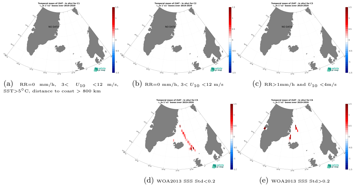
Figure 12: Temporal mean gridded over spatial boxes of size 1^{\circ}\times 1^{\circ} of \Delta\text{SSS} (SMAP SSS L3 v5 - Monthly (RSS) - TSG (Lauge-Koch)) for 5 different subdatasets corresponding to:RR=0 mm/h, 3 < U_{10} < 12 m/s, SST >5^{\circ}\text{C} , distance to coast > 800 km (a), RR=0 mm/h, 3 < U_{10} < 12 m/s (b), RR >1 mm/h and U_{10} < 4 m/s (c), WOA2013 SSS Std <0.2 (d), WOA2013 SSS Std >0.2 (e).
