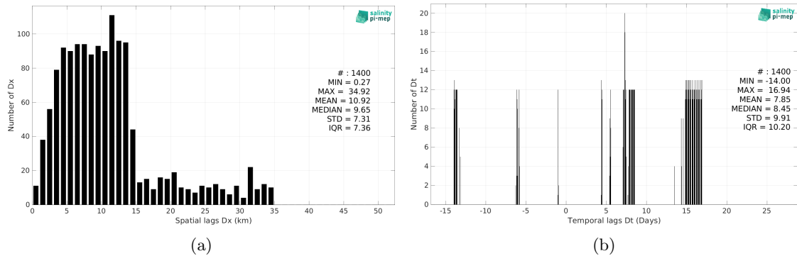
Figure 5: Histograms of the spatial (a) and temporal (b) lags between the location/time of the TSG (Lauge-Koch) measurement and the date of the corresponding SMAP SSS L3 v5 - Monthly (RSS) SSS pixel.
