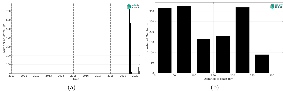
Figure 1: Number of match-ups between TSG (Lauge-Koch) and SMAP SSS L3 v5 - Monthly (RSS) SSS as a function of time (a) and as function of the distance to coast (b) over the Arctic Ocean Pi-MEP region and for the full satellite product period.
