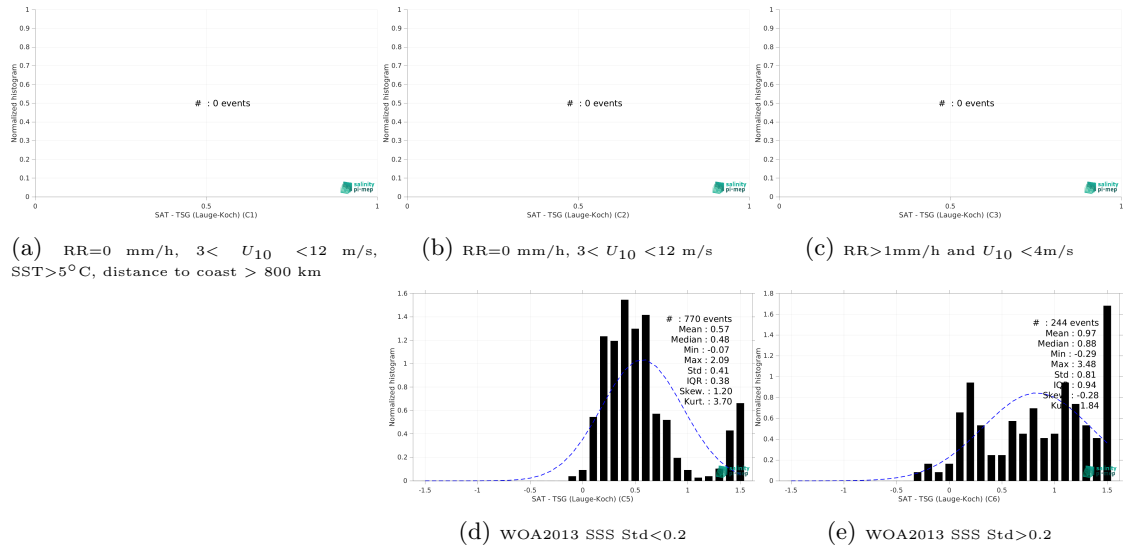
Figure 13: Normalized histogram of \Delta SSS (SMAP SSS L3 v5 - Monthly (RSS) - TSG (Lauge-Koch)) for 5 different subdatasets corresponding to: RR=0 mm/h, 3 < U_{10} < 12 m/s, SST > 5°C, distance to coast > 800 km (a), RR=0 mm/h, 3 < U_{10} < 12 m/s (b), RR > 1mm/h and U_{10} < 4 m/s (c), WOA2013 SSS Std < 0.2 (d), WOA2013 SSS Std > 0.2 (e).
