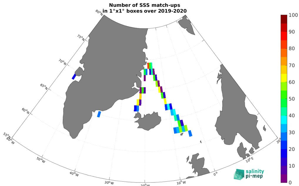
Figure 4: Number of SSS match-ups between TSG (Lauge-Koch) SSS and the SMAP SSS L3 v5 - Monthly (RSS) SSS product for the Arctic Ocean Pi-MEP region over 1^\circ \times 1^\circ boxes and for the full satellite product period.
