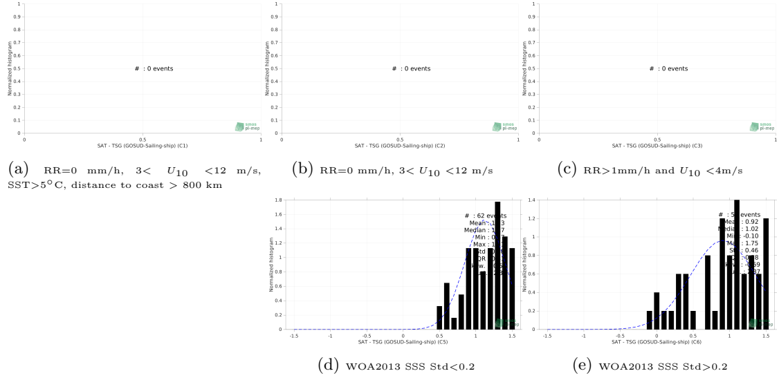
Figure 13: Normalized histogram of \Delta SSS (SMAP SSS L3 v5 - Monthly (RSS) - TSG (GOSUD-Sailing-ship)) for 5 different subdatasets corresponding to: RR=0 mm/h, 3 < U_{10} < 12 m/s, SST >5^{\circ}\text{C} , distance to coast > 800 km (a), RR=0 mm/h, 3 < U_{10} < 12 m/s (b), RR >1 mm/h and U_{10} < 4 m/s (c), WOA2013 SSS Std <0.2 (d), WOA2013 SSS Std >0.2 (e).
