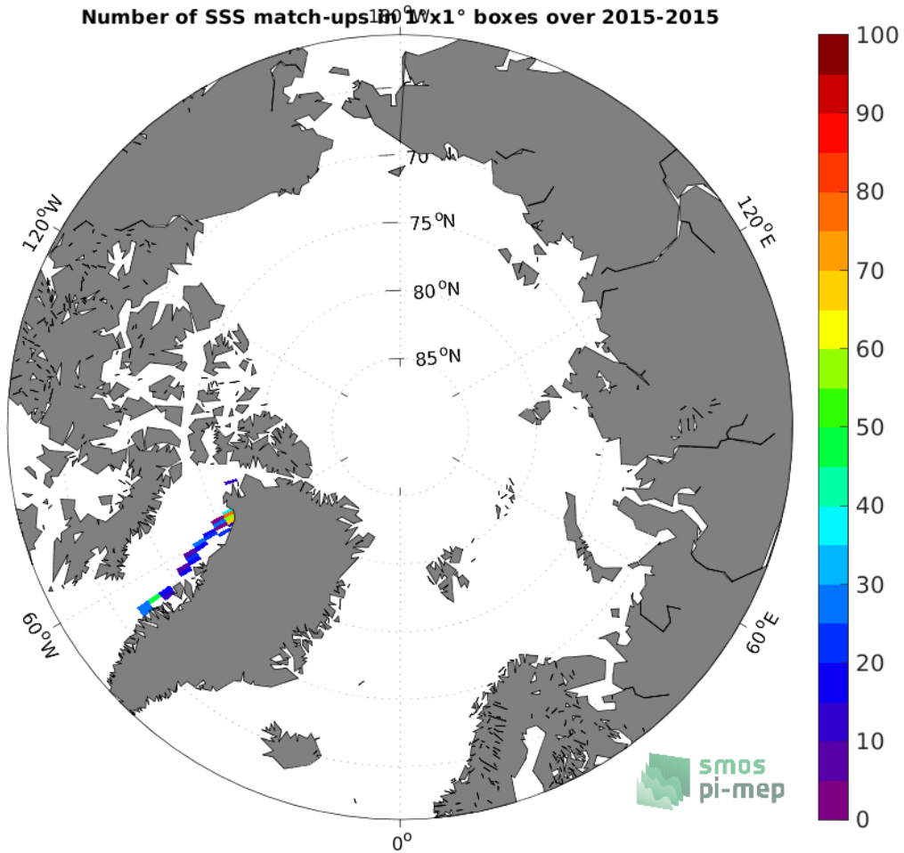
Figure 4: Number of SSS match-ups between TSG (GOSUD-Sailing-ship) SSS and the SMAP SSS L3 v5 - Monthly (RSS) SSS product for the Arctic Ocean Pi-MEP region over 1^\circ \times 1^\circ boxes and for the full satellite product period.
