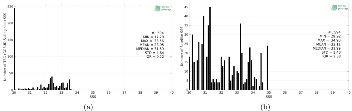
Figure 2: Histograms of SSS from TSG (GOSUD-Sailing-ship) (a) and SMAP SSS L3 v5 - Monthly (RSS) (b) considering all match-up pairs per bins of 0.1 over the Arctic Ocean Pi-MEP region and for the full satellite product period.
