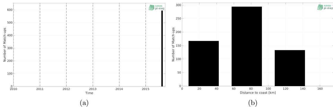
Figure 1: Number of match-ups between TSG (GOSUD-Sailing-ship) and SMAP SSS L3 v5 - Monthly (RSS) SSS as a function of time (a) and as function of the distance to coast (b) over the Arctic Ocean Pi-MEP region and for the full satellite product period.
