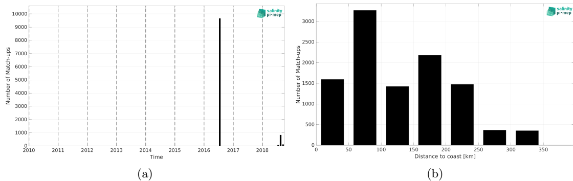
Figure 1: Number of match-ups between TSG (GOSUD-Research-vessel) and SMAP SSS L3 v5 - Monthly (RSS) SSS as a function of time (a) and as function of the distance to coast (b) over the Arctic Ocean Pi-MEP region and for the full satellite product period.
