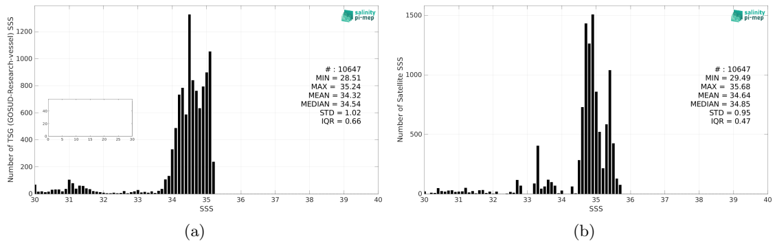
Figure 2: Histograms of SSS from TSG (GOSUD-Research-vessel) (a) and SMAP SSS L3 v5 - Monthly (RSS) (b) considering all match-up pairs per bins of 0.1 over the Arctic Ocean Pi-MEP region and for the full satellite product period.
