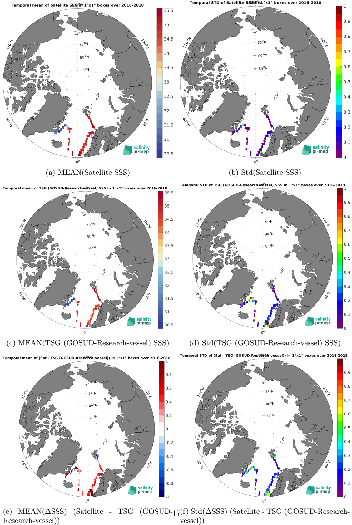
Figure 6: Temporal mean (left) and Std (right) of SSS from SMAP SSS L3 v5 - Monthly (RSS) (top), TSG (GOSUD-Research-vessel) (middle), and of \Delta SSS (Satellite - TSG (GOSUD-Research-vessel)). Only match-up pairs are used to generate these maps.
