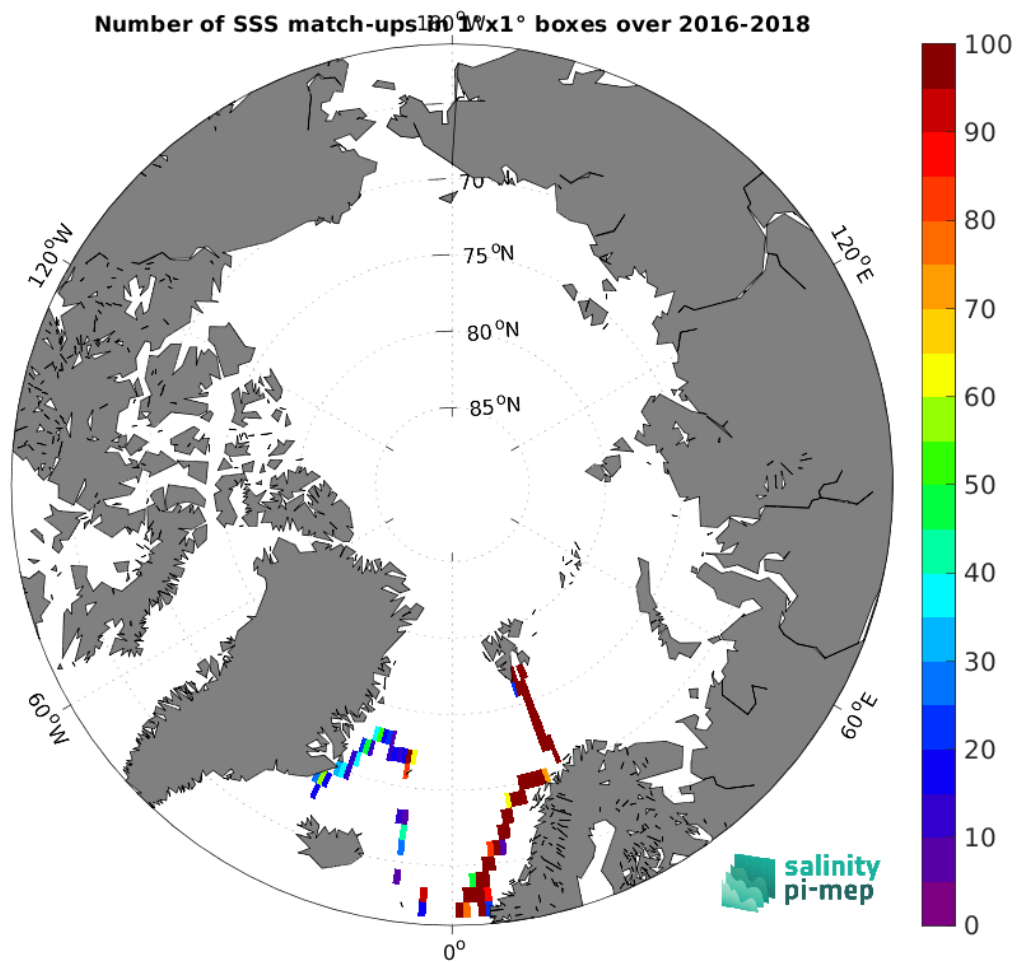
Figure 4: Number of SSS match-ups between TSG (GOSUD-Research-vessel) SSS and the SMAP SSS L3 v5 - Monthly (RSS) SSS product for the Arctic Ocean Pi-MEP region over 1^\circ \times 1^\circ boxes and for the full satellite product period.
