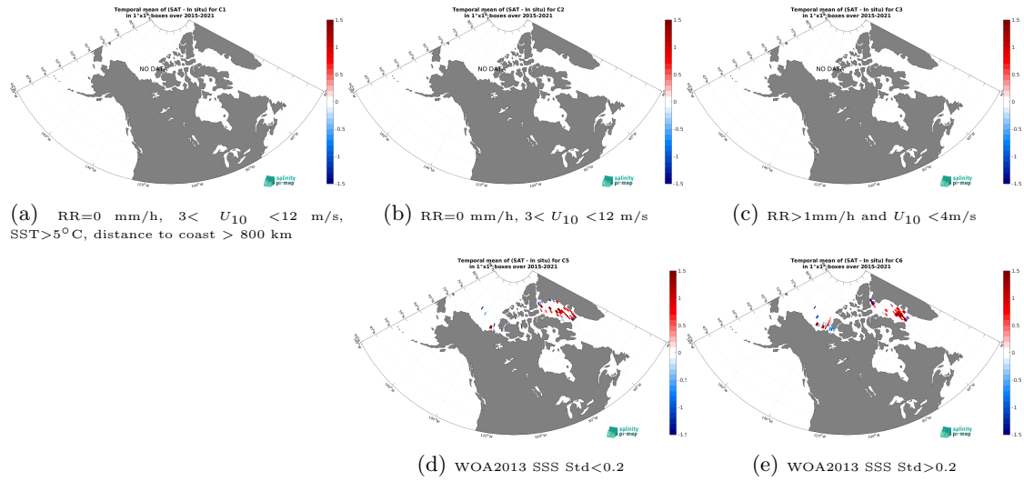
Figure 12: Temporal mean gridded over spatial boxes of size 1^{\circ}\times 1^{\circ} of \Delta\text{SSS} (SMAP SSS L3 v5 - Monthly (RSS) - TSG (Amundsen)) for 5 different subdatasets corresponding to:RR=0 mm/h, 3 < U_{10} < 12 m/s, SST > 5^{\circ}\text{C} , distance to coast > 800 km (a), RR=0 mm/h, 3 < U_{10} < 12 m/s (b), RR > 1 mm/h and U_{10} < 4 m/s (c), WOA2013 SSS Std < 0.2 (d), WOA2013 SSS Std > 0.2 (e).
