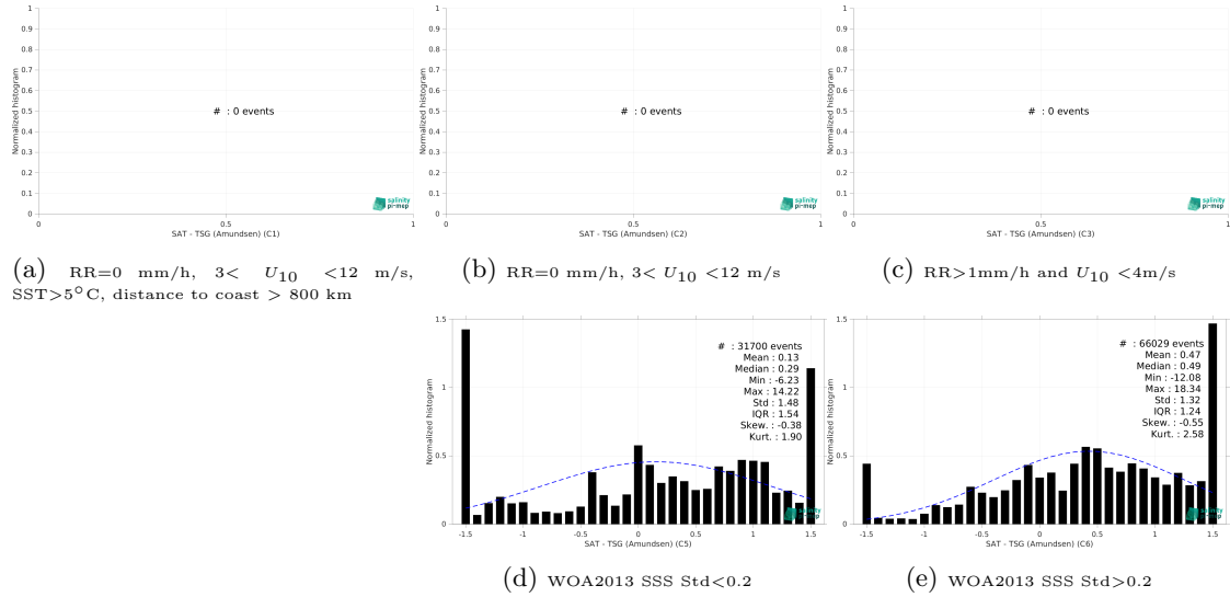
Figure 13: Normalized histogram of \Delta SSS (SMAP SSS L3 v5 - Monthly (RSS) - TSG (Amundsen)) for 5 different subdatasets corresponding to: RR=0 mm/h, 3 < U_{10} < 12 m/s, SST>5°C, distance to coast > 800 km (a), RR=0 mm/h, 3 < U_{10} < 12 m/s (b), RR>1mm/h and U_{10} < 4 m/s (c), WOA2013 SSS Std<0.2 (d), WOA2013 SSS Std>0.2 (e).
