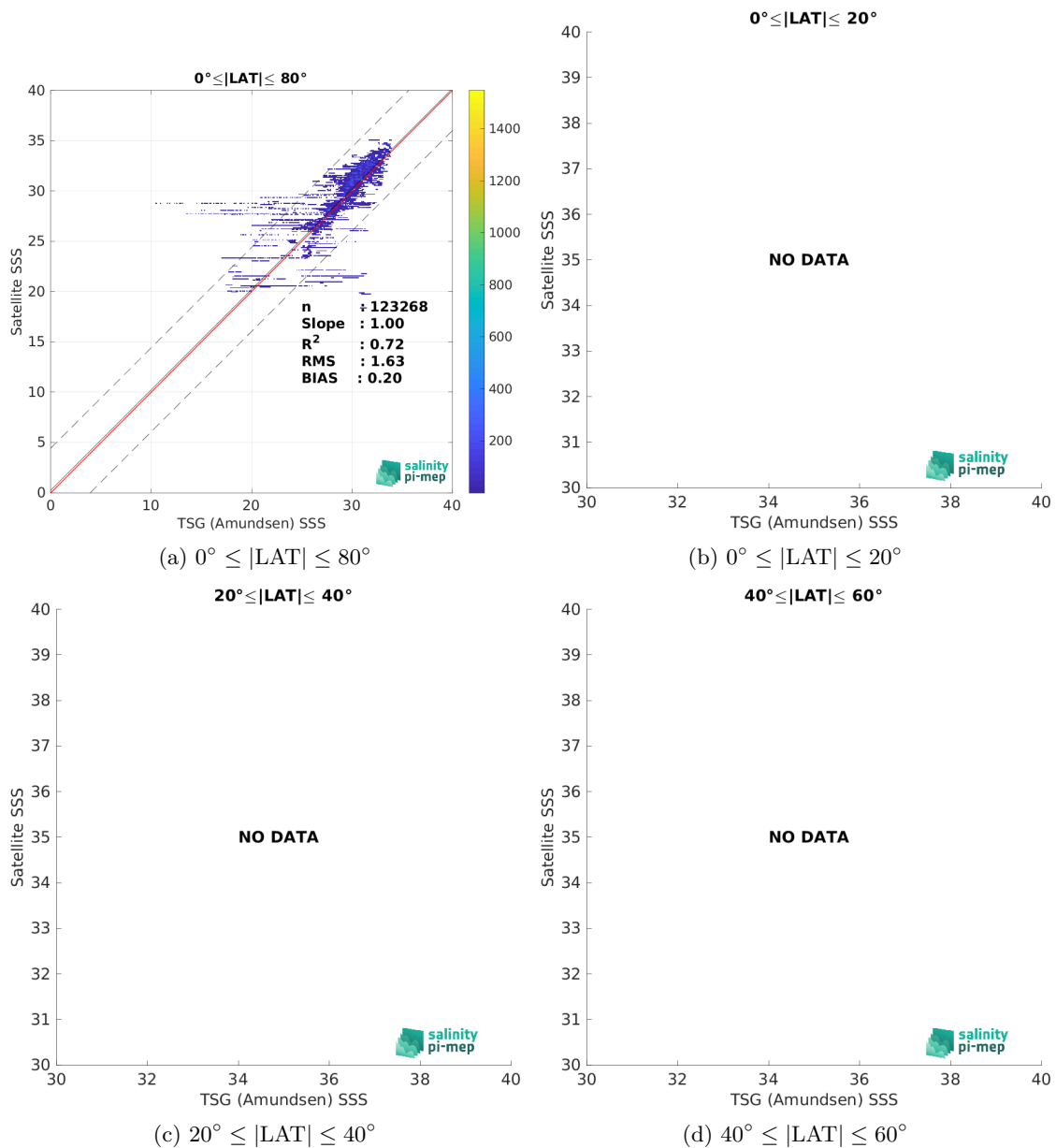
Figure 9: Contour maps of the concentration of SMAP SSS L3 v5 - Monthly (RSS) SSS (y-axis) versus TSG (Amundsen) SSS (x-axis) at match-up pairs for different latitude bands. For each plot, the red line shows x=y . The black thin and dashed lines indicate a linear fit through the data cloud and the \pm 95\% confidence levels, respectively. The number match-up pairs n , the slope and R^2 coefficient of the linear fit, the root mean square (RMS) and the mean bias between satellite and in situ data are indicated for each latitude band in each plots.
