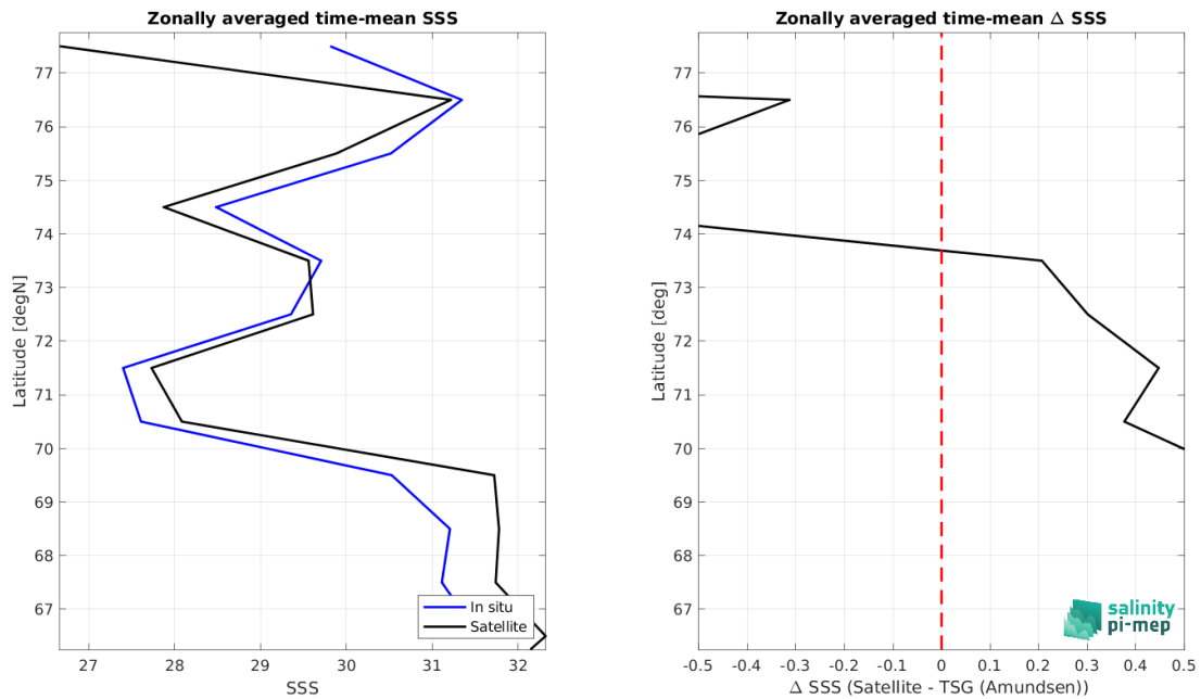
Figure 8: Left panel: Zonal mean SSS from SMAP SSS L3 v5 - Monthly (RSS) satellite product (black) and from TSG (Amundsen) (blue). Right panel: Zonal mean of \Delta SSS (Satellite - TSG (Amundsen)) for all the collected Pi-MEP match-up pairs estimated over the full satellite product period.
