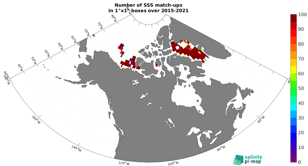
Figure 4: Number of SSS match-ups between TSG (Amundsen) SSS and the SMAP SSS L3 v5 - Monthly (RSS) SSS product for the Arctic Ocean Pi-MEP region over 1°×1° boxes and for the full satellite product period.
