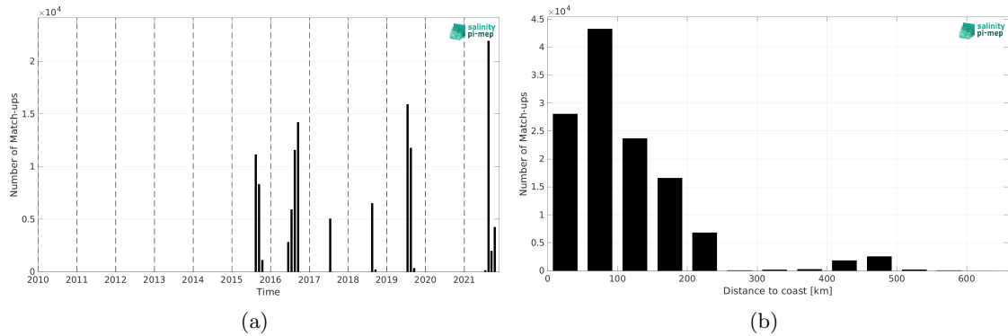
Figure 1: Number of match-ups between TSG (Amundsen) and SMAP SSS L3 v5 - Monthly (RSS) SSS as a function of time (a) and as function of the distance to coast (b) over the Arctic Ocean Pi-MEP region and for the full satellite product period.
