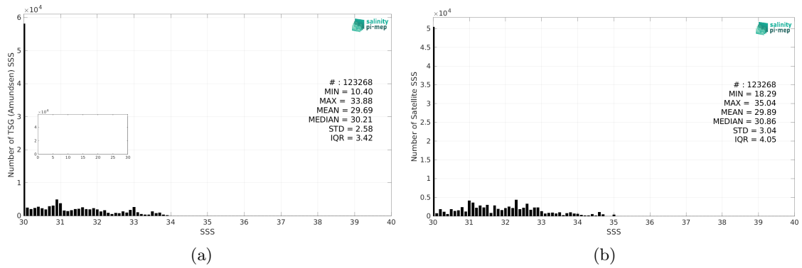
Figure 2: Histograms of SSS from TSG (Amundsen) (a) and SMAP SSS L3 v5 - Monthly (RSS) (b) considering all match-up pairs per bins of 0.1 over the Arctic Ocean Pi-MEP region and for the full satellite product period.
