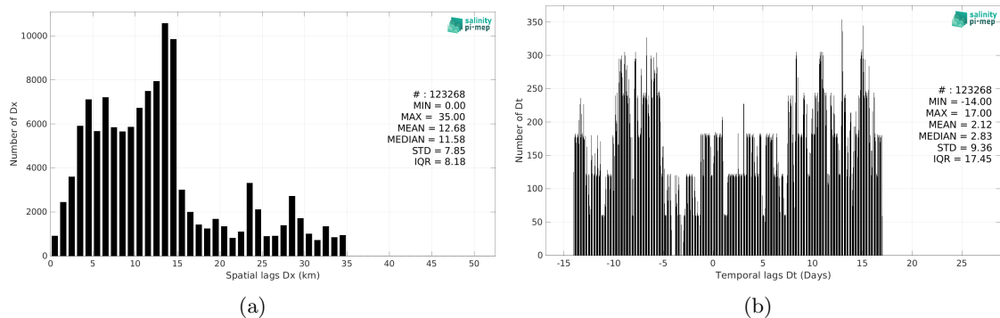
Figure 5: Histograms of the spatial (a) and temporal (b) lags between the location/time of the TSG (Amundsen) measurement and the date of the corresponding SMAP SSS L3 v5 - Monthly (RSS) SSS pixel.
