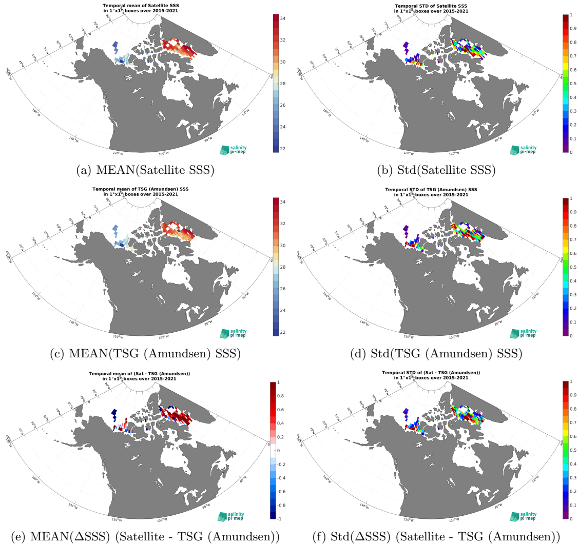
Figure 6: Temporal mean (left) and Std (right) of SSS from SMAP SSS L3 v5 - Monthly (RSS) (top), TSG (Amundsen) (middle), and of \Delta SSS (Satellite - TSG (Amundsen)). Only match-up pairs are used to generate these maps.
