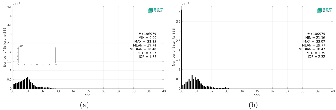
Figure 2: Histograms of SSS from Saildrone (a) and SMAP SSS L3 v5 - Monthly (RSS) (b) considering all match-up pairs per bins of 0.1 over the Arctic Ocean Pi-MEP region and for the full satellite product period.
