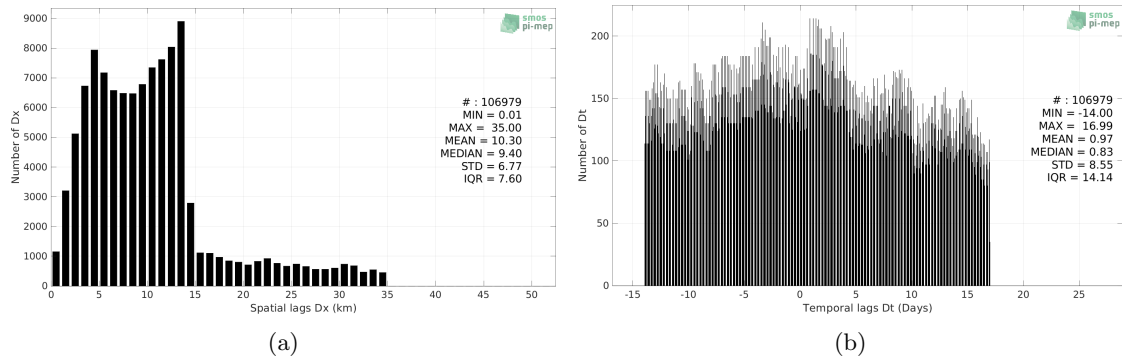
Figure 5: Histograms of the spatial (a) and temporal (b) lags between the location/time of the Sairdrone measurement and the date of the corresponding SMAP SSS L3 v5 - Monthly (RSS) SSS pixel.
