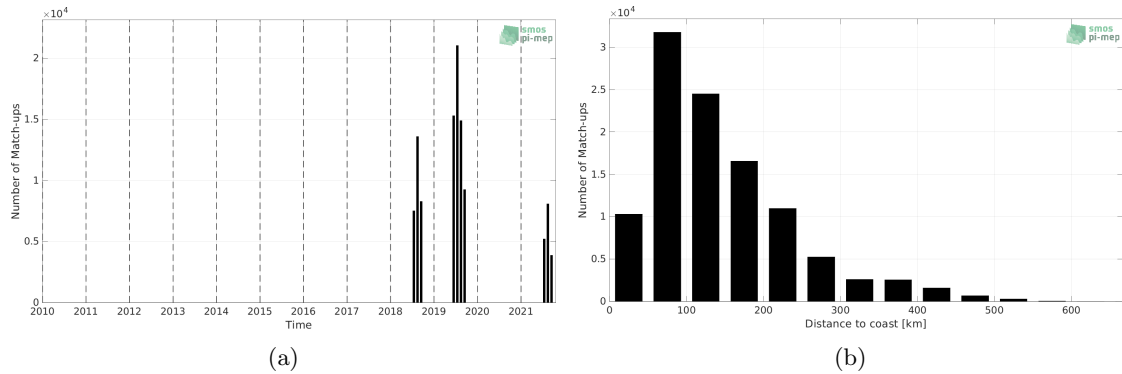
Figure 1: Number of match-ups between Saildrone and SMAP SSS L3 v5 - Monthly (RSS) SSS as a function of time (a) and as function of the distance to coast (b) over the Arctic Ocean Pi-MEP region and for the full satellite product period.
