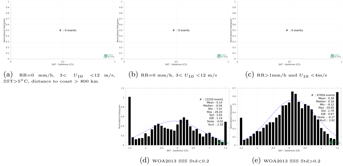
Figure 13: Normalized histogram of \Delta SSS (SMAP SSS L3 v5 - Monthly (RSS) - Saildrone) for 5 different subdatasets corresponding to: RR=0 mm/h, 3 < U_{10} < 12 m/s, SST>5°C, distance to coast > 800 km (a), RR=0 mm/h, 3 < U_{10} < 12 m/s (b), RR>1mm/h and U_{10} < 4 m/s (c), WOA2013 SSS Std<0.2 (d), WOA2013 SSS Std>0.2 (e).
