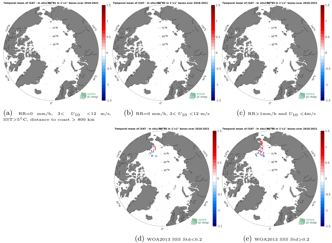
Figure 12: Temporal mean gridded over spatial boxes of size 1^{\circ}\times 1^{\circ} of \Delta\text{SSS} (SMAP SSS L3 v5 - Monthly (RSS) - Saildrone) for 5 different subdatasets corresponding to:RR=0 mm/h, 3 < U_{10} < 12 m/s, SST > 5^{\circ}\text{C} , distance to coast > 800 km (a), RR=0 mm/h, 3 < U_{10} < 12 m/s (b), RR > 1 mm/h and U_{10} < 4 m/s (c), WOA2013 SSS Std < 0.2 (d), WOA2013 SSS Std > 0.2 (e).
