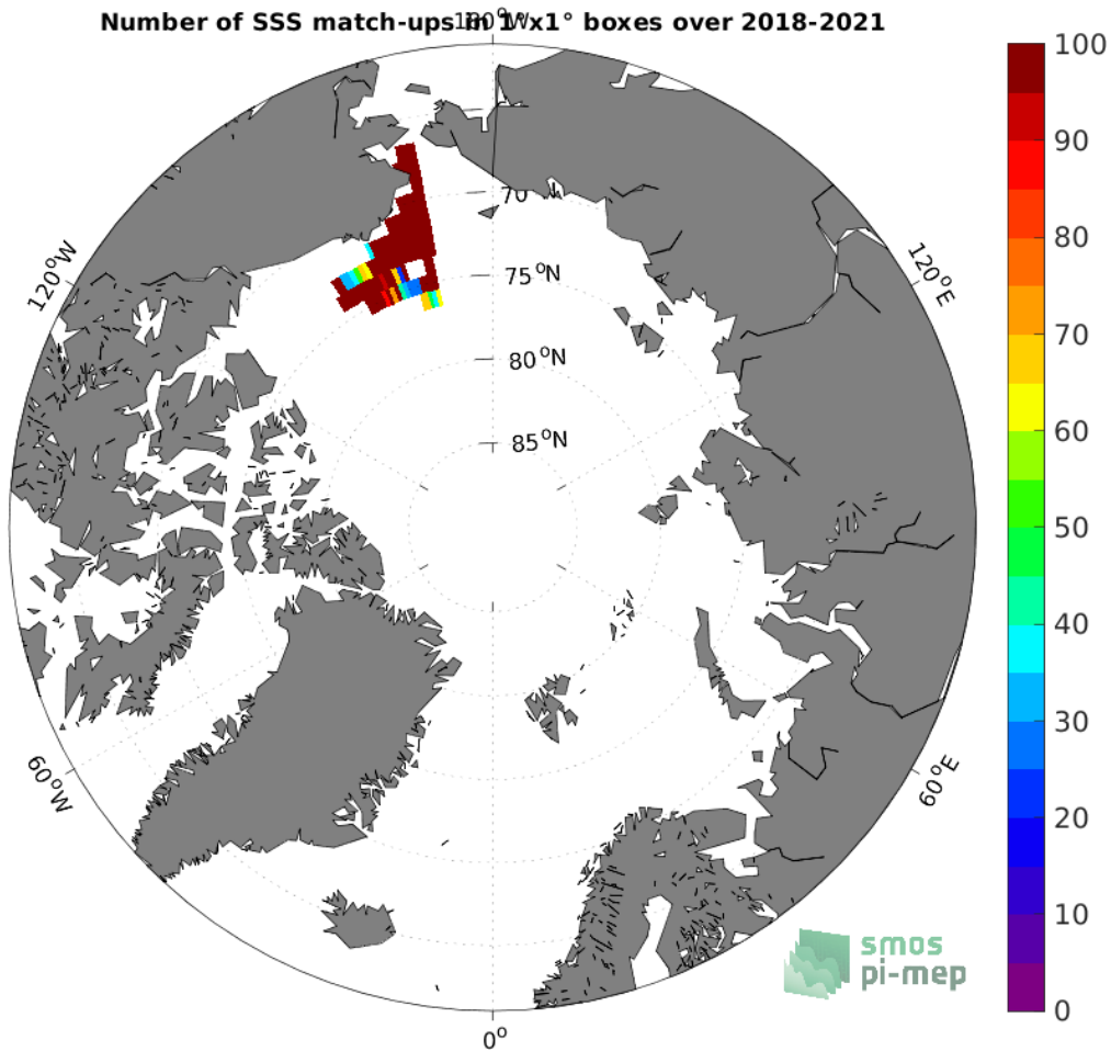
Figure 4: Number of SSS match-ups between Sairdrone SSS and the SMAP SSS L3 v5 - Monthly (RSS) SSS product for the Arctic Ocean Pi-MEP region over 1^\circ \times 1^\circ boxes and for the full satellite product period.
