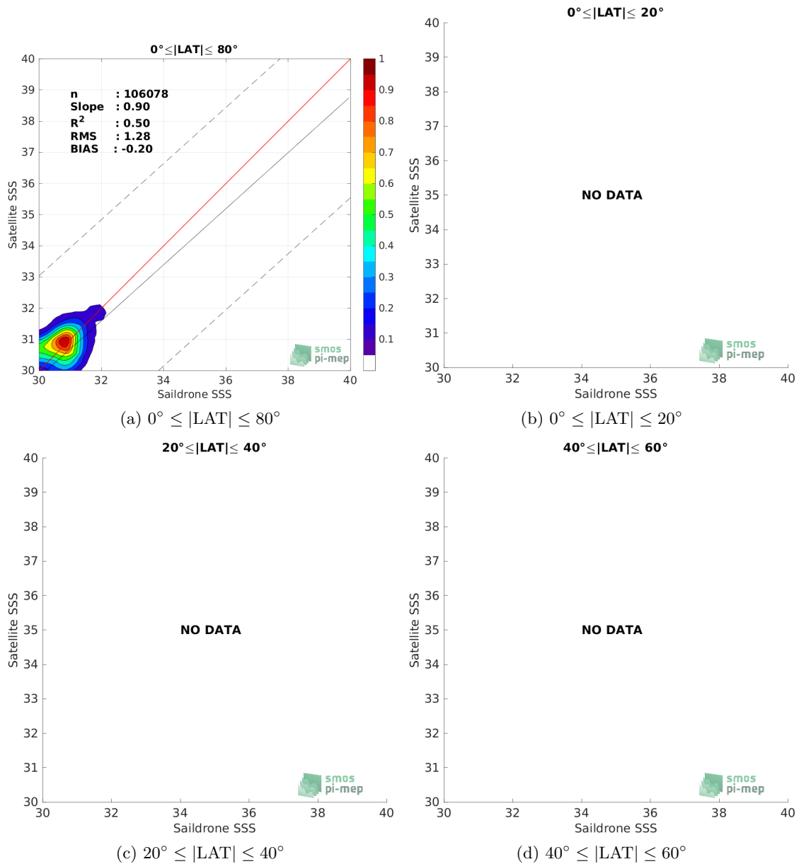
Figure 9: Contour maps of the concentration of SMAP SSS L3 v5 - Monthly (RSS) SSS (y-axis) versus Saildrone SSS (x-axis) at match-up pairs for different latitude bands. For each plot, the red line shows x=y . The black thin and dashed lines indicate a linear fit through the data cloud and the \pm 95\% confidence levels, respectively. The number match-up pairs n , the slope and R^2 coefficient of the linear fit, the root mean square (RMS) and the mean bias between satellite and in situ data are indicated for each latitude band in each plots.
