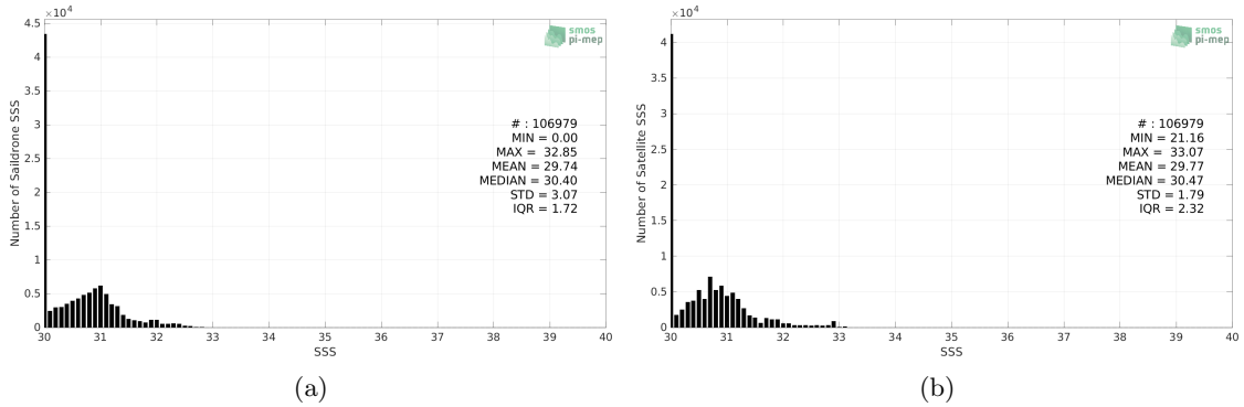
Figure 2: Histograms of SSS from Saikdrone (a) and SMAP SSS L3 v5 - Monthly (RSS) (b) considering all match-up pairs per bins of 0.1 over the Arctic Ocean Pi-MEP region and for the full satellite product period.
