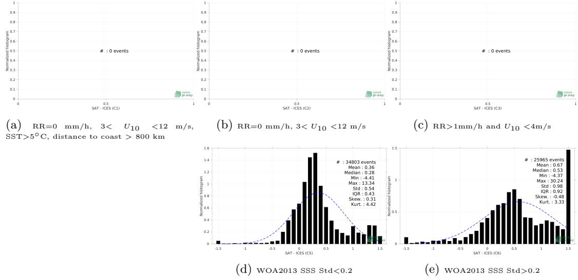
Figure 13: Normalized histogram of \Delta SSS (SMAP SSS L3 v5 - Monthly (RSS) - ICES) for 5 different subdatasets corresponding to: RR=0 mm/h, 3 < U_{10} < 12 m/s, SST > 5°C, distance to coast > 800 km (a), RR=0 mm/h, 3 < U_{10} < 12 m/s (b), RR > 1mm/h and U_{10} < 4 m/s (c), WOA2013 SSS Std < 0.2 (d), WOA2013 SSS Std > 0.2 (e).
