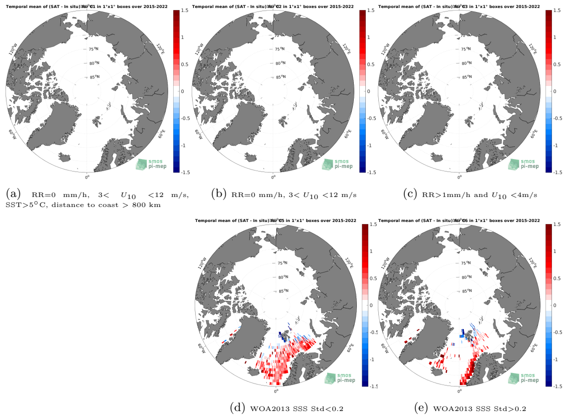
Figure 12: Temporal mean gridded over spatial boxes of size 1^{\circ}\times 1^{\circ} of \Delta\text{SSS} (SMAP SSS L3 v5 - Monthly (RSS) - ICES) for 5 different subdatasets corresponding to:RR=0 mm/h, 3 < U_{10} < 12 m/s, SST >5^{\circ}\text{C} , distance to coast > 800 km (a), RR=0 mm/h, 3 < U_{10} < 12 m/s (b), RR >1 mm/h and U_{10} < 4 m/s (c), WOA2013 SSS Std <0.2 (d), WOA2013 SSS Std >0.2 (e).
