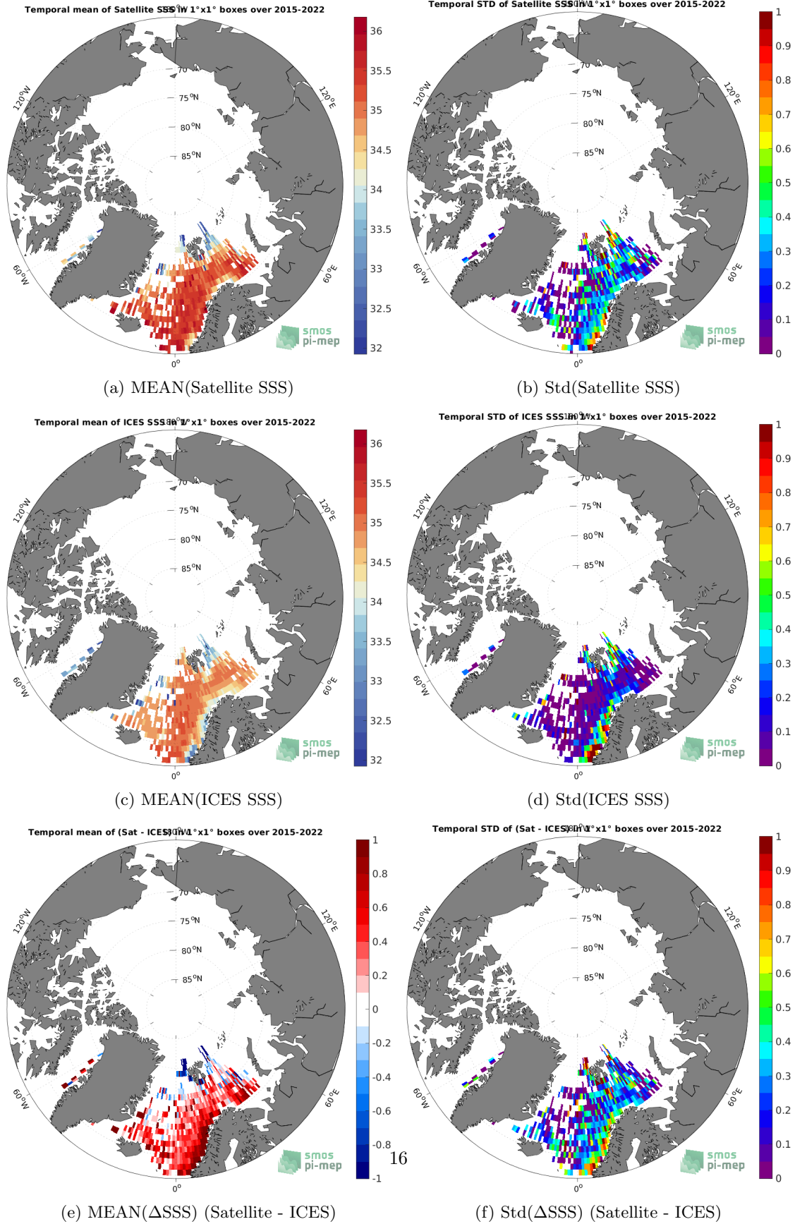
Figure 6: Temporal mean (left) and Std (right) of SSS from SMAP SSS L3 v5 - Monthly (RSS) (top), ICES (middle), and of \Delta SSS (Satellite - ICES). Only match-up pairs are used to generate these maps.
