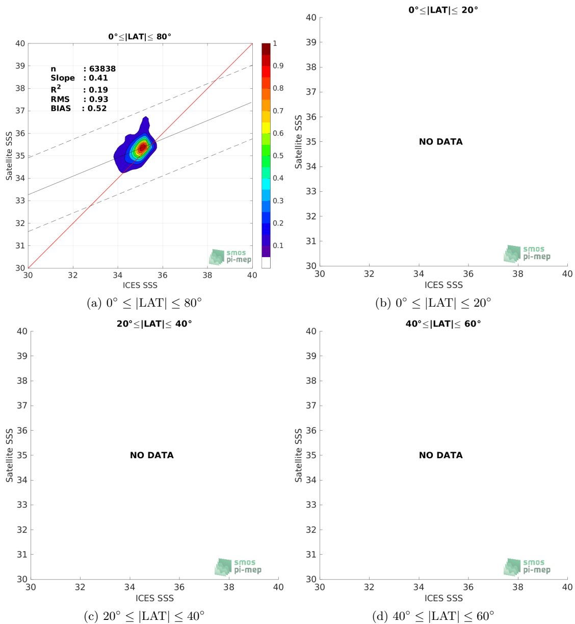
Figure 9: Contour maps of the concentration of SMAP SSS L3 v5 - Monthly (RSS) SSS (y-axis) versus ICES SSS (x-axis) at match-up pairs for different latitude bands. For each plot, the red line shows x=y . The black thin and dashed lines indicate a linear fit through the data cloud and the \pm 95\% confidence levels, respectively. The number match-up pairs n , the slope and R^2 coefficient of the linear fit, the root mean square (RMS) and the mean bias between satellite and in situ data are indicated for each latitude band in each plots.
