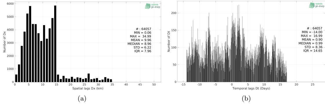
Figure 5: Histograms of the spatial (a) and temporal (b) lags between the location/time of the ICES measurement and the date of the corresponding SMAP SSS L3 v5 - Monthly (RSS) SSS pixel.
