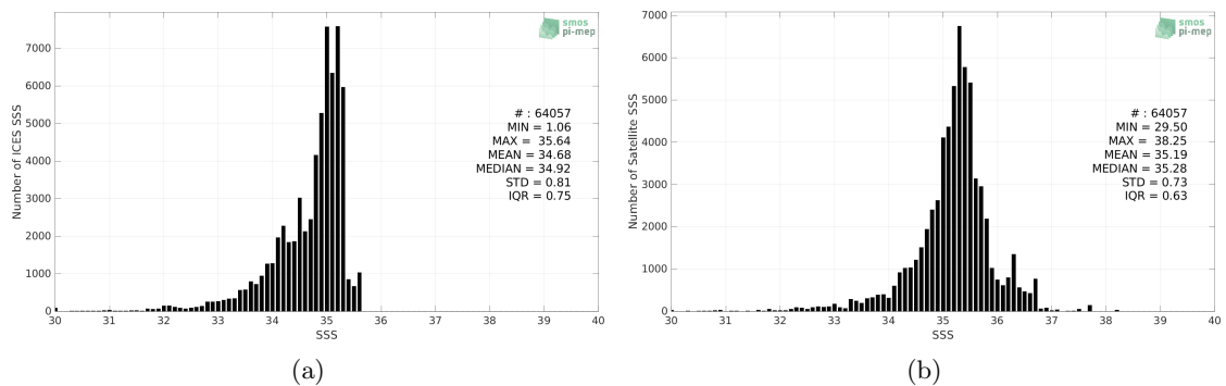
Figure 2: Histograms of SSS from ICES (a) and SMAP SSS L3 v5 - Monthly (RSS) (b) considering all match-up pairs per bins of 0.1 over the Arctic Ocean Pi-MEP region and for the full satellite product period.
