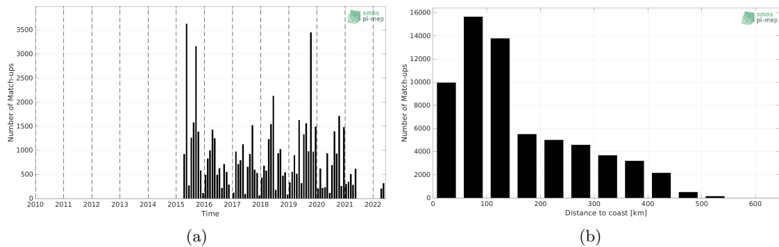
Figure 1: Number of match-ups between ICES and SMAP SSS L3 v5 - Monthly (RSS) SSS as a function of time (a) and as function of the distance to coast (b) over the Arctic Ocean Pi-MEP region and for the full satellite product period.
