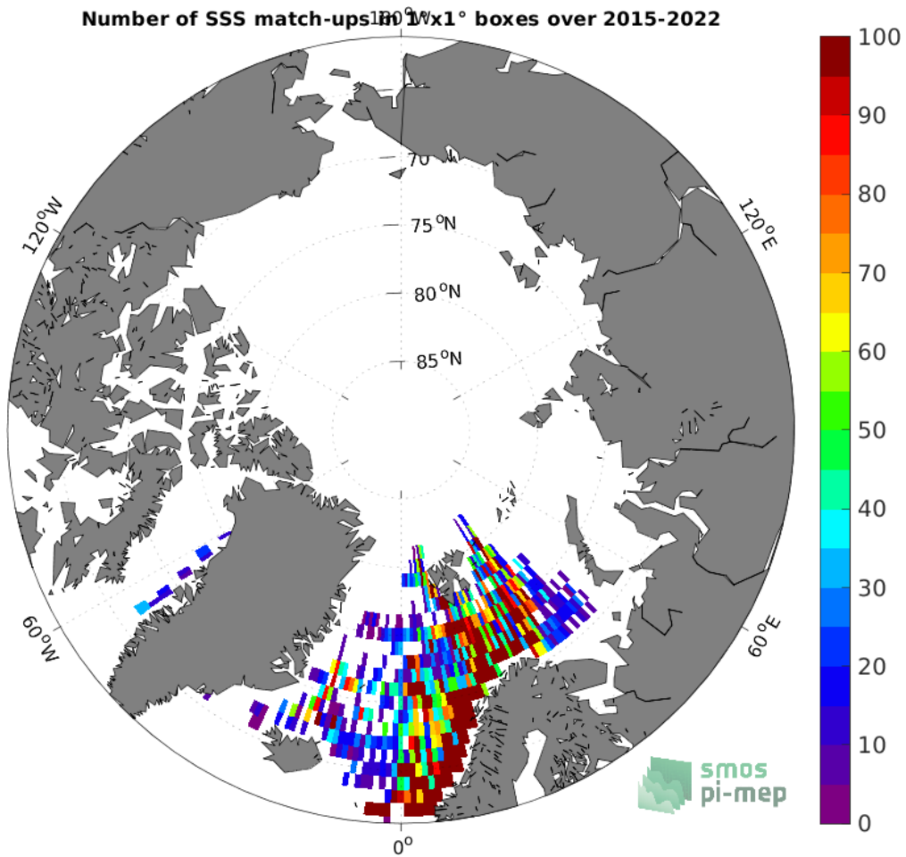
Figure 4: Number of SSS match-ups between ICES SSS and the SMAP SSS L3 v5 - Monthly (RSS) SSS product for the Arctic Ocean Pi-MEP region over 1^\circ \times 1^\circ boxes and for the full satellite product period.
