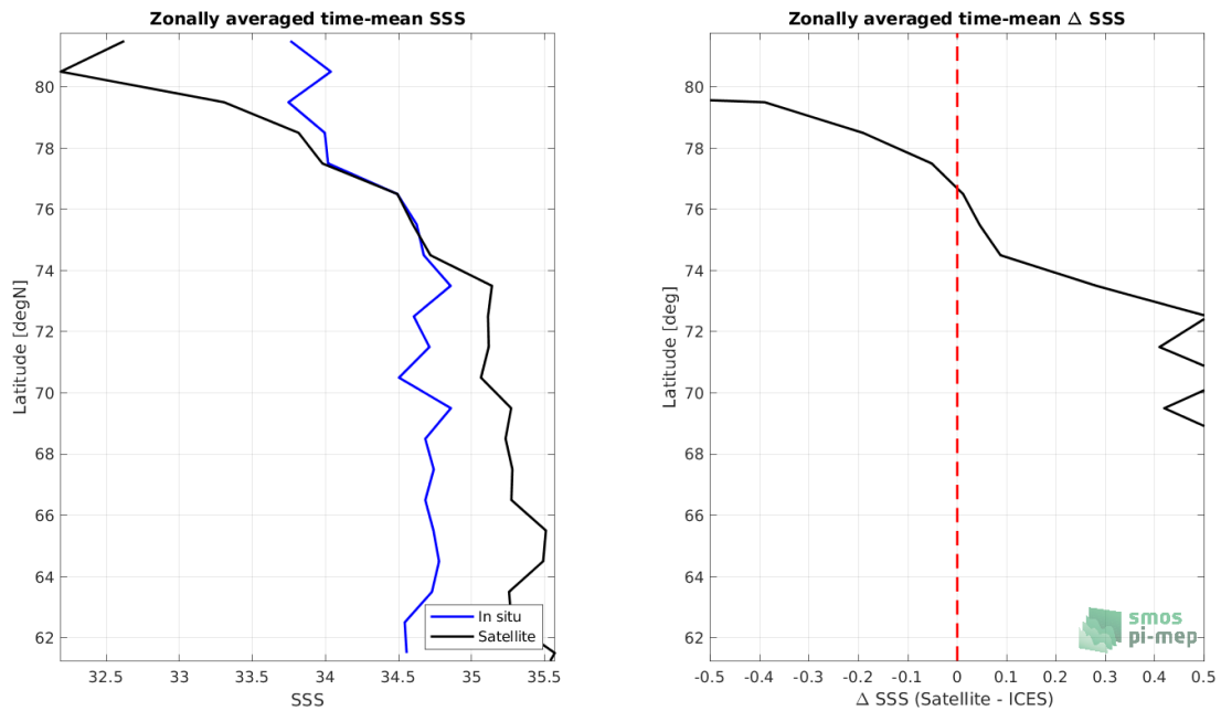
Figure 8: Left panel: Zonal mean SSS from SMAP SSS L3 v5 - Monthly (RSS) satellite product (black) and from ICES (blue). Right panel: Zonal mean of \Delta SSS (Satellite - ICES) for all the collected Pi-MEP match-up pairs estimated over the full satellite product period.
