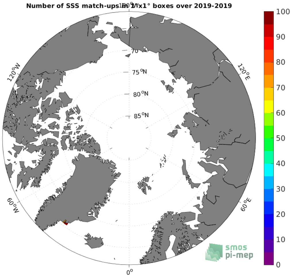
Figure 3: Number of SSS match-ups between Surface drifters SSS and the SMAP SSS L3 v5 - Monthly (RSS) SSS product for the Arctic Ocean Pi-MEP region over 1^\circ \times 1^\circ boxes and for the full satellite product period.
